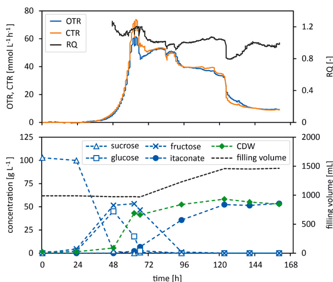
Fig. 7. Fed-batch fermentation of U. maydis MB215 \Delta\text{cyp3 } \Delta\text{MEL } \Delta\text{UA } \Delta\text{gat } \Delta\text{P}_{\text{ria1}}::\text{P}_{\text{etef}} \Delta\text{fuz7 } \text{P}_{\text{etef}}\text{mttA} grown on molasses as the sole carbon source. The cultivation was performed in a 2 L Sartorius BIOSTAT® stirred tank reactor (Sartorius AG, Göttingen, Germany) with a filling volume of 1 L at 30^\circ\text{C} . Dissolved oxygen tension was kept at > 30\% and the pH was kept constant at 6.5. RQ values are only shown for OTR values > 5 \text{ mmol L}^{-1} \text{ h}^{-1} . Samples were taken regularly and analysed via HPLC.
