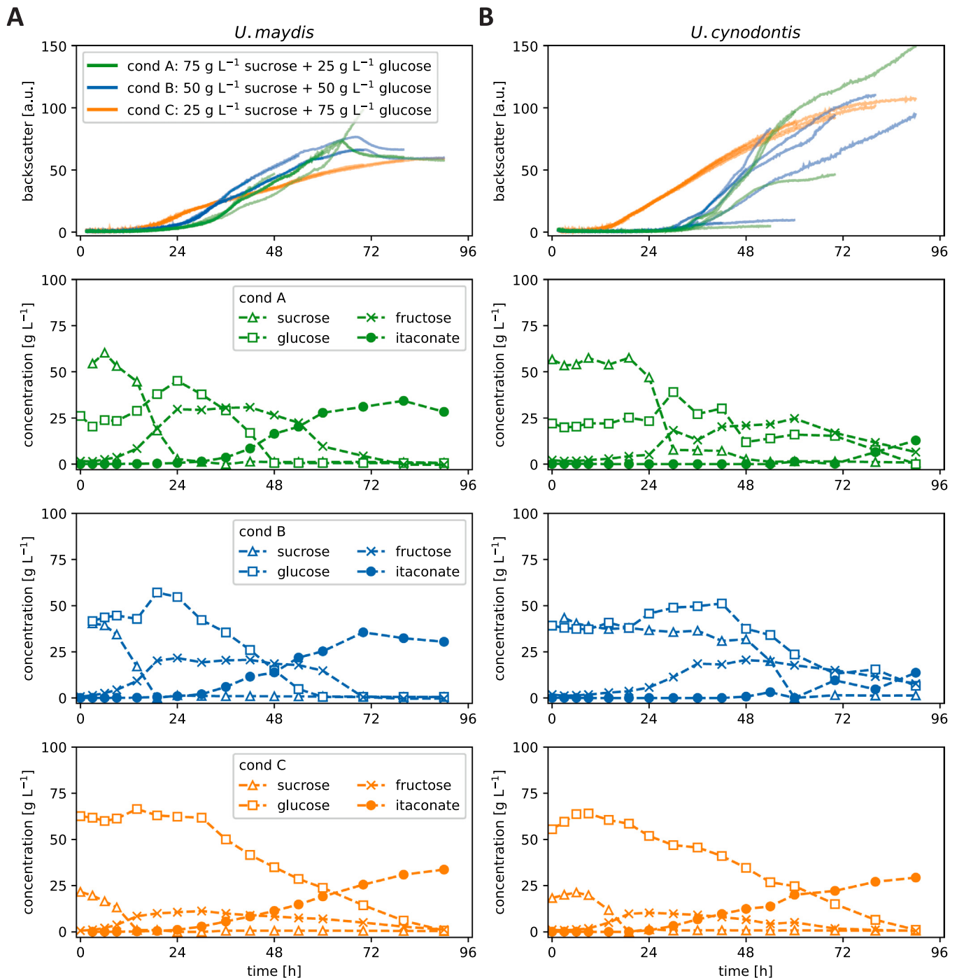
Fig. 6. Growth and itaconate production of A) U. maydis MB215 \Delta cyp3 \Delta MEL \Delta UAA \Delta dgt \Delta P_{ria1}::P_{etef} \Delta fuz7 P_{etef} mttA and B) U. cynodontis \Delta fuz7_r \Delta cyp3_r P_{etef} mttA P_{ria1} rla1 in MTM with different amounts of molasses supplemented with glucose to reach a final sugar concentration of 100 \text{ g L}^{-1} . Microscale cultures were performed in a BioLector Pro at 30^\circ \text{C} , 1400 rpm and humidity controlled at 85%. The pH and DO profiles corresponding to this experiment are depicted in Supplementary Fig. S6 .
