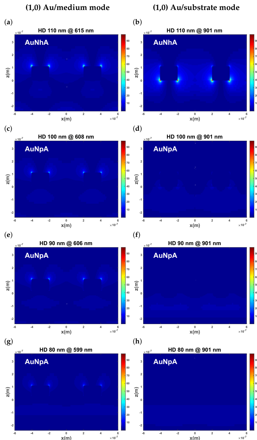
Figure 3. Cross-sectional electric field distribution of (1,0) Au/medium mode (a,c,e,g) and (1,0) Au/substrate mode (b,d,f,h) when hole depth varies from 110 nm to 80 nm.
