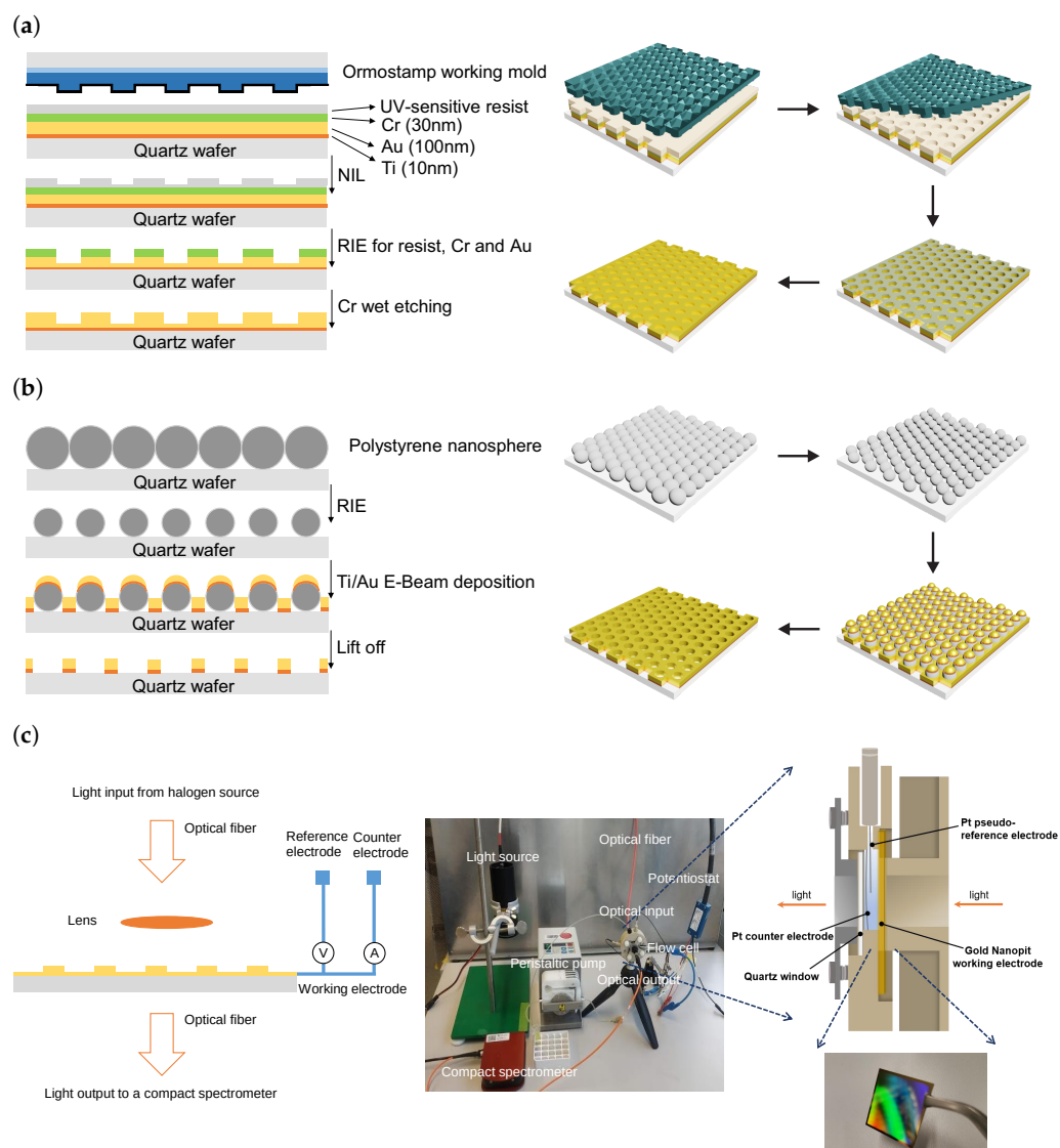
Figure 1. Schematic representation of the fabrication of AuNpA based on nanoimprint lithography (a) and full AuNhA based on nanosphere lithography (b). Schematic of the simultaneous plasmonic and electrochemical dual signal measurement set-up (c).
