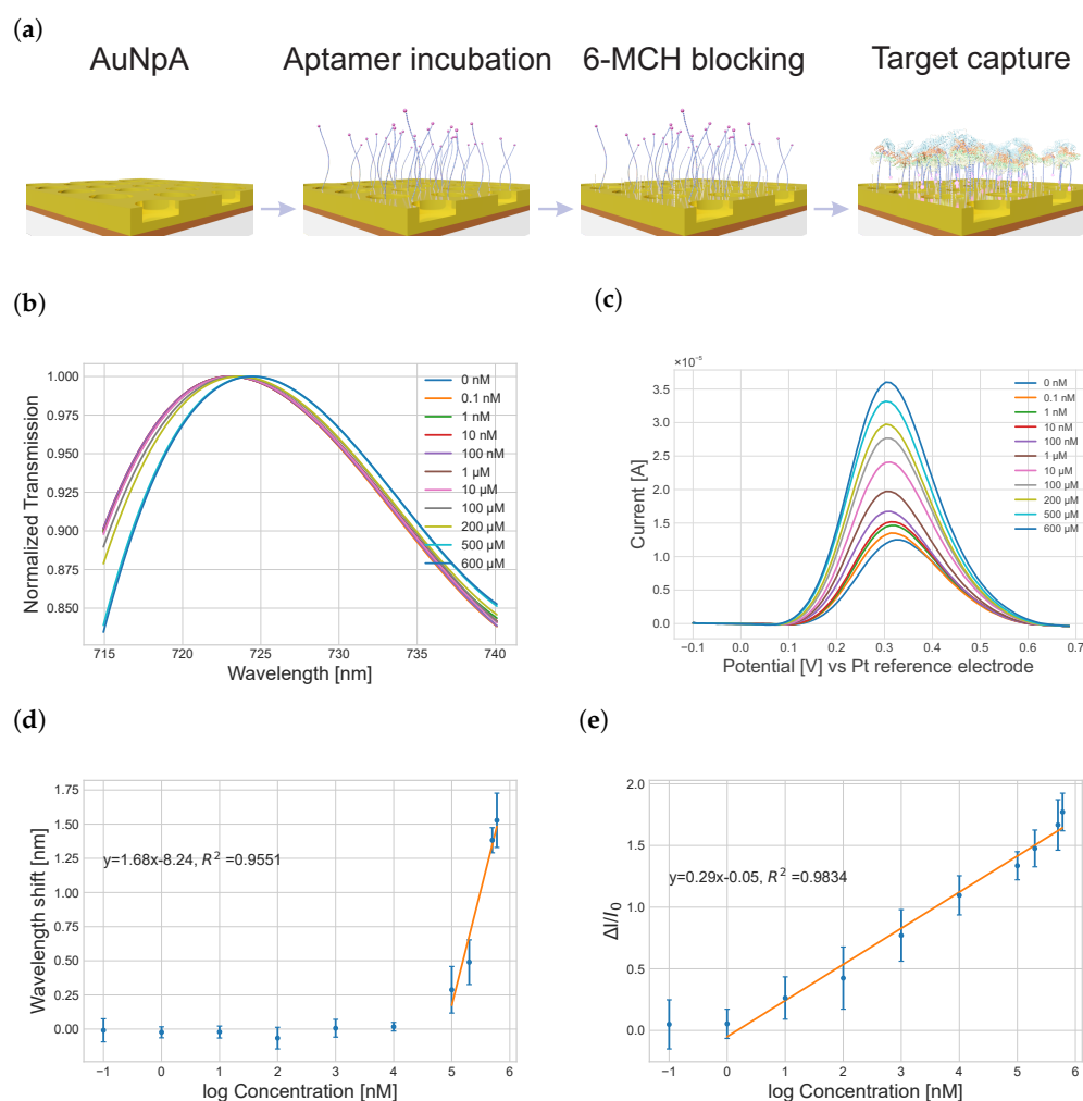
Figure 6. Schematic illustration of the working principle for HSA detection based on non-fully penetrating AuNpA (a). The binding of the HSA analyte caused a change in the aptamer conformation, through which the ferrocene redox probe approached the electrode surface and enhanced the charge transfer, fitting the normalized transmission spectrum (b) and ACV current responses (c) of our aptasensor with different HSA concentrations from 0 to 600 \mu M. The calibration curve of the sensor was found by plotting the optical shift (d) and current change (e) versus the logarithm of the HSA concentration, using 0 nM as a reference.
