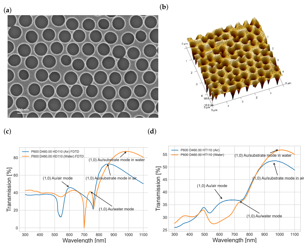
Figure 2. SEM (a) and AFM (b) images of the full AuNpA (periodicity of 600 nm) fabricated by NSL, FDTD simulation spectrum (c) and measured transmission spectrum (d) in air and water medium with P (600 nm), D (460 nm) and HD (110 nm).
