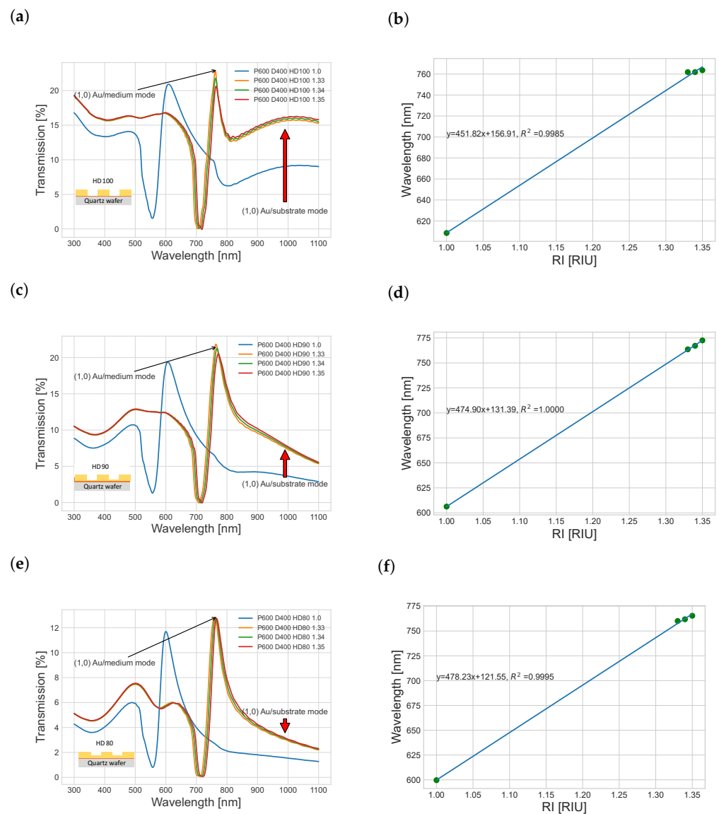
Figure 4. FDTD simulation spectrum with different hole depths from 100 nm, 90 nm and 80 nm (a,c,e, respectively) and refractive index sensitivities of the (1,0) Au/medium mode (b,d,f, respectively).
