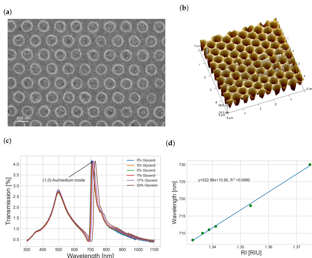
Figure 5. SEM (a) and AFM (b) images of the AuNpA fabricated by NIL, experimental refractive index sensing (c) over a wide concentration range of glycerol aqueous solutions (mass percentage) and peak wavelength regression fitting as a function over the refractive index (d).
