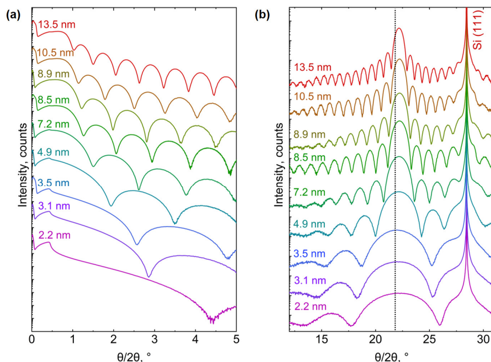
Figure 10. Thickness series of the \text{Bi}_{\text{TRIG}} (001) phase. (a) XRR-measured curves of epilayers ranging in thickness from 2.2 nm to 13.5 nm, whereas (b) depicts the corresponding diffraction patterns. The dotted black line in (b) indicates a slight shift in the out-of-plane lattice parameter due to thin-film effect.
