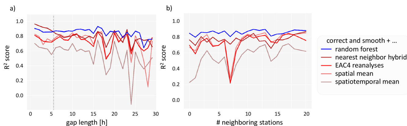
Figure 5. R^2 evaluation metric vs gap characteristics. (a) Different gap lengths up to 30 h. The dashed line marks the gap length 5 h. This is when the final imputation model changes from linear interpolation to random forest + correct and smooth. (b) Number of neighbors in a radius of 50 km around the station. This plot only contains data from isolated gaps longer than 5 h.
