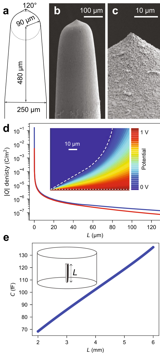
Fig. 1 Capacitance of the scanning tunneling microscope (STM) junction. a Model of the tip based on the scanning electron microscope (SEM) images ( b , c ). b , c SEM images of the tip. d Simulated surface charge density in the junction biased by the voltage of 1 V. Distribution of the potential in the junction (inset). The dashed white lines represent the outline of the tip and the sample. e Dependence of the junction capacitance C on the length L of the tip wire. Model of the STM head used for simulating C (inset).
