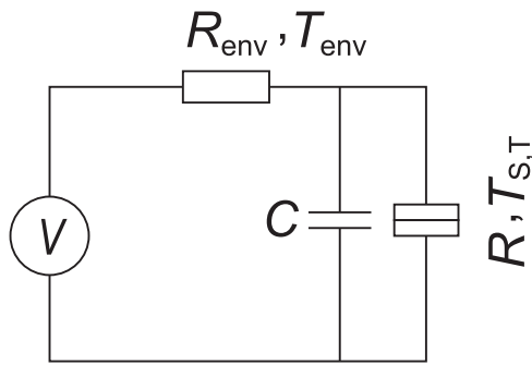
Fig. 2 Lumped element circuit model of the scanning tunneling microscope (STM) junction and its environment. The tunneling junction with tunneling resistance R and temperature T_{S,T} is shunted by the junction capacitance C and connected to a purely dissipative impedance R_{env} whose temperature is T_{env} .
