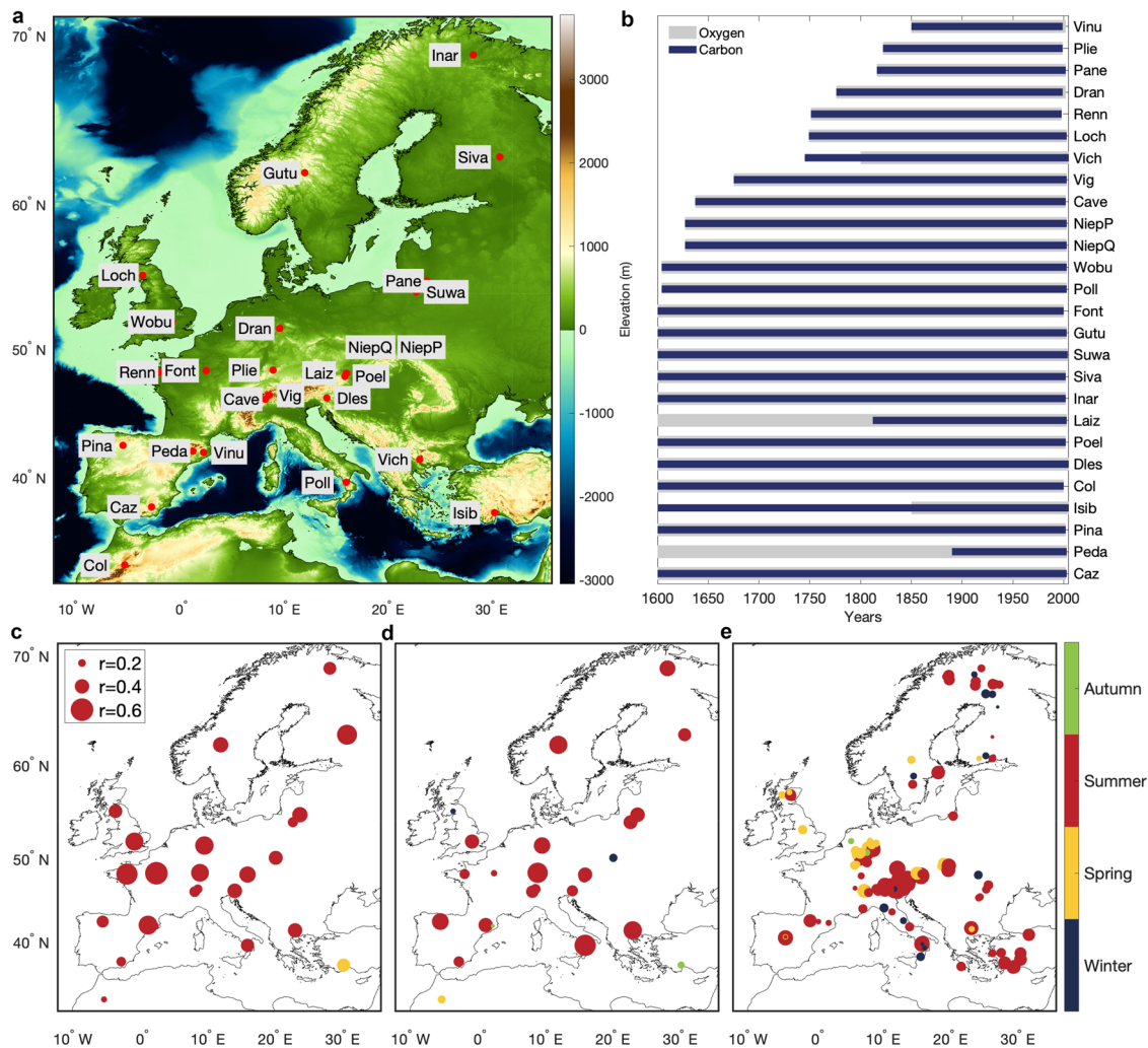
Fig. 1 Overview of the European tree-ring isotope network. a Spatial distribution of the tree sites across Europe with annually resolved isotope records of \delta^{18}\text{O} and \delta^{13}\text{C} . b Temporal distribution of \delta^{18}\text{O} and \delta^{13}\text{C} records as bars. c–e Seasonal response of carbon, oxygen and tree-ring records 62 , respectively, with SPEI-2. Shown is the highest leading seasonal correlation with SPEI. Over the 1901–1998 period the highest correlation for each site is assigned to the closest gridboxes within 60 km.
