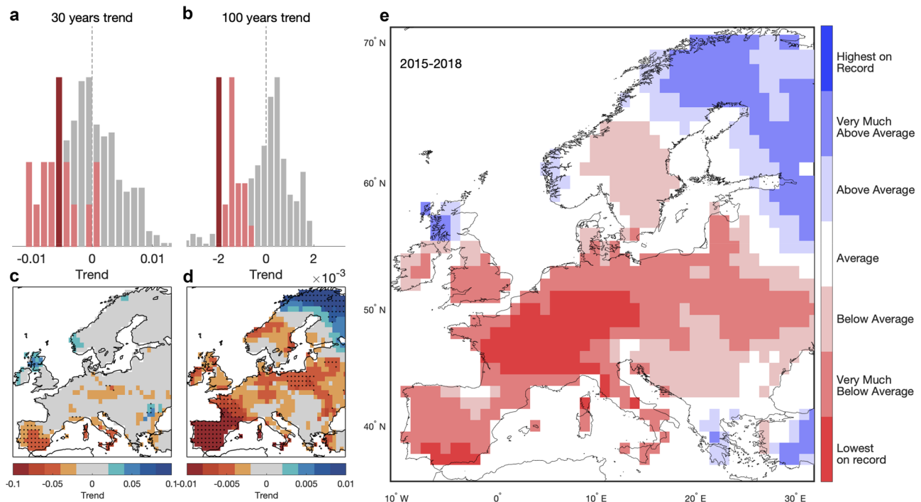
Fig. 4 Recent trends and drought. a, b Contextualising recent 30- and 100-year trends of average European SPEI (JA). Histograms show the full range of the trends (grey shaded bars) prior to 1970 for 30-year periods ( a ) and 1900 for 100-year periods ( b ). Recent periods are shown in light red, except the most recent period, which is shown in dark red. Bar heights are normalised by the maximum occurrence. c, d Recent trends of gridded SPEI of the most recent 30-year period ( c ) and 100-year period ( d ) ending in 2018. Stippling indicates statistically significant trends ( p < 0.05 ). e The recent drought period (2015–2018) is shown as deciles considering the full period (1600–2018).
