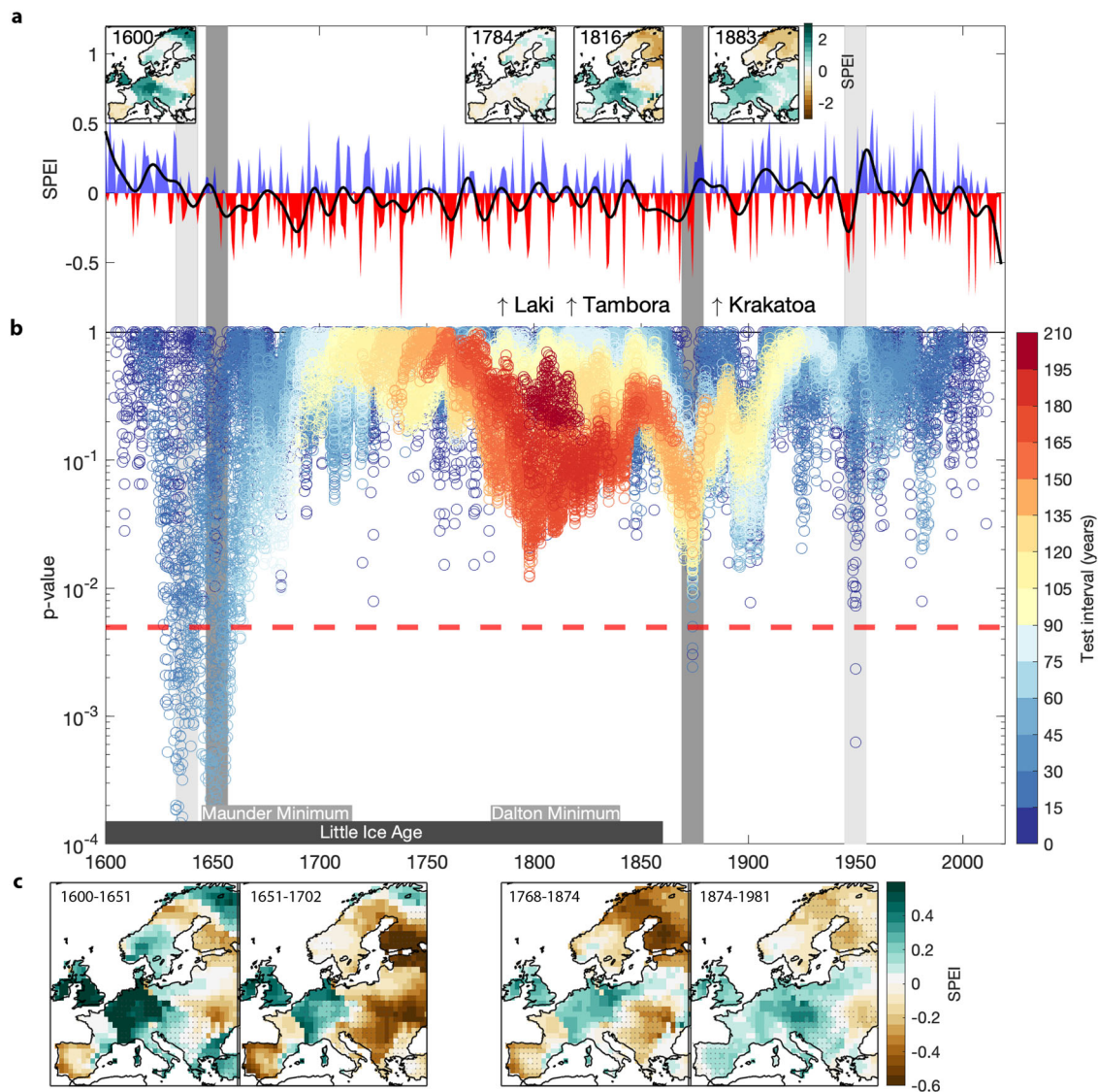
Fig. 3 Reconstructed European summer variability. a European field average of reconstructed SPEI (JA) from 1600 to 2018. A smoothed 13-year Chebyshev low-pass filter is shown as a black line. Insets show the spatial reconstructed SPEI for 1600, 1784, 1816 and 1883. b Change point analysis of European field average using the Wilcoxon rank-sum tests for sliding time intervals between 5- and 200-year time windows. The colour of a point corresponds to the tested time interval, and the year corresponds to the centre of the tested data. Significant change points are below the red horizontal line ( p < 0.01 ). The Little Ice Age ( \approx 1300 –1860 CE) and the Maunder Minimum (1645–1715) periods are highlighted. Vertical lines indicate significant long-term (dark, >30 years) and short-term (light) change points. c Average conditions before and after significant long-term change points in 1651 (left) and 1874 (right).
