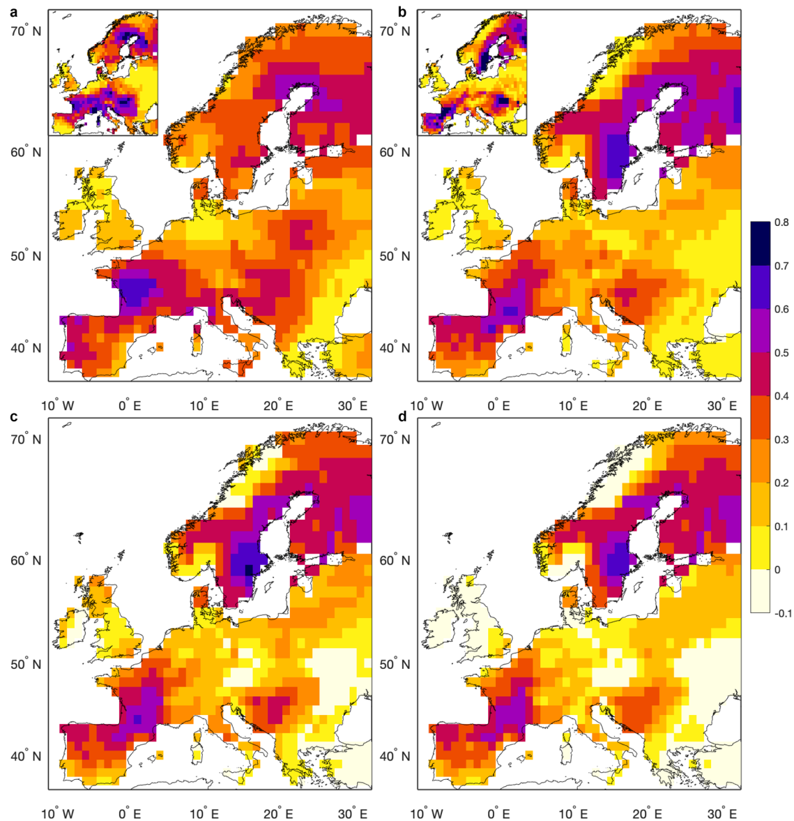
Fig. 2 Spatial reconstruction statistics. Calibration and verification statistics for the SPEI reconstruction. Explained variance ( R^2 ) of a the calibration period (median CRSQ = 0.31) and b the verification period (median VRSQ = 0.22) on interannual and decadal timescales (insets) using a 5-year moving average filter. c Reduction of error of the calibration period (median RE = 0.20). d Coefficient of efficiency of the verification period (median CE = 0.15).
