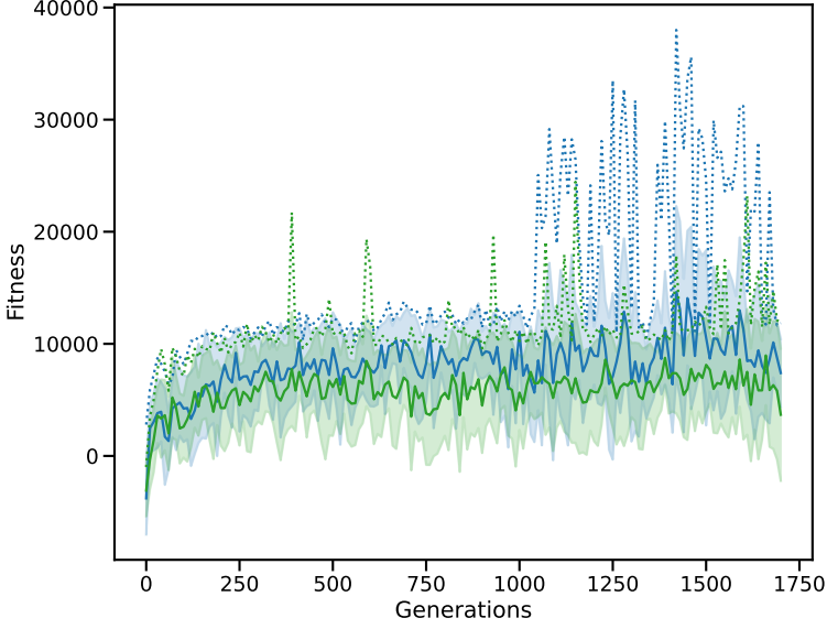
Figure 6.4: Evolution of the fitness of two different ant colony simulations over 1700 generations. In the first SNN-driven model the pheromone pathway is activated. However, the ants of the second SNN-driven model are not able to sense and deposit pheromones. The blue data series illustrates the fitness evolution of the first model. The green data series shows it for the second model. The dotted data series depicts the best individual of every generation. The blue/green solid line is the mean fitness of all individuals and the blue/green shaded area is the standard deviation.
