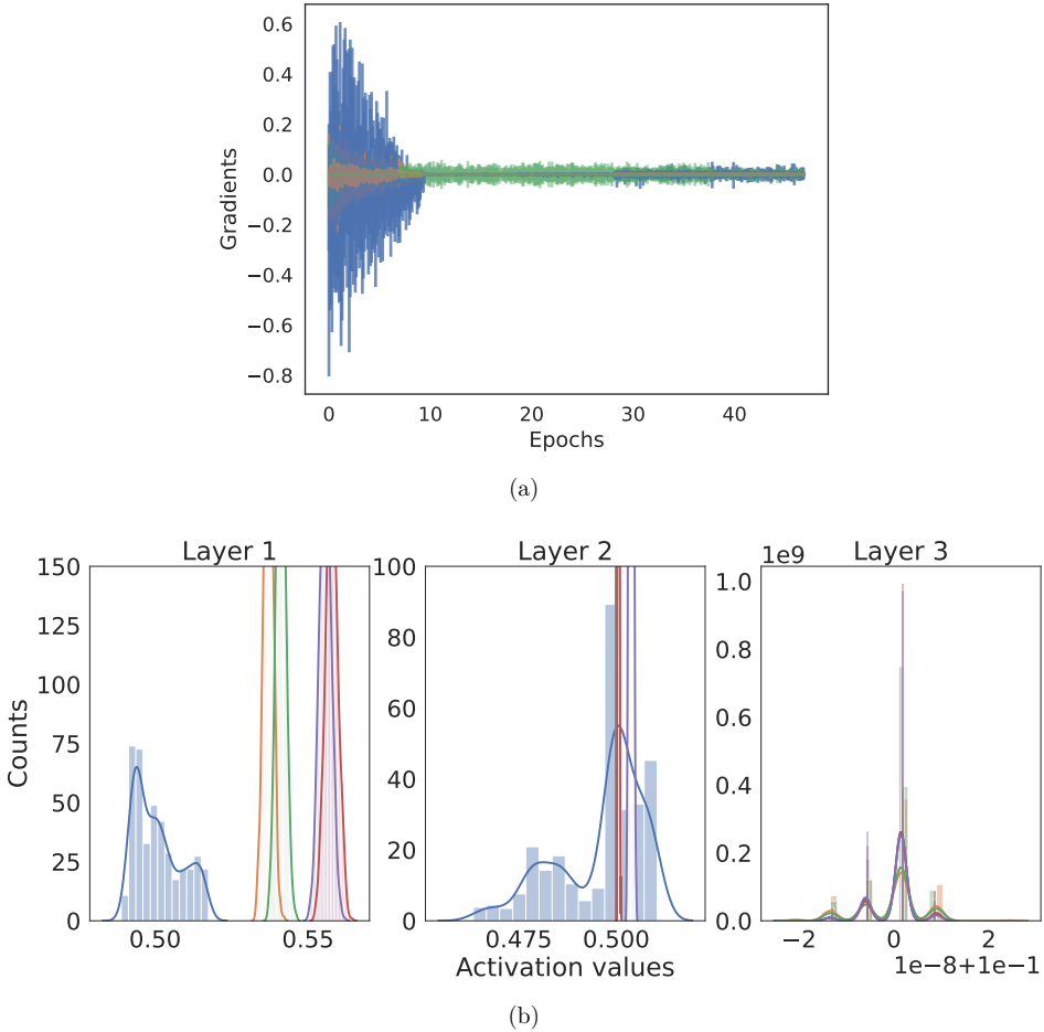
Figure 4.7: Activation values and gradient distributions over epochs using Adam as an optimizer. (a) Mean (line) and standard deviation (vertical bar) of the backpropagated gradients for all three layers for 50 epochs. (b) Mean distributions of activation values over 50 epochs for all three layers. Colors indicate the epoch. Blue: epoch 0, orange: epoch 10, green: epoch 20, violet: epoch 40.
