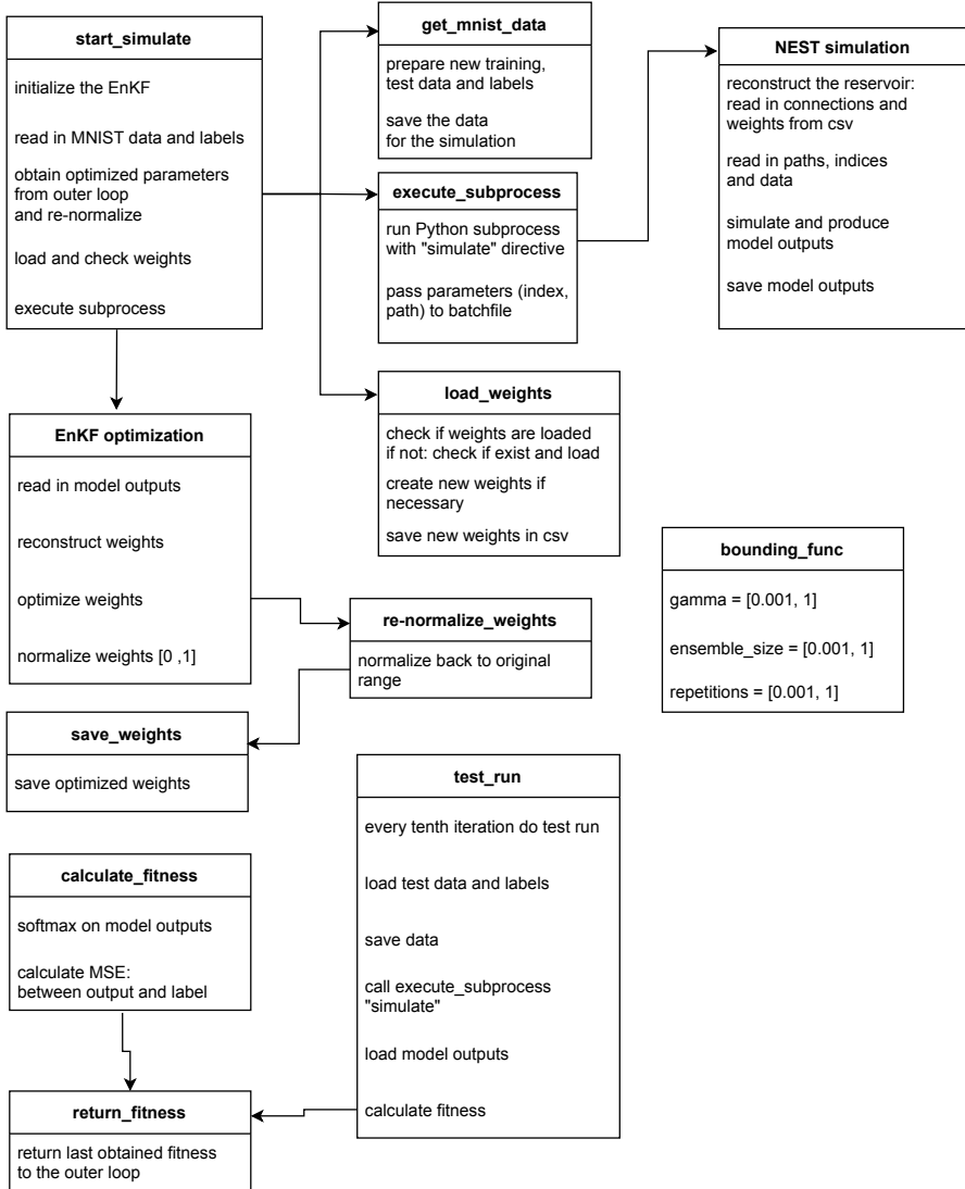
Figure 5.10: The simulation phase simulates the optimizee – the reservoir –, executes the training and test runs and returns the fitness with the hyper-parameters to the outer loop.
