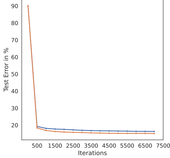
Figure 4.9: Test error on the letters dataset for different sizes of the ensemble members. The blue line depicts the error obtained with 5000 members and the orange line for 10000 members. Every 500th iteration the error is shown.
