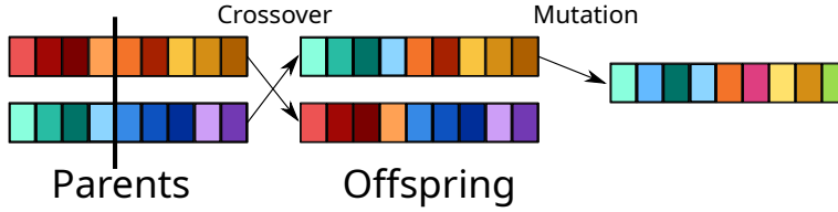
Figure 3.5: A sketch of the recombination process. The left side shows two parental individuals, the colors depict chromosomes. In the first steps crossover is applied. The second step shows the mutation of an individual. Given a probability the chromosome is changed, e.g. by adding Gaussian noise. The crossover step does not have to be applied beforehand.
