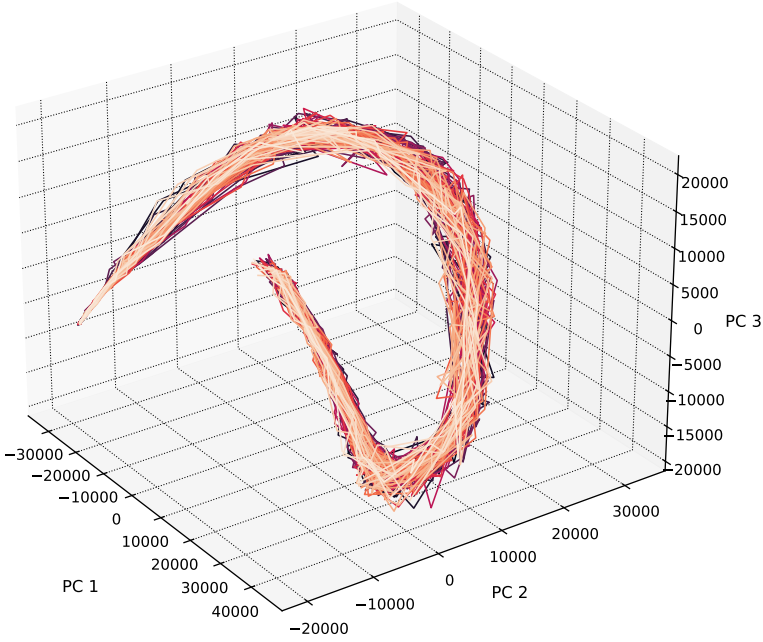
Figure 5.4: PCA of all individual weights of every 10th generation. Each color corresponds to one individual. All weights lie on the same manifold. This is due to the EnKF optimization which quickly converges the weights to an optima.
