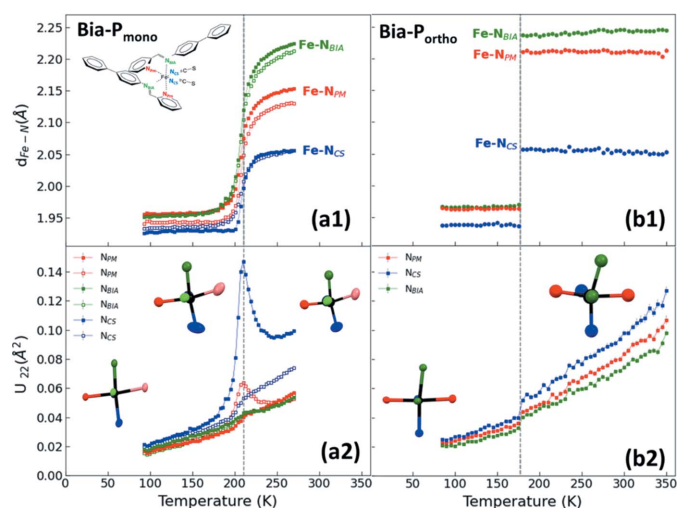
Figure 11 Temperature dependence of U_{22} (Å 2 ) for the N atoms of (a) Bia-P mono and (b) Bia-P ortho . The gray dashed line represents the transition temperature. The insets schematic diagrams in (a1), (a2) and (b2) show the molecular structure of the \text{Fe}(\text{PM-Bia})_2(\text{NCS})_2 and the corresponding ADPs of the N atoms bonded to Fe atom, respectively.
