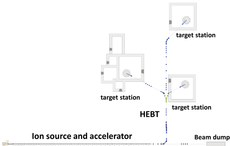
Figure III.3: Top view of the HBS High-Energy Beam Transport (HEBT) beamline to the individual target stations. The multiplexer is underground, and the beam is impinging on the targets from below.
