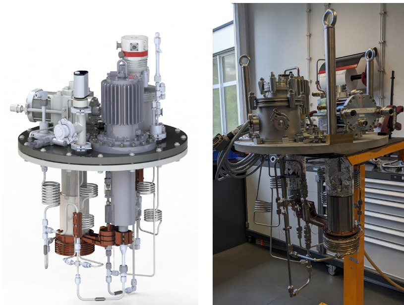
Figure III.8: Left: Design of the para-hydrogen main cryostat (courtesy of S. Eisenhut). Right: Assembly.
