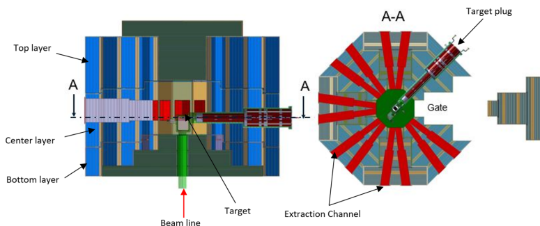
Figure III.5: Vertical cut through the target station (left side) and horizontal cut through the center of the target station with opening (right side).
