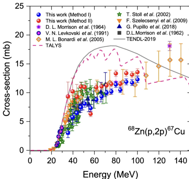
Figure A.2: Cross section for the production of Cu-67 from Zn-68 showing the scatter of the experimentally determined values and supporting the need for high proton energies around 70 MeV. [22]
