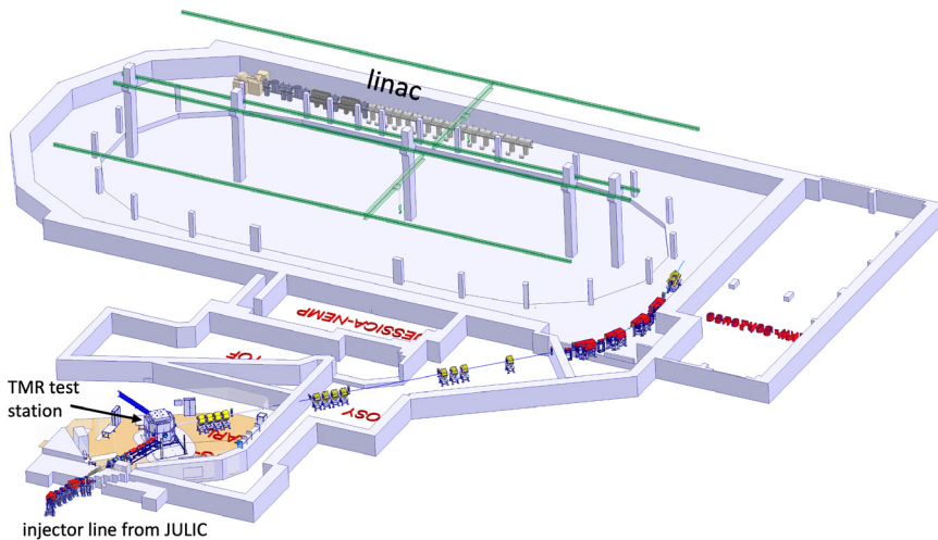
Figure A.4: Floor plan of the COSY facility. The width of the COSY hall is 37 m. The linac of the demonstrator is shown in the COSY hall, as well as the proton transfer line to the test TMR (lower left), where the current injector line of the JULIC cyclotron is still visible. The instruments can be placed around the TMR test station (in the so-called Big Karl area) and extend into the adjacent experimental areas, so that the instruments can have a maximum length of 30 m.
