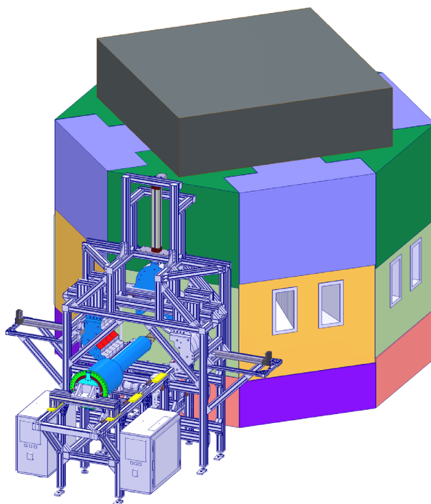
Figure III.6: Handling tool in front of HBS target station, of which the target unit is pulled out.
