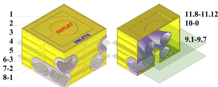
Figure III.7: Light water tank used as confinement of the liquid thermal moderator. Left: main view, Right: vertical cross section. For details see [18].
