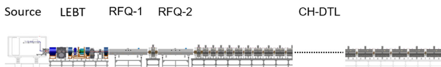
Figure III.2: Conceptual layout of the HBS linac.
