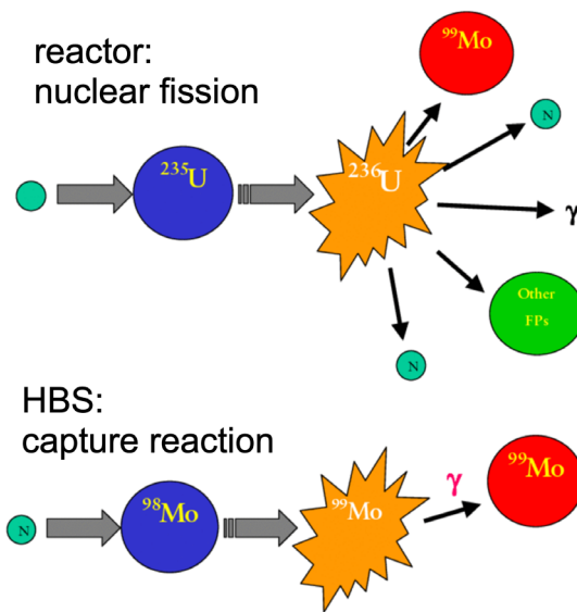
Figure A.1: Schematic of two possible routes to produce Mo-99, the parent nuclide of Tc-99m. Production in reactors by a fission reaction has a high cross section, but requires the use of nuclear fuel and leaves behind a significant amount of radioactive waste. Production by neutron capture at HBS has a lower cross section and results in less specific activity, but avoids the use of nuclear fuel material.
