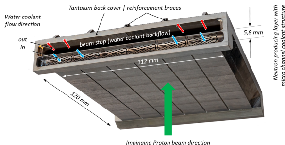
Figure III.4: Prototype of the 100 kW HBS target.
