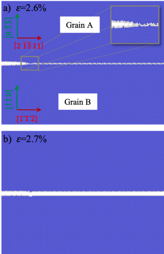
Fig. 9. Simulation setup and critical strain for fracture of the asymmetric high-angle tilt \Sigma 7\ [111]\ 38.21^\circ\ (8\ \bar{3}\ \bar{5})/(1\ \bar{1}\ 0) GB. (a) shows the orientations of grain A and B and a stable crack upon relaxation at a strain of \varepsilon = 2.6\% . The GB approximates the experimentally tested GB B7, which is shown in Fig. 5. (b) shows that the GB crack has completely cleaved the sample at \varepsilon_{cr,ini} = \varepsilon_{cr,fin} = 2.7\% . Blue atoms correspond to W atoms in a bcc lattice, while white atoms are atoms identified by CNA as belonging to a defect. The inset shows the magnified crack tip configuration. (For interpretation of the references to colour in this figure legend, the reader is referred to the web version of this article.)
