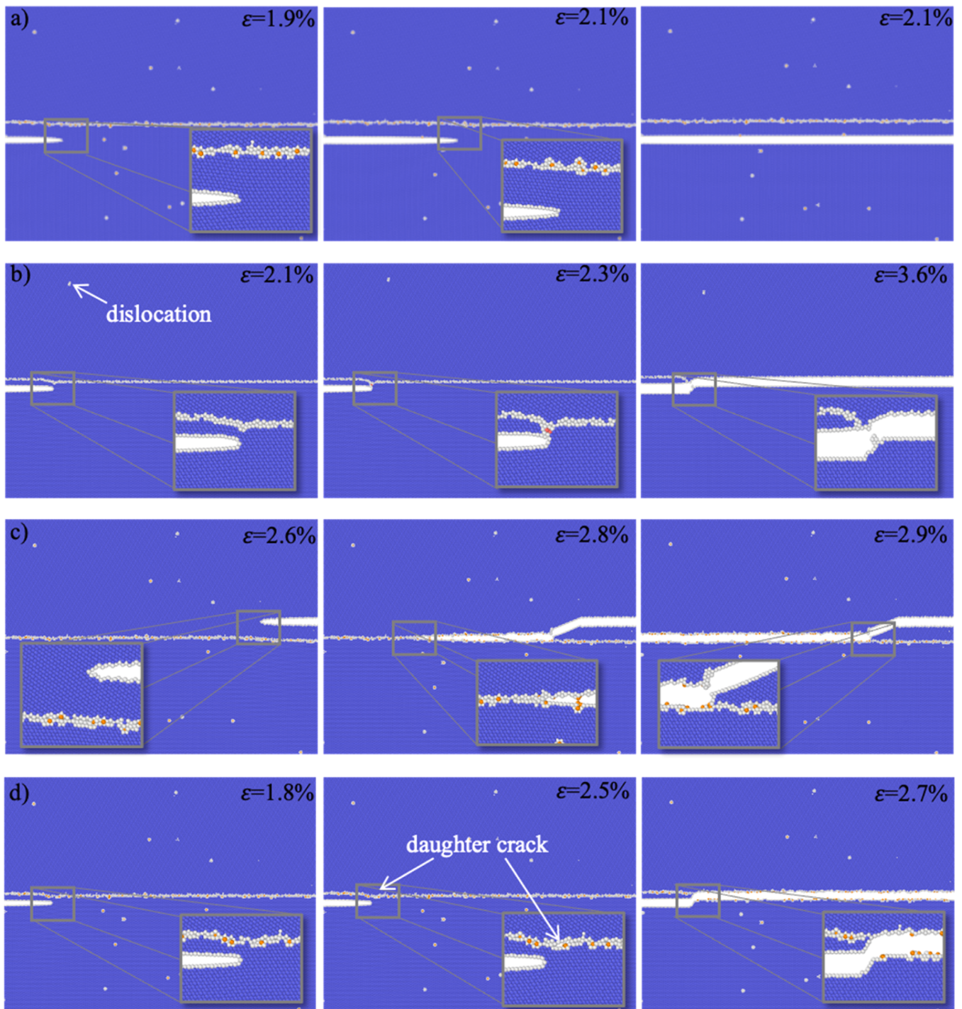
Fig. 11. Different fracture mechanisms for cracks that are not initially placed on the GB. For the colour code and the crystallographic orientations see Figs. 9 and 10. (a) Cleavage along the (1 -1 0) plane in grain B in the P-containing case. The same cleavage takes also place in pure W, but is only observed in grain B. (b) Upon initial minimisation a dislocation is emitted from the GB and the GB plastically deforms towards the crack until the crack joins the GB and propagates along the GB. This mechanism takes place only in pure W. Dislocation emission and GB plasticity also occur if the crack is further away and cannot join the GB but propagates within the grain. (c) Deviation of the crack from the initial plane onto a {110} plane towards the crack and transgranular fracture. This mechanism takes place with or without P but only in grain A (the crack can also propagate away from the GB). (d) Formation of a daughter crack in the GB, cleavage along the GB and merging with the initial crack. This mechanism has only been observed for P-containing GBs. (For interpretation of the references to colour in this figure legend, the reader is referred to the web version of this article.)
