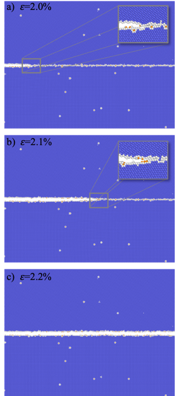
Fig. 10. Fracture of the P-segregated \Sigma 7 GB. Orientation and colour code are identical to Fig. 9, with P atoms shown in orange. (a) stable GB crack configuration; (b) relaxed, arrested crack at \varepsilon_{cr,ini} = 2.1\% ; (c) fully cleaved sample at \varepsilon_{cr,fin} = 2.2\% . (For interpretation of the references to colour in this figure legend, the reader is referred to the web version of this article.)
