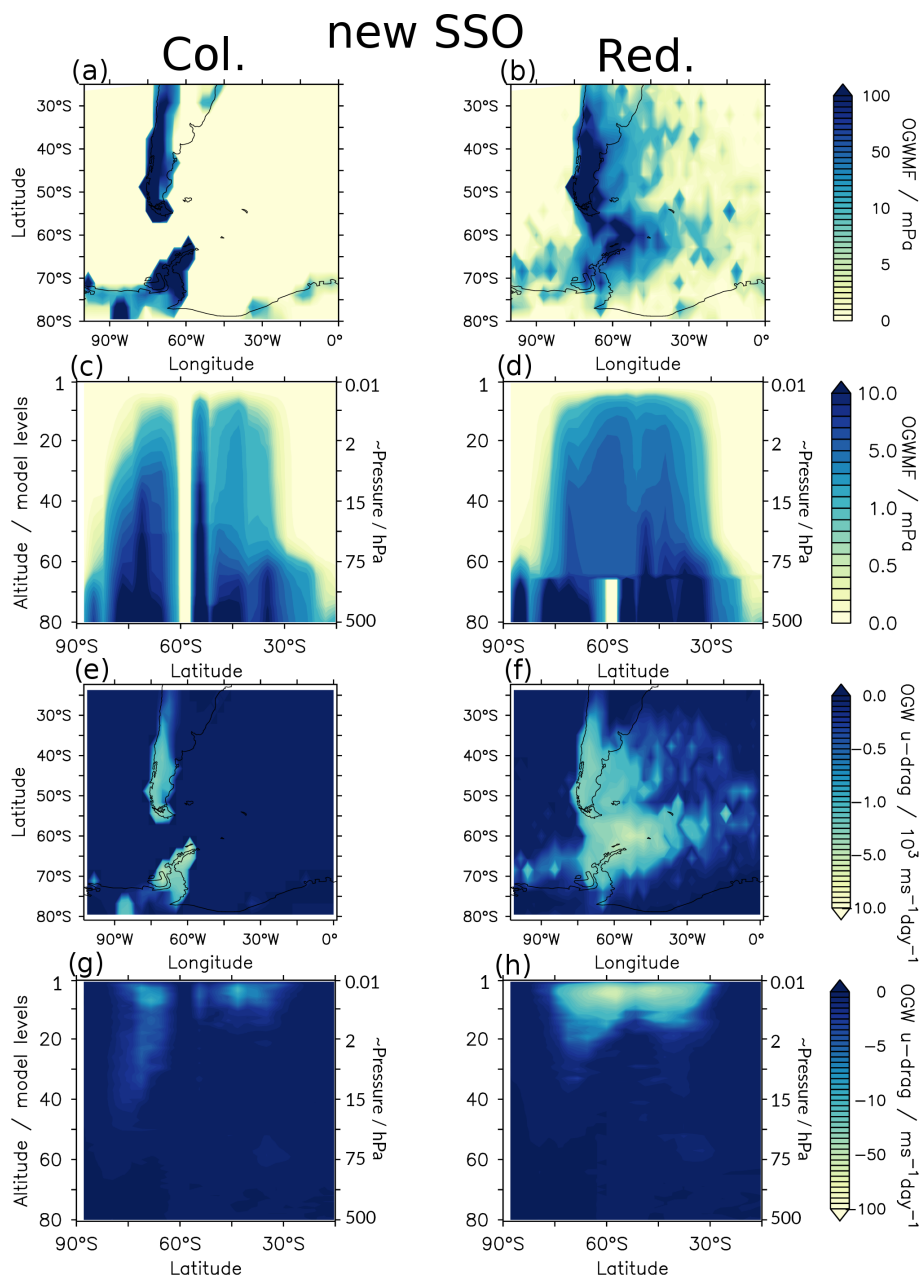
Figure 9. As Fig. 8 but with the updated SSO.
