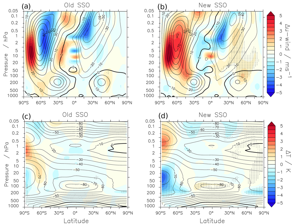
Figure 11. Zonal-mean zonal wind ( a and b ) and temperature ( c and d ) differences in JJA between the simulations with and without OGW redistribution using the old ( a and c ) and the new ( b and d ) SSO. The contour lines show the climatologies without OGW redistribution in metres per second ( \text{m s}^{-1} ) and degrees Celsius ( ^{\circ}\text{C} ), respectively. Dotted regions depict where the differences are statistically significant at the 95 % level.
