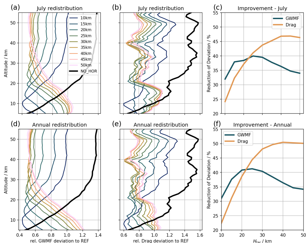
Figure 3. Comparison of MWM simulations with GW redistribution (with varying H_{\text{tar}} , coloured lines) and vertical-only propagating MWM simulations (NO_HOR, black lines) to a simulation including horizontal propagation (REF) for (a, d) GWMF and (b, e) GW drag. To show the effect of the target height, H_{\text{tar}} , the GW redistribution is performed at the lowermost level in these four panels, leading to profile differences at all altitudes. The horizontal axis shows the relative deviation from REF at the corresponding altitude in the monthly and global mean. Panels (c) and (f) show the maximum improvement (reduction of deviation from REF) for different H_{\text{tar}} with optimal redistribution height (i.e. the redistribution takes place at the cross-over of the black and the respective coloured curve). This is proportional to the area between the black and the coloured curves in panels (a) and (b) (only to the left of the black curve). The redistribution maps were generated from simulations of July 2006 in panels (a)–(c) and from simulations of the entire year of 2006 in panels (d)–(f) and applied to simulations of July 2006 in both cases.
