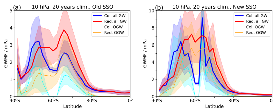
Figure 10. Climatological 20-year JJA zonal-mean total GWMF and OGWMF at 10 hPa for the simulations with (a) the old SSO and (b) the new SSO. Col. stands for columnar and Red. for redistribution activated. The shading denotes the variability by means of 1\sigma of the GWMF.
