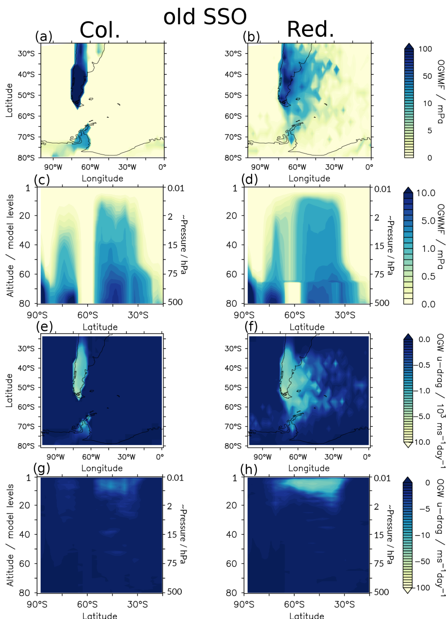
Figure 8. Comparison of orographic GWMF and GW drag between the standard columnar approach (left) and using the GW redistribution (right) with the standard SSO: (a–d) GWMF at model level 65 (level of redistribution) (a, b) and as a zonal mean (c, d). (e–h) GW drag vertically summed up (e, f) and as a zonal mean (g, h). Note that panels (c), (d), (g) and (h) are depicted in hybrid sigma-pressure model levels to clearly visualise the redistribution level. For reference, the second vertical axis denotes approximated pressure levels, and additionally the distribution of hybrid sigma-pressure model levels of the EMAC L90MA setup with pressure altitude is shown in the Supplement.
