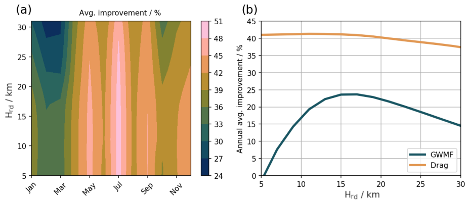
Figure 4. (a) Improvement of GW drag across the year 2006 as monthly means for varying H_{rd} . The improvement is the reduction in deviation from REF through GW redistribution. (b) Annual mean improvement for GWMF (blue) and GW drag (orange) with varying H_{rd} .
