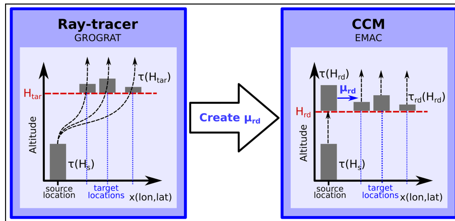
Figure 1. Schematic of the redistribution approach with example momentum propagation paths. The momentum transport target locations are estimated at a fixed target height, H_{\text{tar}} , and weighted by the GWMF of the respective GWs. This pattern of horizontal transport (the redistribution map \mu_{\text{rd}} ) is applied in EMAC at the redistribution height, H_{\text{rd}} , which should be lower than H_{\text{tar}} . Energy conservation is preserved by only redistributing the GWMF that EMAC computes in the source column just below H_{\text{rd}} , i.e. by \tau(H_{\text{rd}}) = \sum_x \tau_{\text{rd}}(H_{\text{rd}}) .
