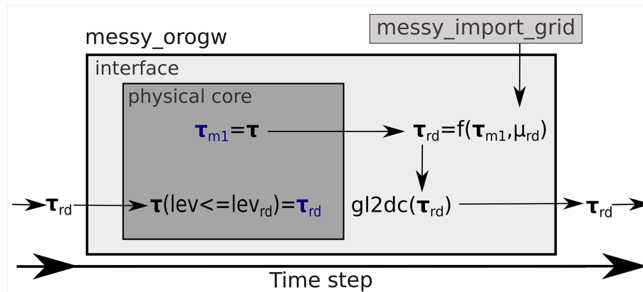
Figure 5. Schematic of the GW redistribution implementation in the EMAC submodel OROGW. The physical core denotes the parameterisation itself, and the interface is the connection to the other model parts. Here, gl2dc stands for global to decomposition, \mu_{rd} for the redistribution (rd) function, m/ for the minus 1 (with respect to the time step) value, lev for model level and \tau for the GW flux. See main text for more explanations and the Supplement for EMAC/MESSy-specific implementation details.
