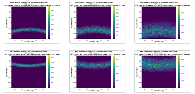
Fig. 8. McStas simulation results of scattering of fullerene C60 samples on two detection panels positioned as indicated in Fig. 7, using neutrons with a wavelength \lambda = 5 \text{ \AA} with a resolution of \Delta\lambda/\lambda = 5\% (left panels), 10% (middle panels) and 20% (right panels).
