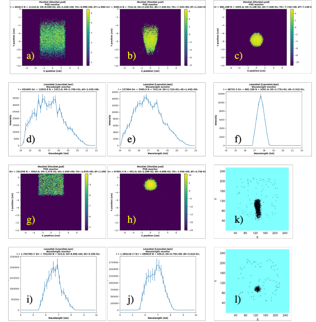
Fig. 4. Results of McStas simulations (taking into account the gravity) and neutron measurements of the direct beam profile on the detector placed at 17.5 m for 4-lens system in beam. Panels a) and g) show the direct beam on the detector when lenses are out of beam for \lambda = 18 Å and \lambda = 7 Å, respectively, for a \Delta\lambda/\lambda = 20\% in both cases, while panels e) and g) present the wavelength distribution in both situations. Panels b) and c) show the direct beam on the detector when lenses are in beam, for a \Delta\lambda/\lambda = 20\% and \Delta\lambda/\lambda = 5\% , respectively, while panels e) and f) present the corresponding wavelength distribution. Panels h) and j) present the same data for \lambda = 7 Å with a \Delta\lambda/\lambda = 20\% . Panels k) and l) show measured direct beam profile on the HRD for \lambda = 18 Å, with \Delta\lambda/\lambda = 20\% and \Delta\lambda/\lambda = 5\% (using TOF mode).
