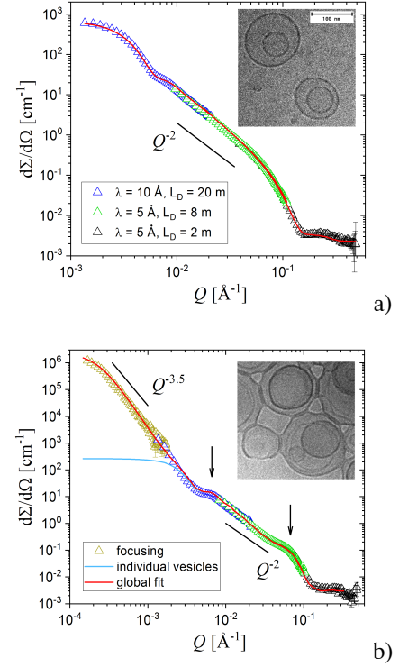
Fig. 5. SANS data of lipid (a) and lipid + MBP (b) solutions recorded at KWS-2 in pinhole mode (a) and in combined pinhole and focusing modes (b). The red curves show the model fit of the experimental data according to the vesicle form factor (a) and the unified model of the docked vesicles, as the product of vesicle form factor and docking structure factor, and the large-scale aggregates (b). The light blue curve in panel (b) shows the scattering contribution of the docked vesicles. The insets show cryo-TEM images of the same samples, where the scale bar valid for both images is 100 nm.
