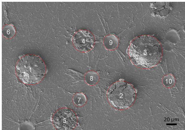
Fig. 8 Single-splat morphologies sprayed with the 4L2 nozzle on mirror-polished stainless-steel substrates at 350-mm spray distance: softened No. 1–3, splat Ø 56–66 \mu\text{m} ; semi-molten No. 4 and 5, splat Ø 43–48 \mu\text{m} ; fully molten No. 6–10, splat Ø 26–31 \mu\text{m} ; (secondary electron image)
