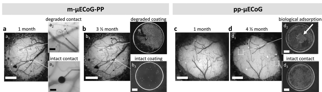
Fig. 6 Chronic stability of \mu ECoGs. (a) Widefield vessel image after one month (a 1 ) and three-and-a-half-month post-implantation (b 1 ). Red circles point out those electrical contacts that are degraded. Scale bar = 0.5 mm. Zoomed in degraded (a 2 ) and intact contact (a 3 ). Scale bar = 50 \mu m. The degradation signs exhibited by m- \mu ECoG-PP are stagnating after one month-implantation. (b 2 ) Scanning electron microscopy (SEM) images exposing exemplary electrical contacts of a m- \mu ECoG-PP with a degraded (b 2 ) and intact (b 3 ) PEDOT:PSS coating after three-and-a-half month post-implantation. Widefield vessel image of pp- \mu ECoG one month (c) and four-and-a-half-month (d 1 ) post-implantation. (d 2 ) and (d 3 ) SEM images of an biological adsorption on an intact electrode contact and an intact contact without residues of a pp- \mu ECoG four and a half months post-implantation. Scale bar of SEM pictures = 10 \mu m.
