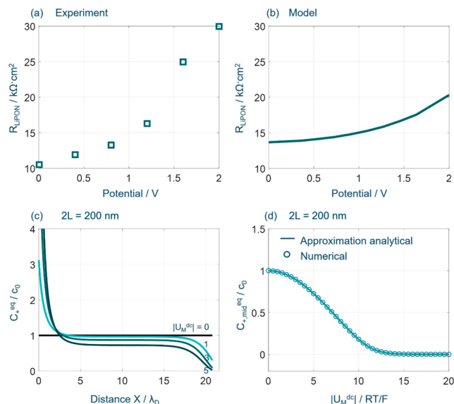
Figure 4. EIS of ion transport in the double-blocking closed cells. (a, b) Comparison between model and experimental results of the EIS response at different potentials. Experimental data were reported by Katayama et al. in Ni/LiPON/Li. 54 The model-based result is calculated using c_0 = 0.25 M, D_+ = 2 \times 10^{-12} m 2 s -1 , \epsilon_s = \epsilon_{\text{LiPON}} = 16.6\epsilon_0 , and 2L = 760 nm. (c) shows the steady-state distribution of cation concentration at different applied voltages, and (d) the steady-state cation concentration at the middle plane as a function of applied voltage. Analytical and numerical results are displayed as solid and dashed lines, respectively. Model parameters are c_0 = 1 \times 10^{-3} mol L -1 , D_{\pm} = 1 \times 10^{-11} m 2 s -1 , 2L = 200 nm, and \delta_{\text{HP}} = 0 nm.
