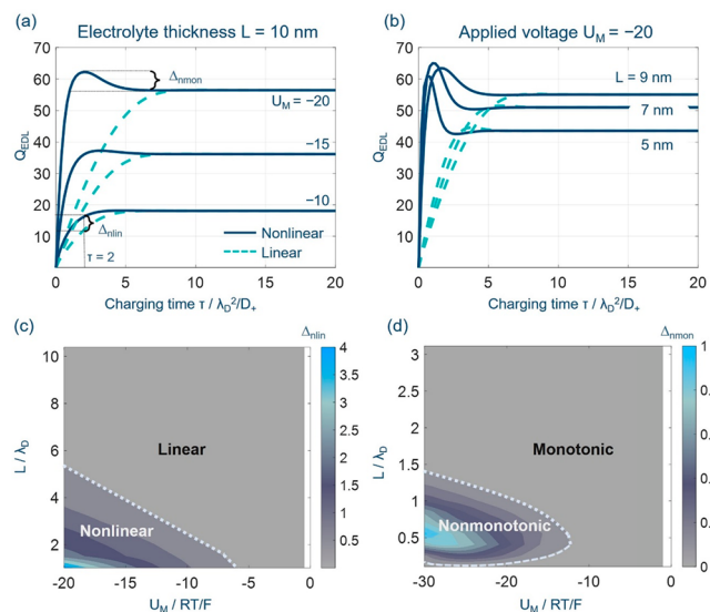
Figure 2. Charging dynamics of nanoconfined electrolytes in terms of the total diffuse charge Q_{\text{EDL}}(\tau) for the nonlinear (solid line) and linear PNP theory (dashed line) at (a) different applied voltages and (b) electrolyte thicknesses for the single-blocking open cells. (c) Regime of nonlinearity of the PNP theory. (d) Regime of nonmonotonic EDL charging dynamics. Model parameters are c_0 = 1 \times 10^{-3} \text{ mol L}^{-1} , D_{\pm} = 1 \times 10^{-11} \text{ m}^2 \text{ s}^{-1} , and \delta_{\text{HP}} = 0.3 \text{ nm} , and the corresponding reference values are \lambda_D \approx 9.63 \text{ nm} , t_{\text{ref}} = \lambda_D^2 / D_+ = 9.27 \times 10^{-7} \text{ s} , and U_{\text{ref}} = RT/F = 25 \text{ mV} .
