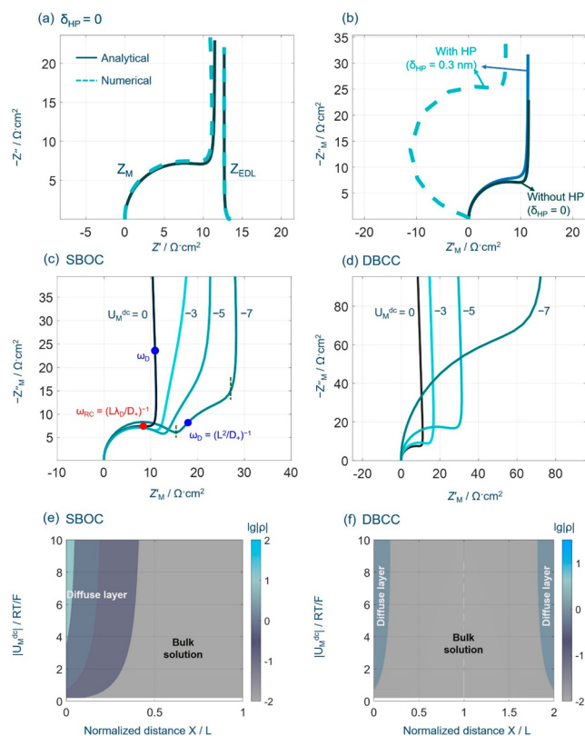
Figure 3. EIS of ion transport in the single-blocking open cells. (a) Comparison between the EIS calculated from the total diffuse charge, denoted as Z_{EDL} , and that from the electrode surface charge, Z_M , at the potential of zero charge, U_M^{dc} = 0 and \delta_{HP} = 0 nm. Analytical and numerical results are displayed as solid and dashed lines, respectively. (b) Influence of the Helmholtz plane (HP) on analytical (solid lines) and numerical (dashed lines) solutions of Z_M , Z_M at different electrode potentials U_M^{dc} for the (c) SBOC and (d) the DBCC at L = 100 nm and \delta_{HP} = 0 nm. (e, f) Distribution of the net charge density at different U_M^{dc} s for the SBOC and the DBCC, respectively. Model parameters are c_0 = 1 \times 10^{-3} mol L ^{-1} , D_{\pm} = 1 \times 10^{-11} m ^2 s ^{-1} , E_M = 2.5 \times 10^{-3} sin \omega t V, and E_{eq} = E_{pzc} = 0 . The frequency range is 1 \times 10^6 – 1 \times 10^{-1} Hz.
