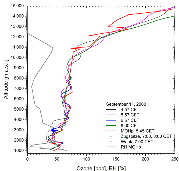
Figure 16. Ozone measurements on 11 September 2000 (see Fig. 13 of Trickl et al., 2003); in this case no offset was determined.
