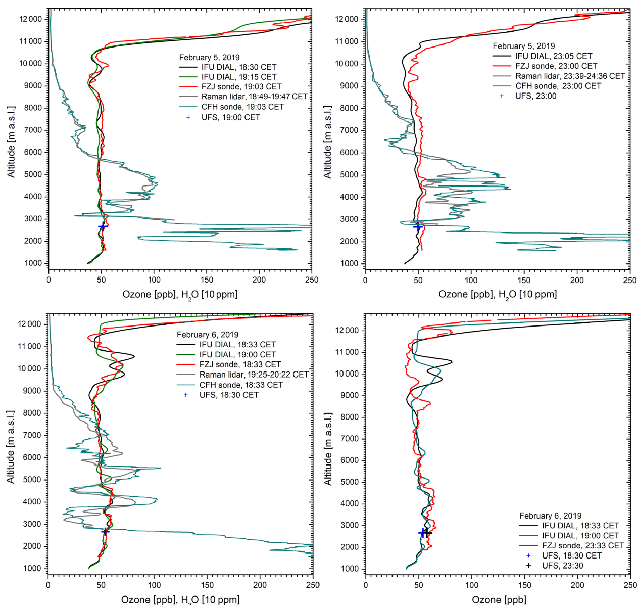
Figure 2. Four ozone measurements on 5 and 6 February 2019 with lidar (IFU), ECC sonde (FZJ) and an in situ sensor at UFS; for two measurements the FZJ ozone mixing ratios are slightly higher than the lidar results. The fourth FZJ ozone measurement took place much later than the final lidar measurements, which resulted in slightly larger differences up to 4.8 km, confirmed by the 23:30 CET measurement at UFS. The lidar results around 10 km on 6 February are uncertain owing to a cirrus correction. In order to visualize more details on the complex layering we also show water-vapour mixing ratios for roughly coinciding measurements of the UFS Raman lidar and the FZJ CFH sonde. The tropospheric structures are strongly smoothed for the lidar owing to the 1 h data-acquisition time. At 3.3 km 250 ppm corresponds to roughly 5 % RH.
