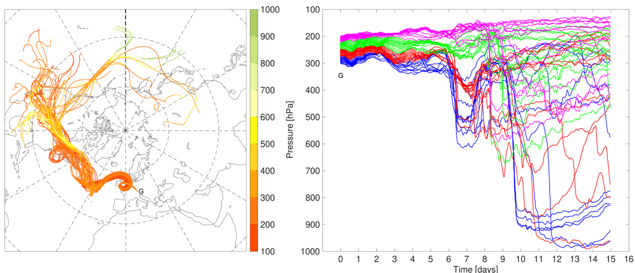
Figure 6. 350 h LAGRANTO backward trajectories, started above Garmisch-Partenkirchen (G) on 9 July 2018 at 07:00 CET.
