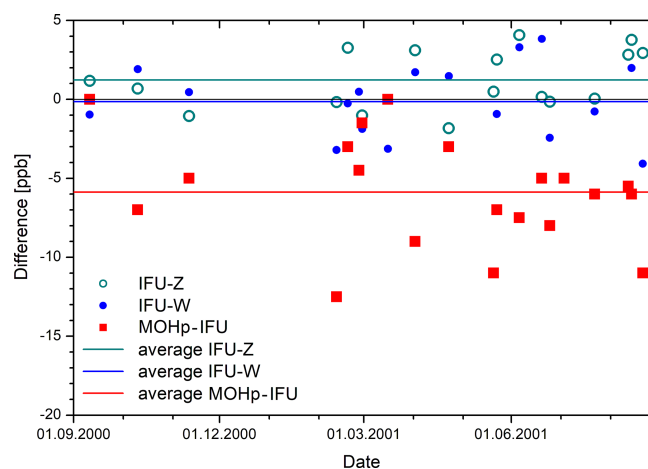
Figure 18. Differences between the ozone mixing ratios of the lidar (IFU) and the stations Zugspitze (Z), Wank (W) at the summit altitudes, and between lidar and MOHp sonde, determined by shifting the sonde profile, for the period September 2000 to August 2001.
