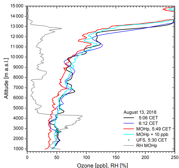
Figure 8. Ozone measurements on 13 August 2018: the agreement of the shifted MOHp ozone profile (cyan) with the lidar curves is rather good up to 12 km given the high summertime variability. The low to moderate RH above 4.4 km (grey) indicates that the elevated ozone is partially caused by stratospheric air.
