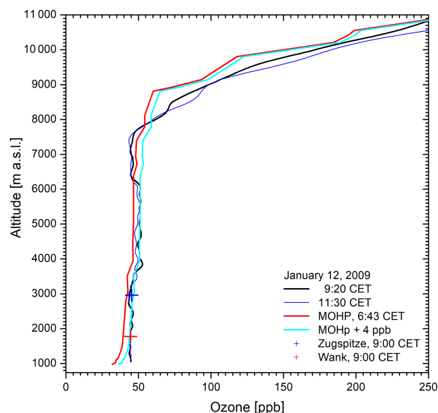
Figure 13. Ozone measurements on 12 January 2009.
