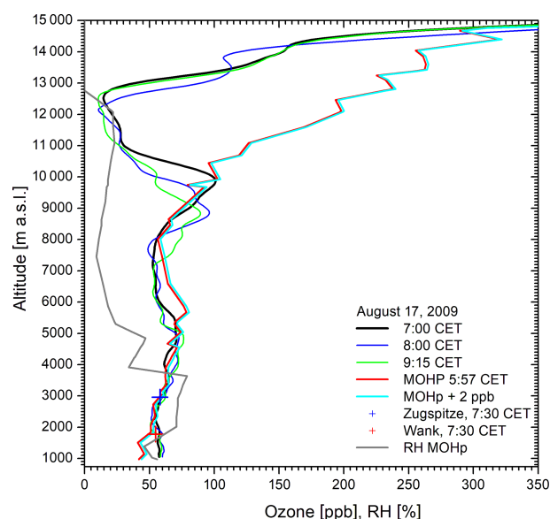
Figure 14. Ozone measurements on 17 August 2009; the structure in the upper troposphere is strongly influenced by smoothing. The bias between 5.5 and 8 km has not been explained.
