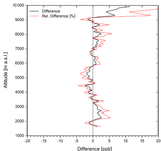
Figure 3. Averaged differences between FZJ ozone sonde and IMK-FU lidar for the first three comparisons after a slight offset correction of the sonde profiles (see text).
