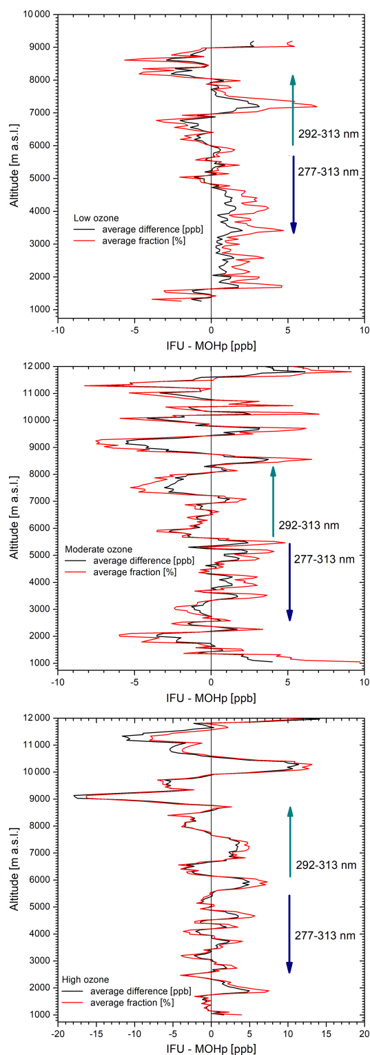
Figure 11. Average differences between IFU lidar and offset-corrected MOHp sonde in 2018 for low, moderate, and high conditions (based on six, seven, and six comparisons respectively); the uncertainties may be estimated from the maximum differences around the respective altitudes. We also indicate the approximate altitude ranges of the two wavelength pairs used for the lidar data evaluation.
