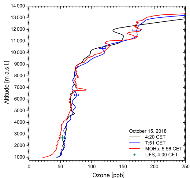
Figure 9. Ozone measurements on 15 October 2018: the MOHp ozone (red) is not shifted. The agreement above 4.3 km is better with the earlier lidar measurement (black); above 7 km it is better with the blue curve. The lidar data are strongly smoothed in the stratosphere, as can be seen from the more detailed ozone structure in the sonde data. This example is one of the two examples with a pronounced low-altitude discrepancy between lidar and sonde extending to more than 3 km.
