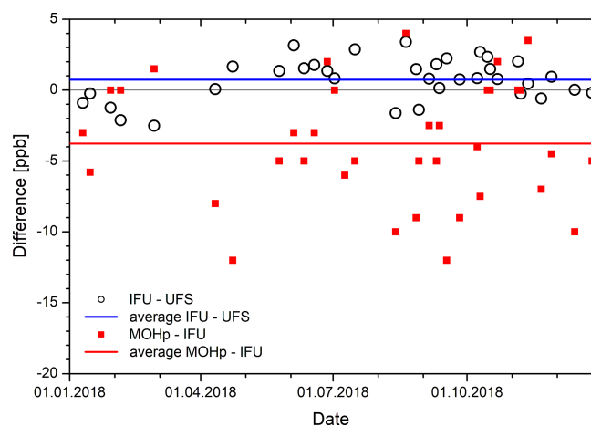
Figure 10. Differences between the ozone values of the IFU DIAL at 2670 m and the UFS routine measurements as well as the offsets of the MOHp profiles with respect to the DIAL for 35 of the 36 measurement days of the 2018 comparison. The blue and red horizontal lines are the arithmetic averages for the full year (for the values see the text).
