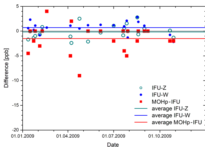
Figure 12. Differences between the ozone mixing ratios of the lidar (IFU) and the stations Zugspitze (Z), Wank (W) at the summit altitudes, and offsets between lidar and MOHp sonde for 2009.
