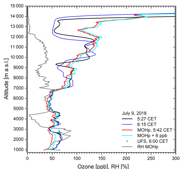
Figure 5. Summertime ozone measurements (9 July 2018) with pronounced layering; the sonde ozone (red) is brought to reasonable agreement with the lidar (black curve) above 2.7 km by adding 6 ppb (cyan curve). Above 9 km the air masses are no longer comparable. The particularly strong discrepancy of the UFS in situ ozone can be explained by orographic lifting of the ozone edge at 2.7 km. The low to moderate RH (grey) in parts of the free troposphere indicates that the elevated ozone values could be due to a stratospheric air component.
