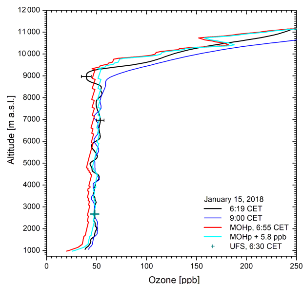
Figure 4. Ozone measurements on 15 January 2018: the MOHp ozone (red) is also shifted (cyan) by 5.8 ppb to match the lidar ozone and the UFS value (cyan), in part the black, in part the blue curve. Differences exist in the tropopause region, which is frequently the case. The sawtooth structure in the MOHp data is due to insufficient digital resolution in the NDACC database.
