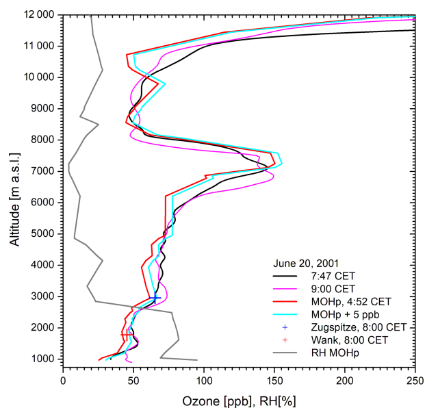
Figure 17. Ozone measurements on 20 June, 2001; the entire temporal development of the stratospheric air intrusion around 7.3 km is depicted in Fig. 6 of Zanis et al. (2003), and Fig. 3 of Trickl et al. (2010).
