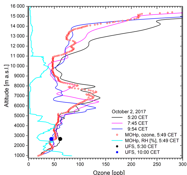
Figure 1. Ozone measurements at Garmisch-Partenkirchen (IFU, UFS) and Hohenpeißenberg (MOHp) on 2 October 2017; the low relative humidity between 5.2 and 8.3 km ( RH = 2\% ) verifies the presence of a stratospheric air intrusion. The time for MOHp is the launch time of the sonde.
