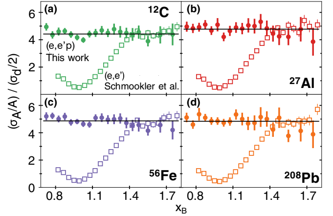
FIG. 2. Measured (e, e'p) per nucleon cross-section ratios for 350 \leq p_{\text{miss}} \leq 600 MeV/c for carbon, aluminum, iron, and lead relative to deuterium as function of x_B . Open squares are the inclusive (e, e') per nucleon cross section ratios of Ref. [26]. The horizontal lines show the average (e, e') cross section ratio for 1.45 \leq x_B \leq 1.8 [26]. Error bars show the data uncertainty (statistical plus point-to-point systematical) at the 1\sigma or 68% confidence level. Overall (e, e'p) systematic uncertainties of 10% (C) to 15% (Pb) are not shown.
