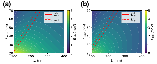
FIG. 16. Orbital splitting as a function of the geometric parameters of the SQS without disorder. (a) Minimum orbital splitting E_{\text{orb}}^x extracted from the first mode of the Fourier analysis as a function of the SQS unit-cell length L_x and the thickness of the SiGe layer ( h_{\text{SiGe}} ). (b) Calculation of the minimum orbital splitting E_{\text{orb}}^x from solving the Schrödinger equation on the full-mode periodic potential. In both (a) and (b), h_{\text{ox}} = 10 nm and V_a = 100 mV is fixed and the red line indicates L_{\text{opt}}^{\text{inh}} and the red dashed line L_{\text{opt}} .
