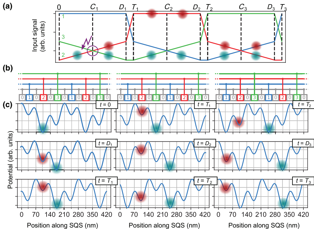
FIG. 4. Illustration of the propagation of an electron in BB mode for which the QD transfer fails once (red) and comparison with an electron, which follows the intended path (blue). (a) Three-input signal as a function of time applied to the gate sets labeled 1, 2, and 3 in (b). (b) Labeling of the clavier gates and electrical connection. Fixed voltages are applied to all barrier gates, labeled 0. (c) Sketch of the potential in the QW along the SQS channel aligned with the clavier gates in (b). The potential plotted in each subpanel corresponds to a different position time t labeled in (a). Blue circles show the intended position of the shuttled electron and red circles mark the expected electron position in the case of a failed LZR transition marked by the circle in (a).
