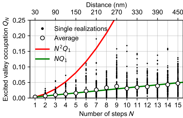
FIG. 19. Probability of occupying higher valley state after N -step passage Q_N . We use a simple model of disorder in which electron velocity v fluctuates between the realizations (filled dots) with rms \delta v = 0.1v , and for remaining parameters we take L = 15 nm, E_{\text{VS},0} = 100 \mu\text{eV} , \bar{v} = 30 m/s, \vartheta = 0.25^\circ , which corresponds to \bar{d} \sim 30 nm. To show statistical behavior, for each number of steps N we draw a new arrangement of steps with terrace lengths given by the distribution Eq. (D10) and for that arrangement simulate 200 realizations of velocity.
