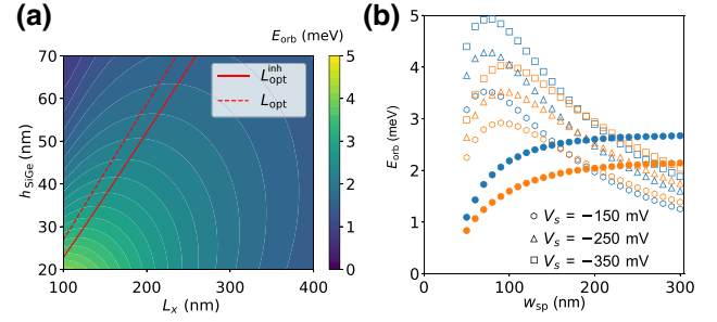
FIG. 6. Orbital splitting as a function of the geometric parameters of the SQS without disorder. (a) Using h_{\text{ox}} = 10 nm and V_a = 100 mV, the minimum orbital splitting E_{\text{orb}}^x is computed by solving the Schrödinger equation on the full-mode periodic potential. The red dashed line indicates L_{\text{opt}} and the red solid line the optimal unit-cell length for the case of inhomogeneous dielectrics L_{\text{opt}}^{\text{inh}} (discussed in Appendix A). (b) Orbital splitting E_{\text{orb}}^x (filled symbols) and E_{\text{orb}}^y (open symbols) as a function of the gap between the screening gates w_{\text{sp}} for an oxide thickness h_{\text{ox}} = 5 nm (blue symbols) and h_{\text{ox}} = 10 nm (orange symbols) and the voltage V_s applied to the screening gates [see the model in Fig. 5(b)]. A fixed sin-signal amplitude V_a = 100 mV is applied to the clavier gates and h_{\text{SiGe}} = 45 nm.
