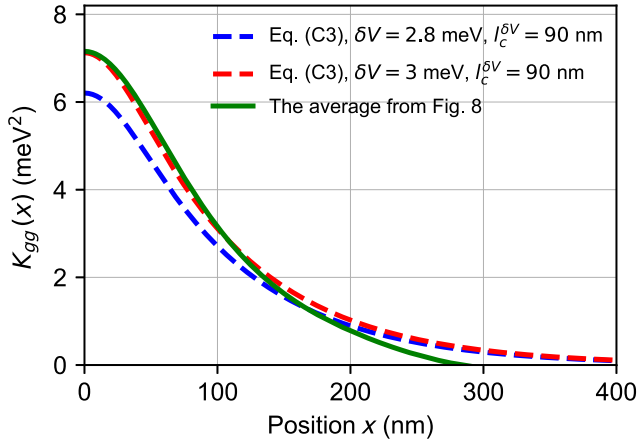
FIG. 17. Correlation function of the matrix element for the electron occupying ground orbital state K_{gg}(|x|) . With dashed lines we plot numerically integrated formulas Eq. (C3) assuming exponential form of the correlation function of effective 1D potential \langle \delta V(x)\delta V(0) \rangle = \delta V^2 e^{-|x|/l_c^{\delta V}} , with l_c^{\delta V} = 90 nm and two values of noise amplitude \delta V = 2.8 meV (blue) and \delta V = 3 meV (red). For comparison using the green solid line we plot K_{gg}(|x|) , obtained from the numerical averaging of different realizations of electrostatic disorder (see Fig. 9).
