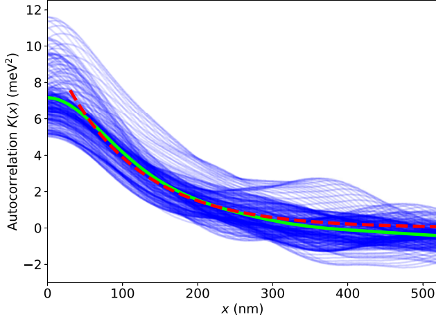
FIG. 9. Autocorrelation function K(x_0, x_0 + x) of the matrix element \delta M_{gg}(x_0) = \langle g_o | \delta V(x) | g_o \rangle , defined in Eq. (9), calculated for device geometry and voltages used in Figs. 7(d) and 7(f), and averaged over 80 disorder realizations. Blue lines correspond to 250 distinct values of x_0 . We plot averaged autocorrelation (solid green line) and an exponential fit (dashed red line) for x > L_{\text{dot}} of the K_{gg}(L_{\text{dot}})e^{-|x-L_{\text{dot}}|/l_c^{gg}} form. The fitted values \sqrt{K_{gg}(0)} = 2.8 meV and l_c^{gg} = 90 nm indicate typical amplitude and correlation length of effective 1D disorder \delta V(x) . The long correlation length l_c^{gg} \gg L_{\text{dot}} is an indicator of stability of the moving QD against potential disorder.
