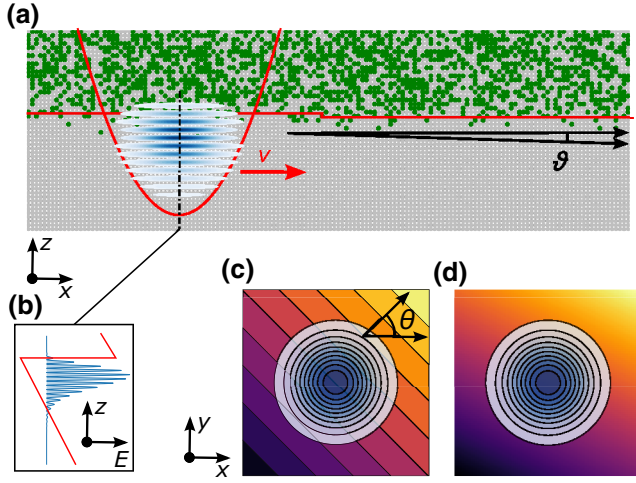
FIG. 11. Modeling of the local valley splitting across the SQS channel. (a) A 2D cross section through a Si/SiGe interface region with a gate-defined quantum dot containing the electron. A single atomistic step is indicated at the center, with Ge-alloy disorder smearing out the location of the interface. Gray dots represent Si atoms in the strained Si layer and QW barrier region, respectively. Dark green dots represent Ge atoms. The angle \vartheta indicates the average effective miscut. (b) A 1D line-cut along the growth direction, which is the model containing all short-range disorder discussed in the main text. The models describing long-range disorder in the 2D plane perpendicular to the growth direction are sketched in (c) (step model) and (d) (gradient model), with the color coding indicating the continuous and discrete spatial variation in valley phase, respectively. The angle \theta in (c) is the angle between the step normal and shuttling direction.
