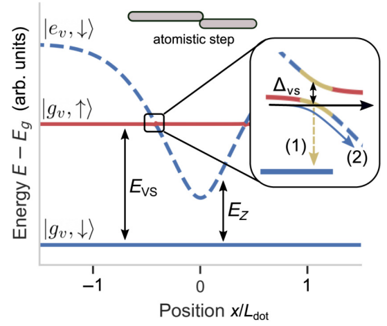
FIG. 14. Sketch of energy difference between the following states: ground valley spin-up state |g_v, \uparrow\rangle , excited valley spin-down state |e_v, \downarrow\rangle , and the lowest-lying level |g_v, \downarrow\rangle with energy E_g at the spin-valley hotspot caused by the atomistic step. Inset: enlargement of the avoided crossing between |e_v, \downarrow\rangle and |g_v, \uparrow\rangle states, where we identify two mechanisms responsible for the spin-flip error \delta p_{\uparrow} : (1) the relaxation in vicinity of avoided crossing, due to hybridization between spin and valley states (yellow arrow) and (2) adiabatic transition that converts spin up to spin down, followed by subsequent relaxation, dephasing, and possibly more nonadiabatic transitions at the subsequent level crossing (blue arrow). For illustration purposes we use arbitrary units.
