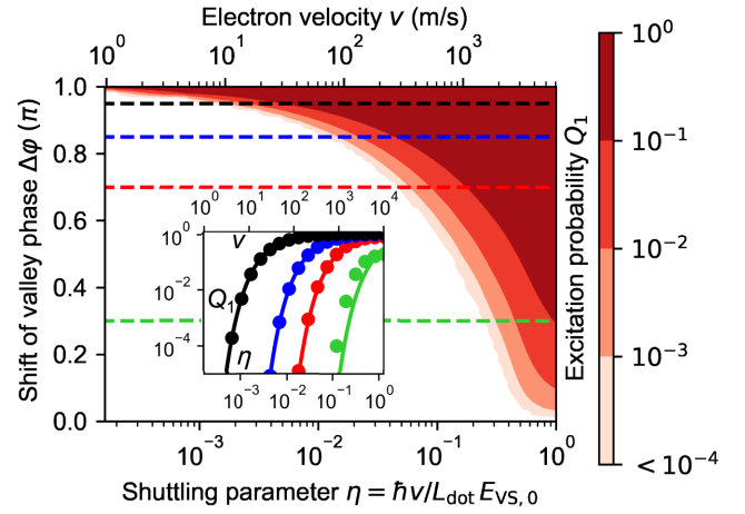
FIG. 18. Occupation of higher valley state after single-step passage Q_1 as a function of shuttling parameter \eta (lower scale) and valley field angle difference \Delta\varphi . Inset: numerical solution to Eq. (22) is compared against effective LZ approximation (30) for selection of angles \Delta\varphi/\pi = 0.3, 0.7, 0.85, 0.95 (dashed lines in larger figure). The upper x axis translates \eta into electron velocity v = L_{\text{dot}}E_{\text{VS},0}\eta/\hbar assuming typical values of L_{\text{dot}} = 20 nm and E_{\text{VS},0} = 200 \mu\text{eV} .
