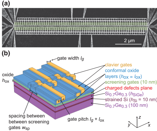
FIG. 5. Realistic Si/SiGe SQS device. (a) Scanning electron micrograph of 10- \mu\text{m} -long SQS showing three gate layers: on top of a screening gate layer (colored in green), two clavier gate layers connected to four gate sets for CB mode. Gates at the ends of the SQS are for the formation of single-electron transistors. (b) COMSOL model of the SQS device from (a) showing two SQS unit cells and thus eight clavier gates. The typical thickness of layers is given in brackets.
