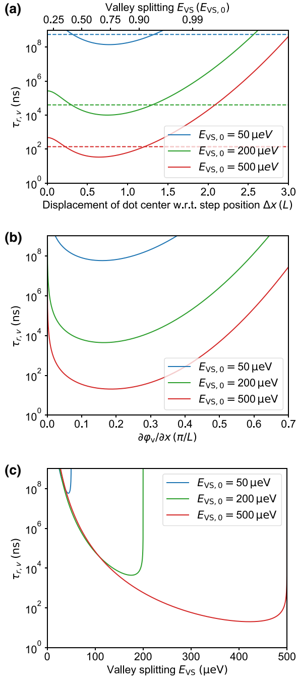
FIG. 13. Valley lifetimes for the step model (a) and linear valley phase model (b),(c). The dashed lines in (a) are the inverses of the relaxation rate averaged over the displayed region. A QD confinement energy of E_{\text{orb}} = 1 \text{ meV} is assumed for all cases.
