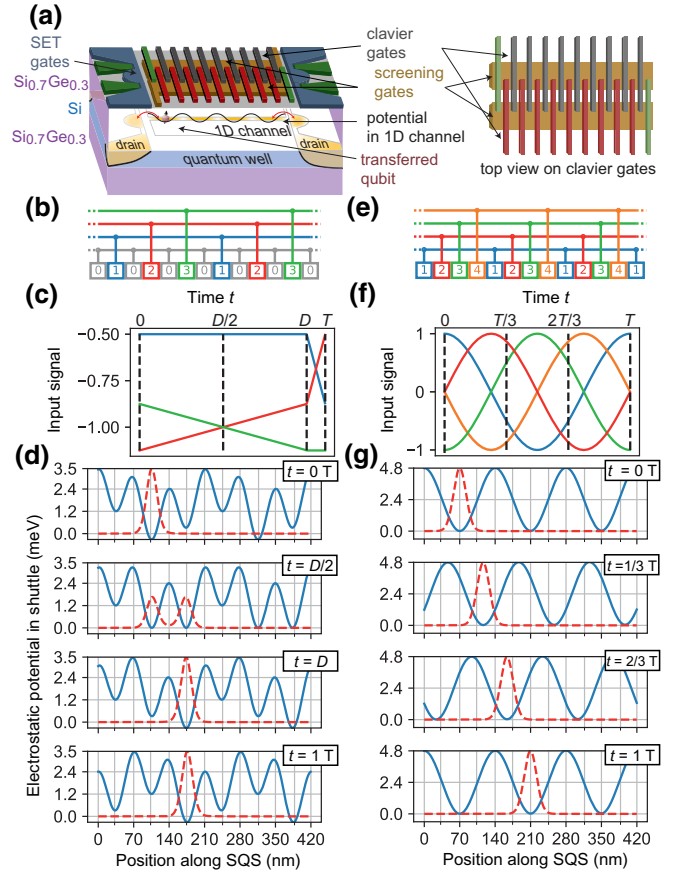
FIG. 2. SQS concept and operation modes. (a) Sketch of a SQS device. (b)–(g) Comparison of BB (left panels) and CB (right panels) transfer modes. (b),(e) Position of the clavier gates and electric connection scheme for the BB mode (b) and CB mode (e), respectively. (c),(f) Input voltages during a SQS step cycle T for the BB mode (c) and CB mode (f), respectively. (d),(g) Electrical potential (blue) calculated along the center of a SQS within the Si/SiGe quantum well for four time frames [dashed lines in (b) and (d) for each mode]. Dashed red line indicates the calculated electron density.
