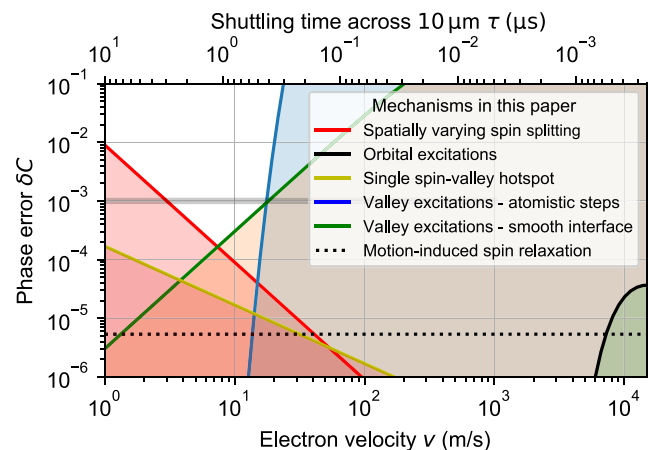
FIG. 1. Sketch of the transfer errors of an electron spin-qubit after 10- \mu m shuttling in the CB mode as a function of the shuttling velocity for various decoherence mechanisms discussed in this paper. In Sec. VIII, we discuss the detailed plots of these dependencies that summarize all the calculations in this paper.
