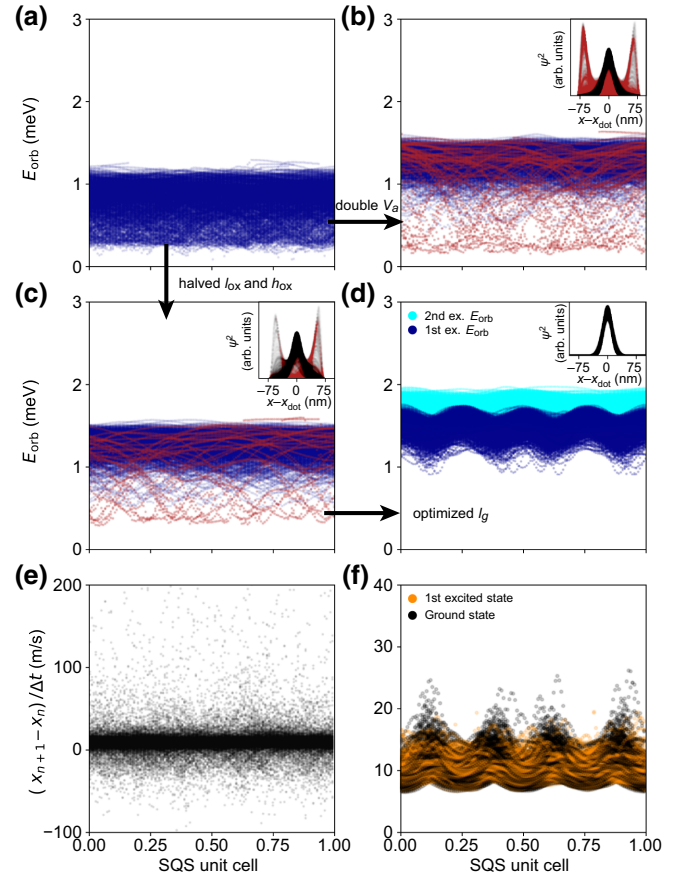
FIG. 7. Simulation based on Poisson-Schrödinger solutions of propagating potential in CB mode for 800 ensembles of randomly distributed charged defects at the Si/SiO 2 interface for h_{\text{SiGe}} = 45 \text{ nm} and w_{\text{sp}} = 200 \text{ nm} . (a) Orbital energy E_{\text{orb}} of the first excited state of the propagating QD assuming an oxide thickness h_{ox} = 10 \text{ nm} , gate width l_g = 30 \text{ nm} and signal amplitude of V_{a,1} = 45 \text{ mV} and V_{a,2} = 100 \text{ mV} applied to the first and second claviature gate layer, respectively. (b) Same as in (a) with parameters ( h_{ox} = 10 \text{ nm} , V_{a,1} = 90 \text{ mV} , V_{a,2} = 200 \text{ mV} , l_g = 30 \text{ nm} ). Inset: the probability density \int |\psi(x, y)|^2 dy of the ground electron wave function is plotted for all expected QD positions x_{\text{dot}} and all charge defect ensembles. Wave functions deviating from a single QD are marked in red together with their corresponding E_{\text{orb}} data point. (c) Same as in (b) with parameters ( h_{ox} = 5 \text{ nm} , V_{a,1} = 60 \text{ mV} , V_{a,2} = 100 \text{ mV} , l_g = 30 \text{ nm} ) and the probability density in the inset. (d) Same as in (b) and (c) with parameters ( h_{ox} = 5 \text{ nm} , V_{a,1} = 65 \text{ mV} , V_{a,2} = 100 \text{ mV} , l_g = 60 \text{ nm} ) and the probability density in the inset. In addition to the first excited orbital energy (blue dots), the second excited orbital energy is plotted (bright blue dots). (e),(f) The numerically calculated velocity for each ensemble for the ground (black) and first excited state (orange) along the SQS direction is plotted corresponding to the parameters from (a) and (d), respectively.
