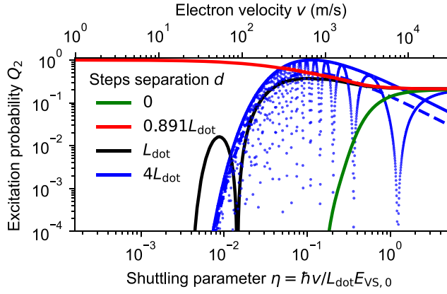
FIG. 12. Probability of occupying excited valley state, after two-step passage Q_2 for four different step separations d corresponding to double height step d = 0 (green), valley collapse d \approx 0.891L_{\text{dot}} (red), and interference d \gg L_{\text{dot}} (blue) as a function of shuttling parameter \eta (lower scale) and electron velocity v (upper scale) for fixed E_{\text{VS},0} = 200 \mu\text{eV} and L_{\text{dot}} = 20 \text{ nm} ( E_{\text{orb}} = 1 \text{ meV} ). We add the intermediate case of d = L_{\text{dot}} (black) to show that d \geq L_{\text{dot}} distances between the steps should be sufficient to avoid the valley collapse. In the interference regime (blue), we compare analytical formulas for constructive interference Q_2^{\text{max}} = 4Q_1 (solid line) and the average \langle Q_2 \rangle = 2Q_1 (dashed line) against the results of numerical simulation (dots).
