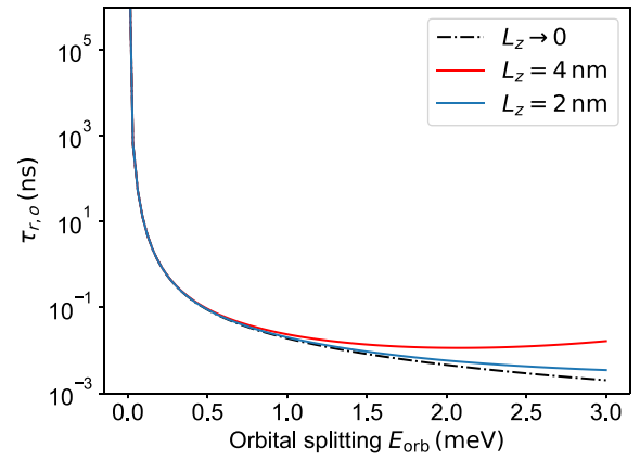
FIG. 10. Orbital relaxation time in a circular QD ( L_x = L_y ), with L_z as the remaining parameter. L_z \rightarrow 0 illustrates the fictitious case of a completely 2D electron (where phonon bottlenecking along the z direction is absent), while L_z = 4 nm is a reasonable upper bound for the localization of the electron wave function in z direction.
