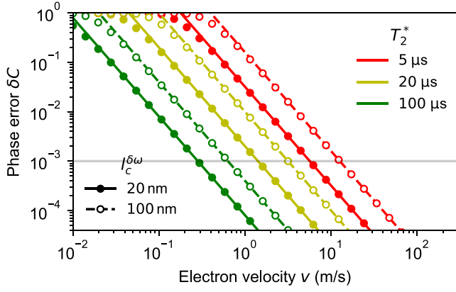
FIG. 8. Improvement of spin coherence of an electron transferred adiabatically along a 10\ \mu\text{m} long channel with its velocity. We plot the coherence error due to quasistatic noise as a function of velocity for dephasing times of static spin T_2^* = 5, 20, 100\ \mu\text{s} , and two values of spatial autocorrelation length of quasistatic disorder in spin splitting: l_c^{\delta\omega} = 20\ \text{nm} (corresponding to typical QD size) and l_c^{\delta\omega} = 100\ \text{nm} \approx l_c^{\delta V} (corresponding to typical electrostatic disorder autocorrelation length, see Fig. 9). Lines correspond to Eq. (4) that holds when \delta\phi \ll 1 , while circles correspond to the formula, \delta C = 1 - e^{-\delta\phi^2/2} , which holds for Gaussian statistics of random phase fluctuations.
