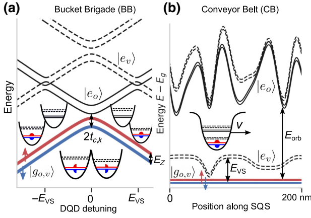
FIG. 3. Schematic picture of the energy spectrum during transfer of spin superposition in the presence of orbital (ground and first excited only), valley, and spin degrees of freedom, as a function of (a) DQD detuning \epsilon in a single transition between the QDs in bucket brigade (BB), (b) position along the SQS in the conveyor belt (CB). We denote excited valley states |e_v\rangle using dashed line and the joint ground state of orbital and valley degrees of freedom |g_{o,v}\rangle by thicker: blue (spin down) and red (spin up) line. In the insets, we illustrate mechanism of electron shuttling in each mode, note that in contrast to BB mode the charge transfer in CB does not require effectively adiabatic evolution in the lowest energy levels. In the conveyor belt (b), we plot the energy difference between excited and ground orbital levels, including expected electrostatic disorder (see Sec. III B). We also include the modification of energy spectrum due to atomistic steps (left kink) and a smooth interface gradient (right kink), that lead to temporal reduction of valley splitting E_{VS} .
