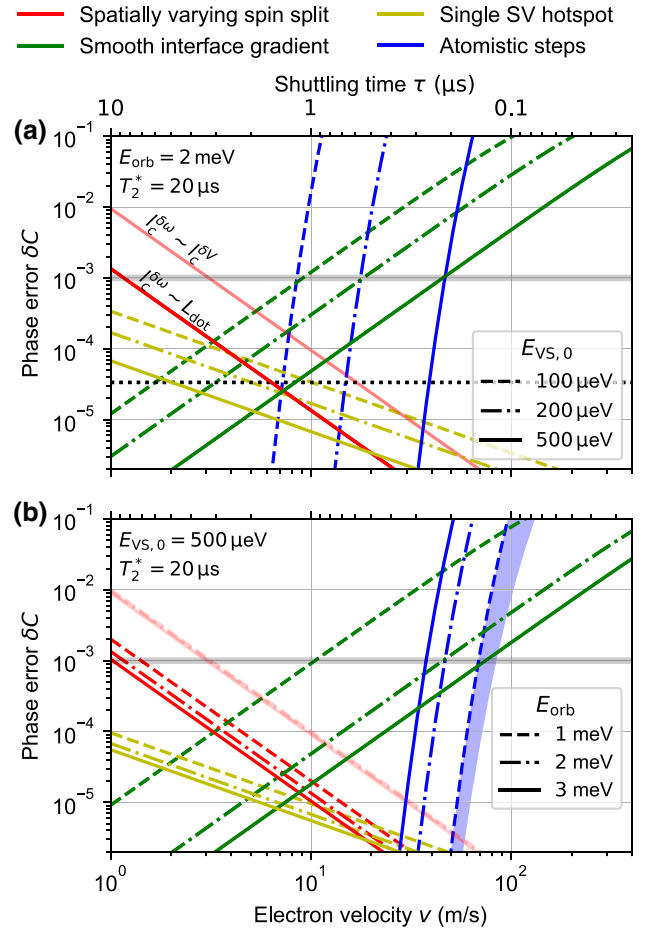
FIG. 15. Expected loss of spin coherence \delta C experienced by an electron shuttled through 10- \mu\text{m} -long SQS as a function of electron velocity v (lower axes) and shuttling time \tau (upper axes). We compare various contribution to such an error: spatial variation of precession frequency (red lines, Sec. IV), single spin-valley hotspot due to intrinsic spin-orbit coupling (yellow, Sec. VII E) and nonadiabatic effects in valley degrees of freedom caused by smooth gradient (green, Sec. VII B) and sharp atomistic steps (blue, Sec. VII C). We distinguish between the magnetic noise due to nuclear spins (darker red line) and the charge noise (lighter red line). We highlight that hotspot contribution is the only one caused by spin-relaxation process, for which \delta p_{\uparrow} \sim \delta C . The corresponding error should be multiplied by the number of hotspots in the SQS (i.e., no hotspots for E_z \ll E_{\text{VS}} ). (a) \delta C for relevant values of effective valley splitting E_{\text{VS},0} = 100, 200, 500 \mu\text{eV} (dashed, dashed-dotted, and solid lines, respectively) for fixed E_{\text{orb}} = 2 \text{ meV} and T_2^* = 20 \mu\text{s} . (b) \delta C , but for different values of orbital energy E_{\text{orb}} = 1, 2, 3 \text{ meV} (dashed, dashed-dotted and solid lines, respectively) for fixed values of E_{\text{VS},0} = 500 \mu\text{eV} and T_2^* = 20 \mu\text{s} . The results are drawn for the gradient of a_x \approx 0.05\pi/\text{nm} (corresponding to intentional miscut angle \vartheta \approx 0.5^\circ ), average step separation \bar{d} = 30 \text{ nm} ( \vartheta \approx 0.25^\circ ) and magnetic field of B = 100 \text{ mT} . The effect of decreasing magnetic field to B = 20 \text{ mT} is illustrated by a shaded regions. For plotted range of velocities v \ll L_{\text{dot}} E_{\text{orb}}/\hbar , \delta C due to orbital nonadiabaticity is exponentially small. For comparison in (a) we use a black, dotted line to plot probability of spin relaxation during the transfer from Ref. [33] and Eq. (14).
