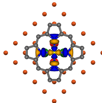
Fig. 8 Superposition of the ^{p^{\text{mc}}\sigma^* 12b_{1g}\text{-based MO (LUMO+2)}^{37}} 3D CP to the ^{nn}\text{Cu}_{\text{ffa}}^{\text{S}} 4s AOs SALC of symmetry b of the bulk terminated Cu(100). Ni–N bonds are aligned with the \langle 001 \rangle directions. Large red and green spheres represent \text{Cu}^{\text{S}} 4s AOs and corresponding different phases.
