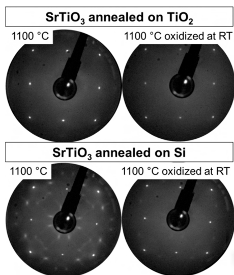
Figure 12. The LEED pattern changed after exposure to oxygen (approximately 150 Langmuirs) in the UHV at the RT for a SrTiO 3 (001) surface previously annealed on TiO 2 and one annealed on Si. The electron energy is equal to 106 eV.
