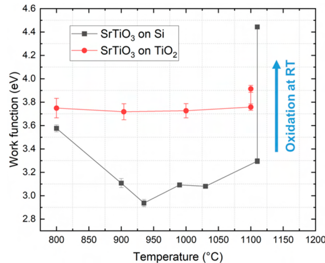
Figure 13. Relationship between the work function and annealing temperature for SrTiO 3 , which was annealed on an oxygen-getter material Si and a non-getter material TiO 2 and subsequently oxidized with approximately 150 Langmuirs of oxygen at room temperature in situ.
