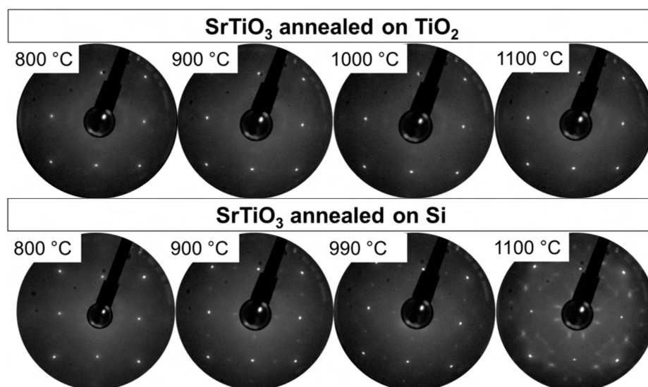
Figure 11. Temperature-dependent changes in the SrTiO 3 (001) surface crystallography when annealed in the presence of a non-getter (TiO 2 ) and an oxygen-getter material (Si). LEED patterns were made for 106 eV. The Si or TiO 2 crystals were used as a heater in a sandwiched sample mount for direct current heating.
