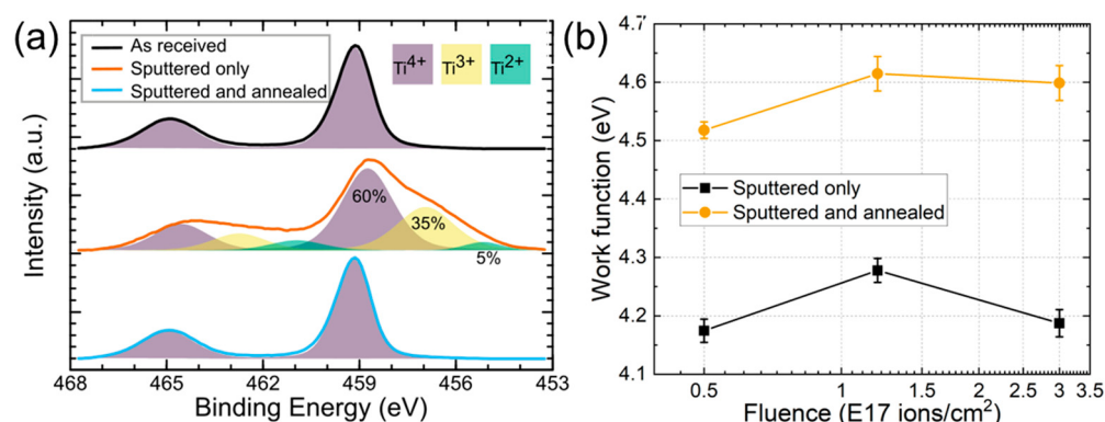
Figure 5. (a) The XPS spectra of the as-received \text{TiO}_2(110) , sputtered only \text{TiO}_2(110) (ion energy 2 keV, fluence: 8.0 \times 10^{15} ions \text{cm}^{-2} , RT), and a \text{TiO}_2(110) surface that was sputtered and subsequently annealed (ion energy 2 keV, fluence: 8.0 \times 10^{15} ions \text{cm}^{-2} , at 800 °C), (b) Effect of the fluence on the work function for sputtered only (ion energy 2 keV, RT) and sputtered and annealed (ion energy 2 keV, 800 °C) \text{TiO}_2(110) . Reprinted from [59].
