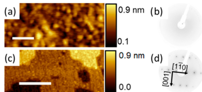
Figure 4. (a) Morphology of the sputtered \text{TiO}_2(110) surface (RT, ion energy 2 keV, fluence 1 \times 10^{17} ions \text{cm}^{-2} ) as shown on an AFM image (scale bar: 100 nm) with (b) the corresponding LEED diffraction pattern (energy: 106 eV); (c) the sputtered and annealed (ion energy 2 keV, fluence: 1.2 \times 10^{17} ions \text{cm}^{-2} , at 800 °C) surface as seen on the STM image (scale bar: 30 nm, sample bias 1.5 V) with (d) the LEED pattern (energy 106 eV). AFM and STM images reprinted from [59].
