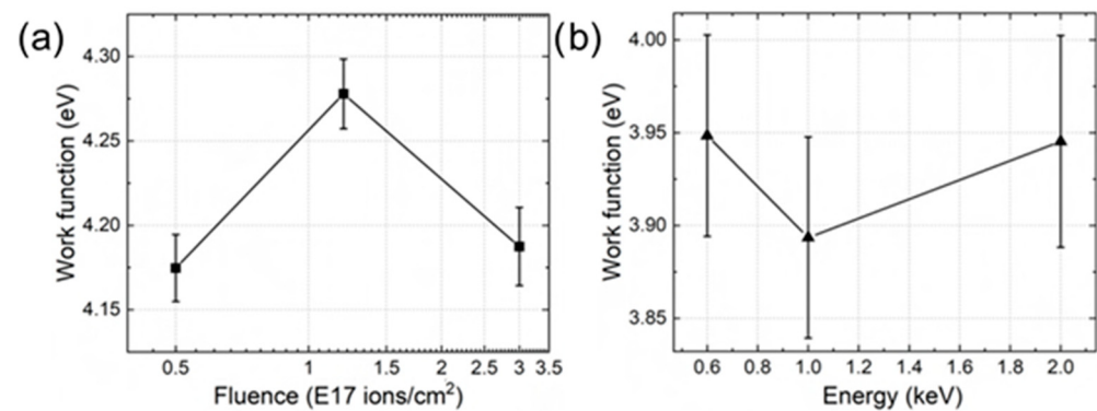
Figure 3. The work function of the \text{TiO}_2(110) surface dependence on (a) the applied ion beam fluence of \text{Ar}^+ ions (with an energy of 2 keV, RT) and (b) energy of \text{Ar}^+ ions (with a fluence of 1 \times 10^{17} ions \text{cm}^{-2} , RT). Reprinted from [59].
