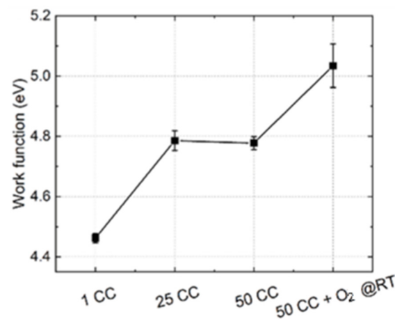
Figure 8. The effect of oxidation at RT on the work function of rutile TiO 2 (110) which underwent multiple cleaning cycles. Cycles were composed of sputtering with argon ions of 2 keV, fluence of 8.6 \times 10^{15} ions cm -2 , and then subsequent annealing at 800 °C. Oxidation proceeded at RT with 310 Langmuirs of oxygen. Reprinted from [59].
