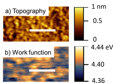
Figure 1. (a) The morphology of the sputtered TiO 2 (110) surface (RT, ion energy 2 keV, fluence 1 \times 10^{17} ions cm -2 ) as shown on a KPFM image (scale bar: 200 nm) and (b) the corresponding work function map.
