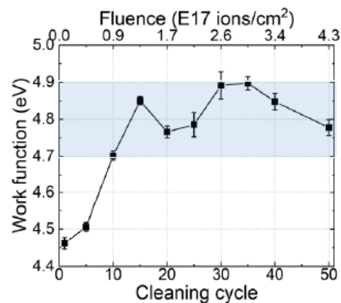
Figure 6. Relationship between the work function of \text{TiO}_2(110) and the number of sputtering/annealing cycles that the sample underwent and the total fluence the sample received. The shadow represents the leveling-off value of the work function. The sputtering was performed for argon ions of 2 keV, fluence of 8.6 \times 10^{15} \text{ ions cm}^{-2} , and the subsequent annealing at 800^\circ\text{C} . Reprinted from [59].
