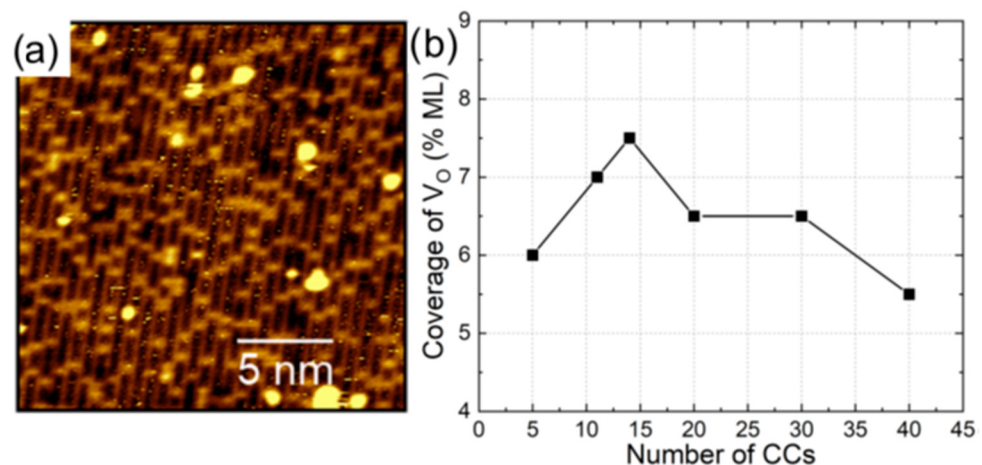
Figure 7. (a) Typical STM image of \text{TiO}_2(110) on which the defects coverage calculations were based. This image shows the typical topography of an 11 CCs sample (sample bias 1.7 V and current 11 pA; cycles were composed of sputtering with argon ions of 2 keV, fluence of 8.6 \times 10^{15} \text{ ions cm}^{-2} , and then subsequent annealing at 800^\circ\text{C} ); (b) the relationship between the coverage of oxygen vacancies and the number of CC.
