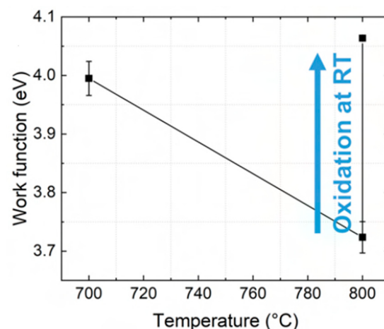
Figure 9. The changes in the rutile TiO 2 (110) work function for crystals annealed in UHV at 700 °C and then 800 °C and subsequently oxidized at room temperature in UHV (oxygen exposure equal to 1260 Langmuirs).
