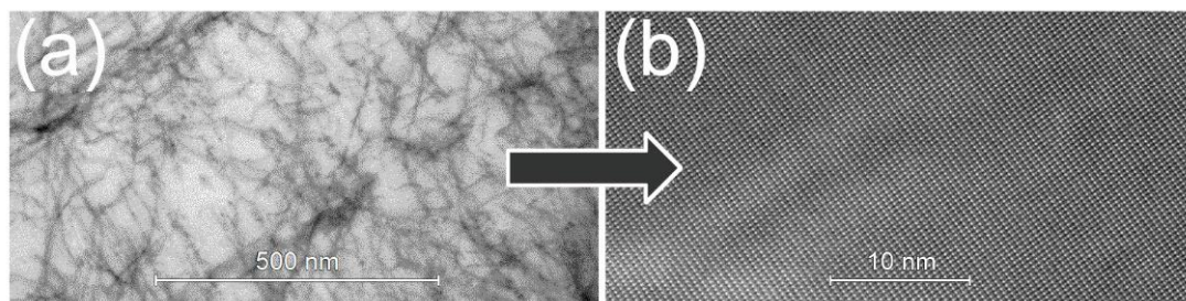
Figure 2. (a) STEM-HAADF image of the dislocation network in STO crystal. (b) Atomically resolved STEM-HAADF image of STO.
