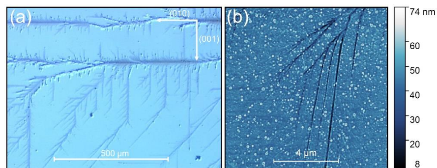
Figure 4. The STO crystal after the electron current discharge as observed by: (a) optical microscopy, (b) topography by atomic force microscopy.
