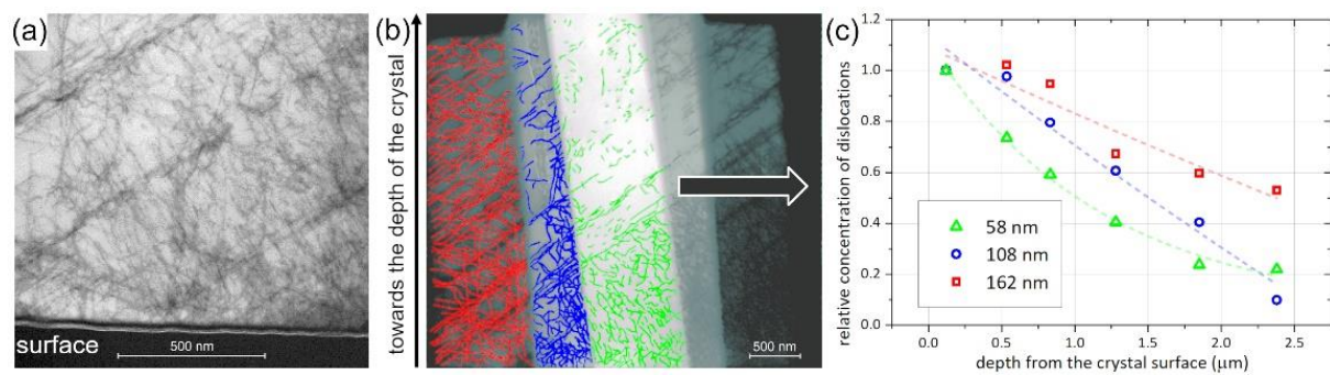
Figure 3. (a) STEM-HAADF image of the STO wedge-type lamella obtained by the Ga FIB thinning from a mechanically modified sample, (b) the lamella regions with different thicknesses and dislocations marked, and (c) the dislocation concentration as a function of depth from the crystal surface obtained for particular lamella thickness from the STEM-HAADF images. The presented data is shown as a relative dislocation concentration for clarity. The colors correspond to different lamella thicknesses: 58 nm to 79 nm—green, 108 nm to 206 nm—blue, and 162 nm to 343 nm—red.
