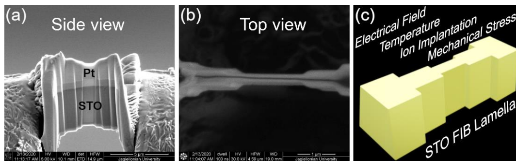
Figure 1. The side (a), the top (b) view, and (c) the wedge geometry of the STO cross-section (lamella).
