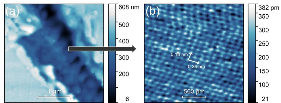
Figure 5. The AFM topography of a crater created on the STO crystal surface under electron irradiation: (a) 3 \times 3 \mu\text{m} region, and (b) atomic resolution of the region on the bottom of the crater.
