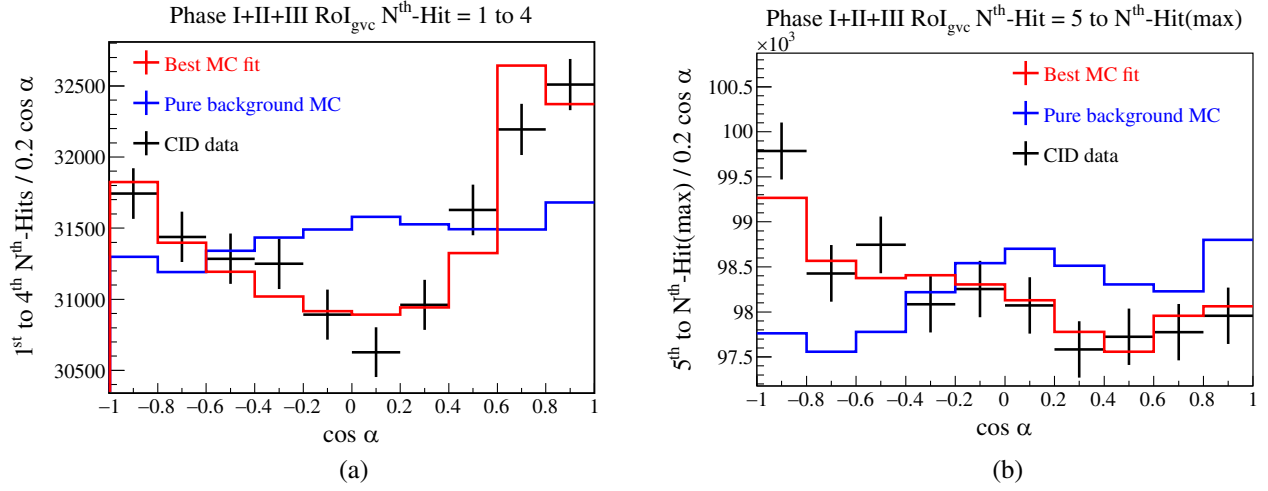
FIG. 5. The CID data (black) and the best fit results (red) for the measurement of the g_{\text{vch}} parameter. While the analysis is done separately for Phase-I and Phase-II + III, here, the sum of Phase-I + II + III is shown for illustration purposes. There are in total 7.86 \times 10^4 events in the \text{RoI}_{\text{gvc}} . The best fit for the constrained number of neutrino events is N_\nu = 5.00 \times 10^4 , while the best fit values for the parameter of interest are g_{\text{vch}} = 0.140 \text{ ns m}^{-1} for Phase-I and g_{\text{vch}} = 0.089 \text{ ns m}^{-1} for Phase-II + III. For comparison, the background MC (blue) scaled to the same total number of events is shown. (a) The sum of the first to fourth N^{\text{th}} -hits \cos \alpha histograms shows the Cherenkov peak. (b) The sum of the fifth to the N^{\text{th}} -hit(max) \cos \alpha histograms shows the effect the \Delta r_{\text{dir}} parameter on the later hits.
