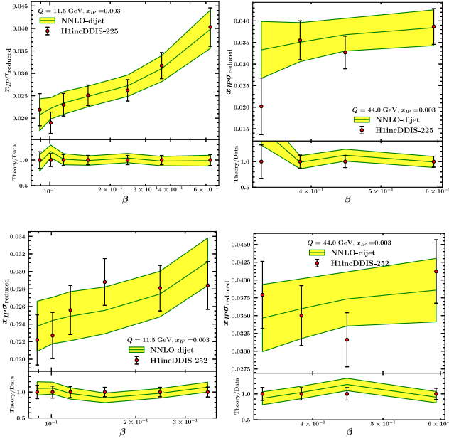
FIG. 9. Comparison of the NNLO theory prediction for the inclusive diffractive cross section obtained using the SKMHS23-dijet with the H1-LRG-11 \sqrt{s} = 225 GeV and H1-LRG-11 \sqrt{s} = 252 GeV inclusive diffractive DIS datasets. Both the absolute distributions (upper) and the data/theory ratios (lower) are shown.
