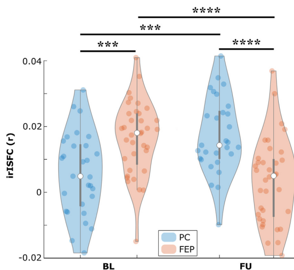
Figure 3. Mean independent-reference intersubject functional connectivity (irISFC) within the interaction network separately for the population control (PC) and first-episode psychosis (FEP) groups at baseline (BL) and follow-up (FU). The violin plots show the median (white dot), interquartile range (black vertical bar), the lower/upper adjacent values (thin black vertical lines extending from the bar) together with kernel density estimates and individual data points. Asterisks indicate statistically significant differences (*** p < .001 , **** p < .0001 ).
