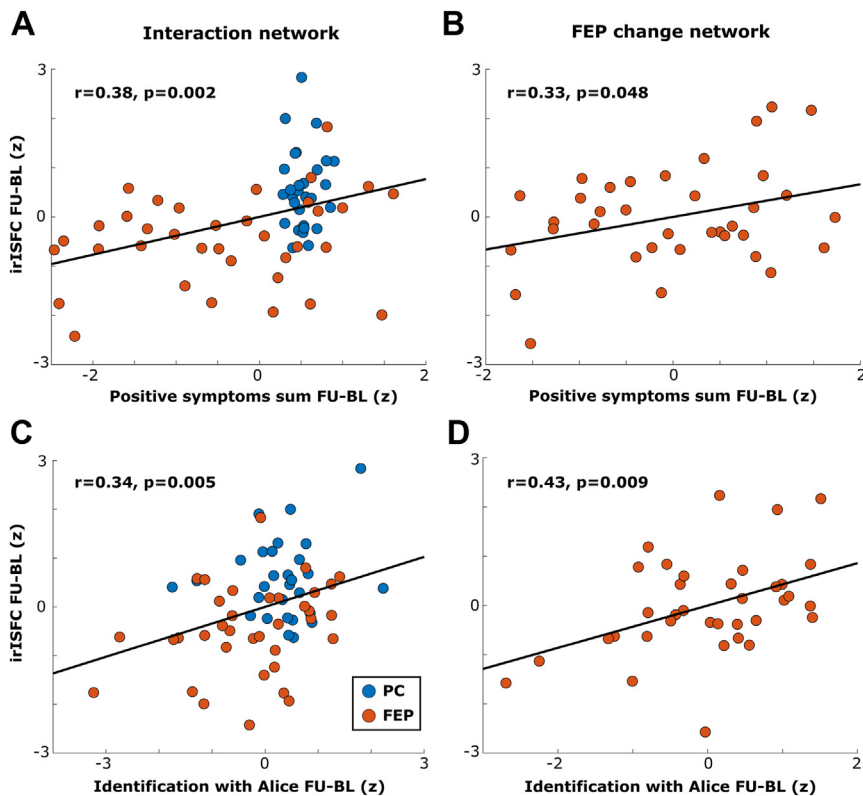
Figure 4. Correlation of network connectivity with positive symptoms and identification. (A) The longitudinal change in positive symptom sum scores plotted against the longitudinal change in the independent-reference intersubject functional connectivity (irISFC) in the interaction network. (B) The longitudinal change in positive symptom sum scores plotted against the longitudinal change in the irISFC in the first-episode psychosis (FEP) change network. (C) The longitudinal change in the subjective rating of how strongly the participants identified with the movie stimulus protagonist Alice and the longitudinal change in the irISFC in the interaction network. (D) The longitudinal change in the subjective rating of how strongly the participants identified with Alice and the longitudinal change in the irISFC in the FEP change network. The irISFC values were averaged across the connections within the network. The plotted values are the standardized z scores (with 0 mean and unit variance) of the residuals after regressing out antipsychotic medication dose and framewise displacement from both the irISFC values and the symptom/behavioral scores. BL, baseline; FU, follow-up; PC, population control.
