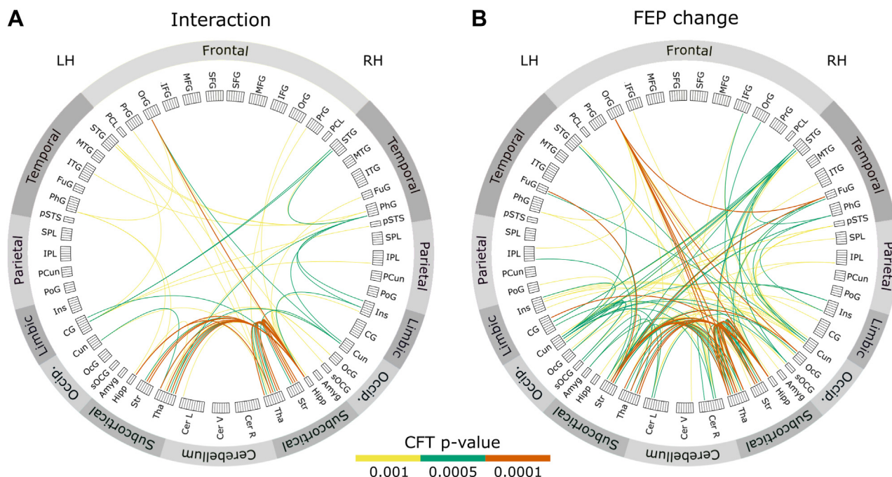
Figure 2. Differences in extrinsic brain networks between groups and time points. (A) Network showing statistically significant group (first-episode psychosis [FEP] vs. population control) \times time of visit (baseline vs. follow-up) independent-reference intersubject functional connectivity interaction and (B) network showing significantly stronger independent-reference intersubject functional connectivity at baseline than at follow-up in the FEP group. The outer circle shows the lobes of the brain, and the inner circle shows the brain regions within the lobes. The color of the connection indicates the cluster-forming threshold (CFT). The connections are multiple comparisons corrected at p < .05 using network-based statistics (20). Regions are from the Brainnetome atlas. Amyg, amygdala; Cer, cerebellum; CG, cingulate gyrus; Cun, cuneus; FuG, fusiform gyrus; Hipp, hippocampus; IFG, inferior frontal gyrus; Ins, insula; IPL, inferior parietal lobule; ITG, inferior temporal gyrus; L, left; LH, left hemisphere; MFG, middle frontal gyrus; MTG, middle temporal gyrus; occip, occipital; OCG, occipital gyrus; OrG, orbital gyrus; PCL, paracentral lobule; PCun, precuneus; PhG, parahippocampal gyrus; PoG, postcentral gyrus; PrG, precentral gyrus; pSTS, posterior superior temporal sulcus; R, right; RH, right hemisphere; SFG, superior frontal gyrus; sOCG, superior occipital gyrus; SPL, superior parietal lobule; STG, superior temporal gyrus; Str, striatum; Tha, thalamus; V, vermis.
