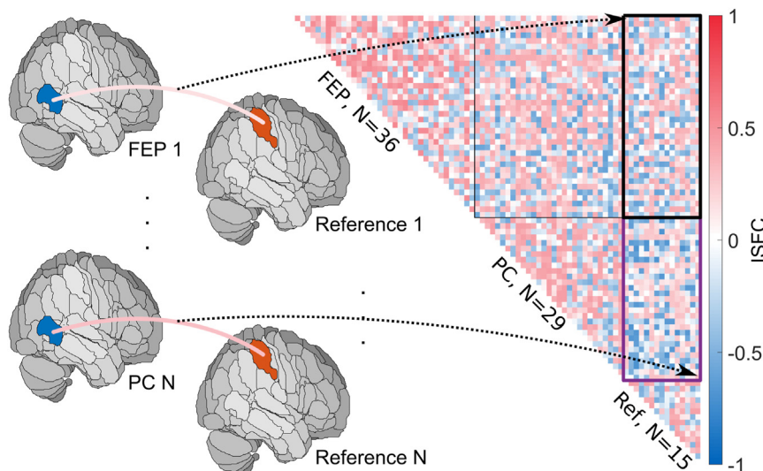
Figure 1. Schematic illustration of the independent-reference intersubject functional connectivity (ISFC) method. The figure shows the calculation of independent-reference ISFC between 2 exemplar brain regions (highlighted in blue and red on the left). In both the first-episode psychosis (FEP) and population control (PC) groups, intersubject interregional temporal correlations of the functional magnetic resonance imaging signals were calculated across all pairs of brain regions with respect to the reference group of 15 independent PC participants. The resulting correlation matrices (on the right) were averaged over the 15-PC reference group to obtain a single connectivity value per participant per brain region pair. Repeating the illustrated calculation for all pairs of brain regions results in a region-to-region (272 × 272) connectivity matrix for each FEP and PC participant.
