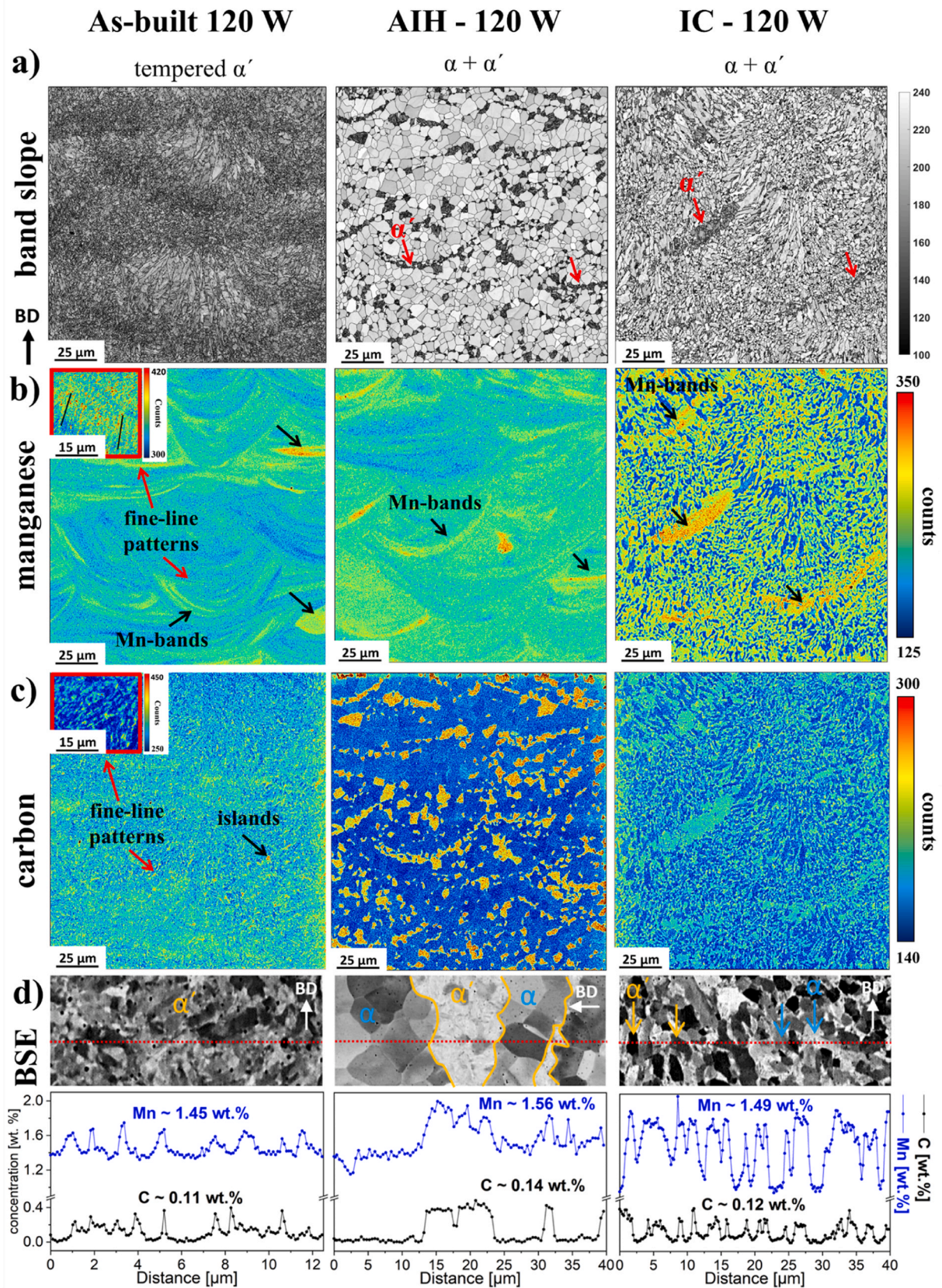
Fig. 6. EPMA results of as-built and heat-treated 120 W samples acquired from the middle of the cross-sections parallel to BD. (a) EBSD band-slope maps. (b) Mn and (c) C intensity maps (in counts). Close-up frames display additional measurements performed to visualize the fine-line Mn and C partitioning in more detail. (d) EPMA line scans and corresponding BSE images showing the local C and Mn distribution in the as-built and heat-treated 120 W samples. The red dashed lines represent the locations of the line-scans. Orange and blue colors show \alpha' and \alpha , respectively.
