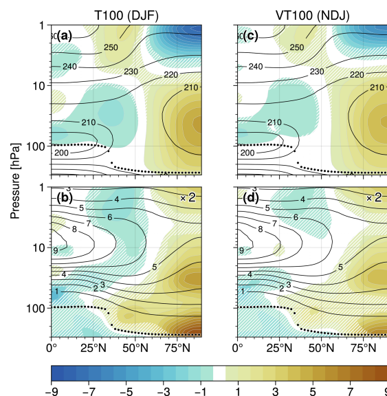
Figure A1. Interannual anomalies (seasonal means, DJF) of zonal-mean temperature (in units of Kelvin, a and c ) and ozone ( b and d ), regressed on the T100 index (DJF, a and b ) and the VT100 predictor (NDJ, c and d ), which are both described in Sect. 2. Note the time lag for the VT100 time series. The ozone responses (in percent) are provided relative to the DJF climatology and have been scaled by a factor of 0.5 before plotting. Black contour lines show the corresponding climatologies (in Kelvin and parts per million by volume for temperature and ozone, respectively) and hatches indicate where the regressions are not statistically significant. The thick dotted lines indicate the seasonal-mean thermal tropopause. All results were obtained from ERA-Interim reanalysis data.
