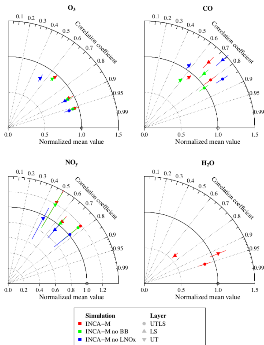
Figure 6. Modified Taylor diagrams synthesizing the assessment of the yearly climatologies beyond 25° N derived from the three LMDZ-OR-INCA simulations against IAGOS-DM, for \text{O}_3 , \text{CO} , \text{NO}_y and \text{H}_2\text{O} . Each simulation is represented by a colour and each layer by a point shape. The radial axis corresponds to a normalized mean value. The orthoradial axis refers to the r correlation coefficient. The error bars are the quartiles 1 and 3 of the relative bias.
