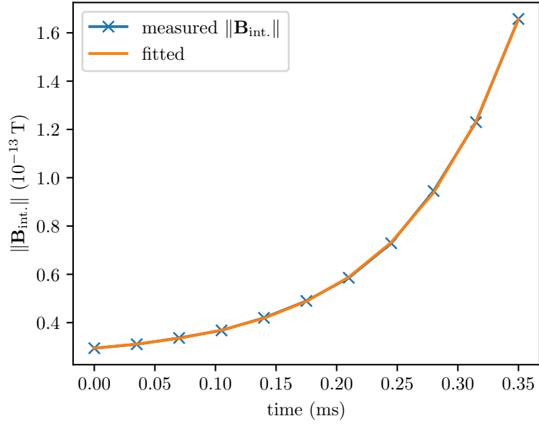
FIGURE 6.23: Time evolution of local \|B_{\text{int.}}\| at \rho = 6.05 m and z = -1 m. The numerical fit of Eq. 6.14 is shown as well. This numerical extrapolation is performed at every grid point in Fig. 6.24.
