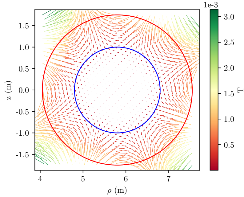
FIGURE 7.1: \mathbf{B}_\theta vector field of Sce. 5.
