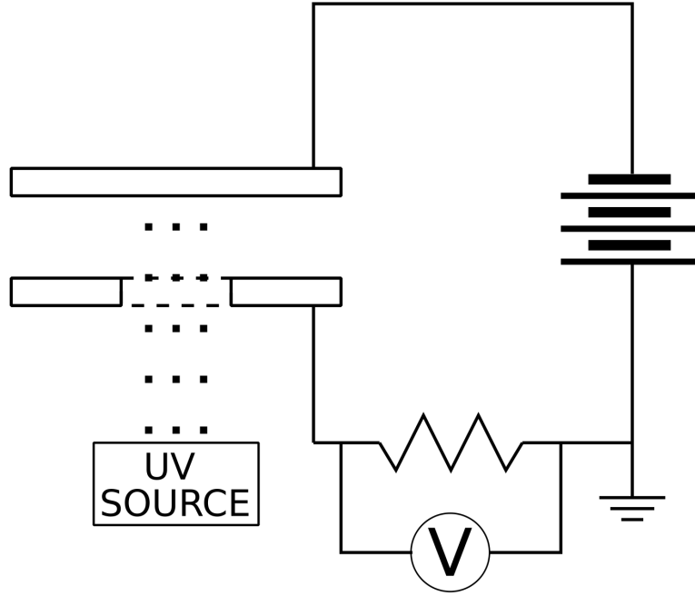
FIGURE 5.1: Townsend avalanche experiment setup.
