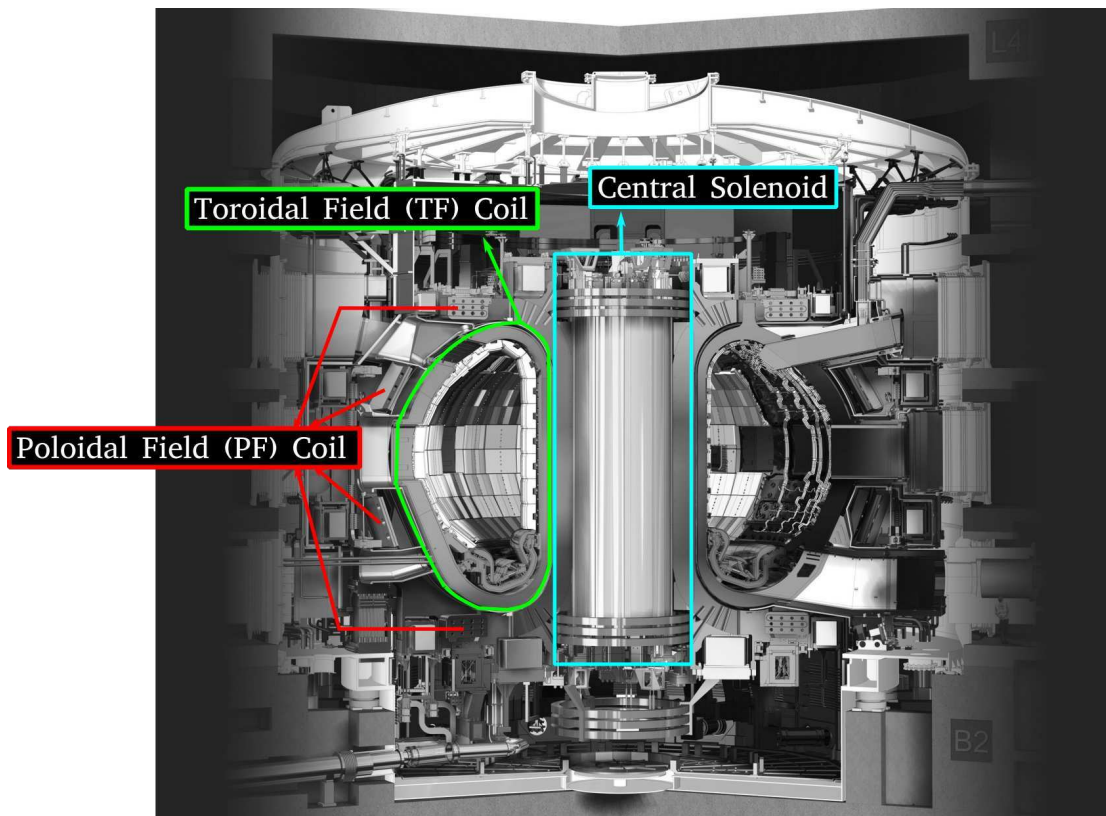
FIGURE 2.3: Magnetic coil placements in ITER.
