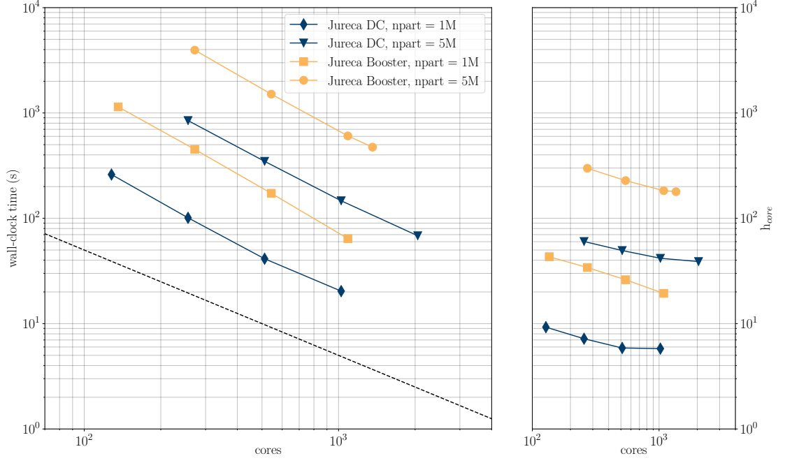
FIGURE 3.1: Left: Strong scaling of PEPC on the Jureca-DC and Jureca booster partitions for a problem size of 10^6 and 5 \times 10^6 particles taken from the tokamak Townsend discharge scenario run for 100 timesteps, without I/O. All accompanying physics and in-development merging algorithm are included. Right: The corresponding required core-hours.
