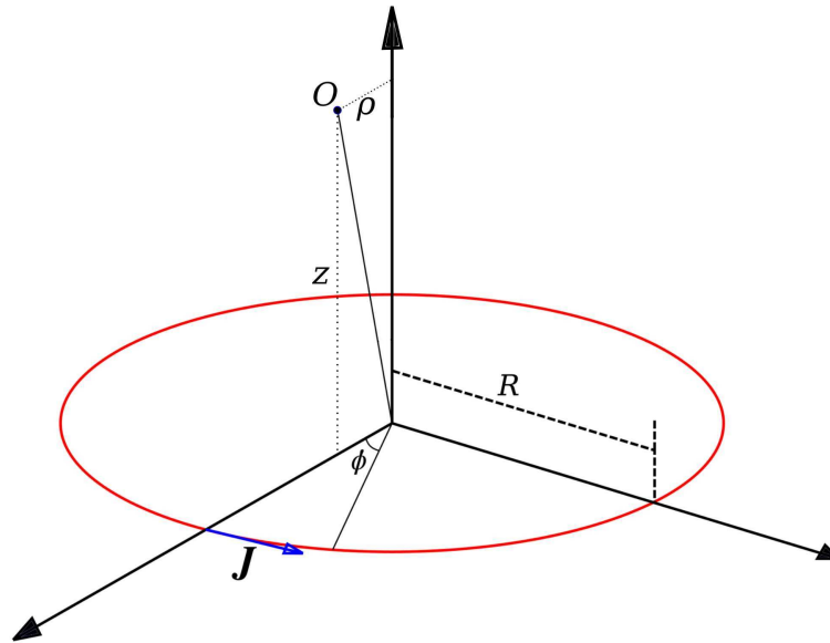
FIGURE 3.9: Current loop setting in cylindrical coordinate system.
