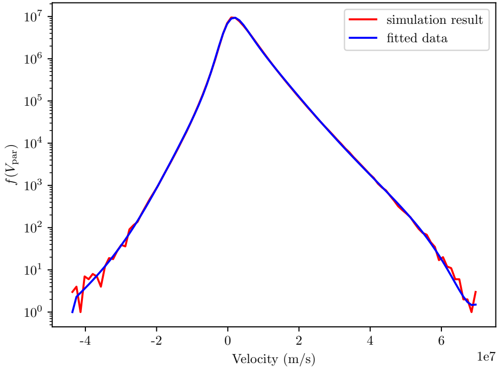
FIGURE 7.4: Electron V_{\text{par}} distribution for Sce. 5 at 0.91 ms.
