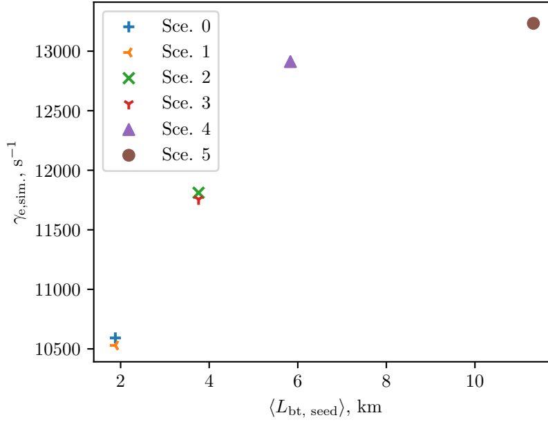
FIGURE 7.8: \gamma_{e,\text{sim.}} with its respective \langle L_{\text{bt, seed}} \rangle for all considered scenarios.
