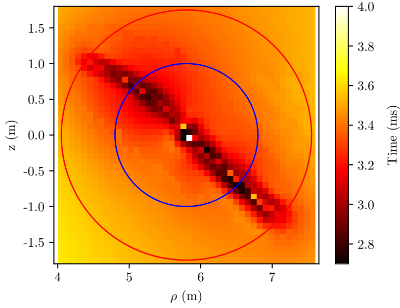
FIGURE 6.24: Computed t_{\text{crit.}} across the poloidal plane.
