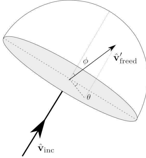
FIGURE 3.4: Allowed scattering angle for freed electron.
