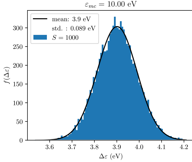
FIGURE 4.10: Distribution of \Delta\epsilon with S = 1000 , accompanied by a fitted Gaussian.
