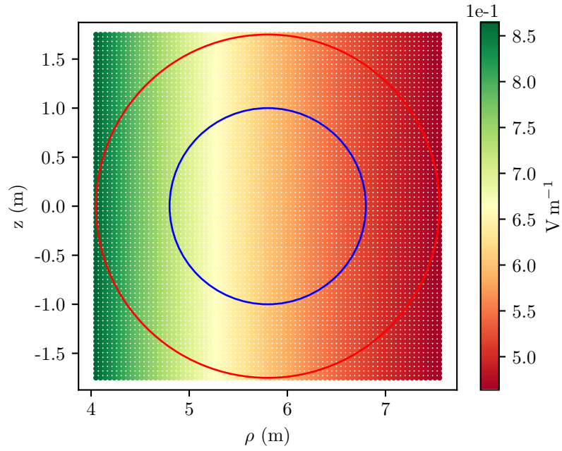
FIGURE 6.5: Toroidal electric field strength in the poloidal plane, \mathbf{E}_\phi is pointing out of the figure.
