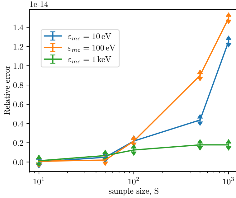
FIGURE 4.6: Relative error of total energy for S = [10, 50, 100, 500, 1000] at various \varepsilon_{mc} .
