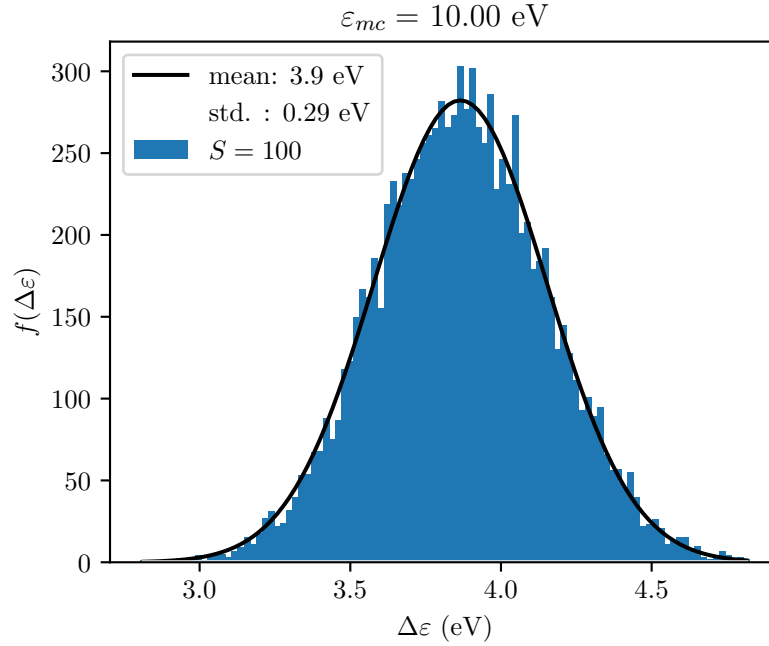
FIGURE 4.9: Distribution of \Delta\varepsilon with S = 100 , accompanied by a fitted Gaussian.
