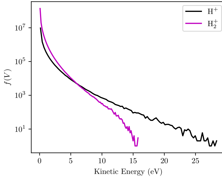
FIGURE 6.6: Ion kinetic energy distribution at the time of 1.1375 ms.
