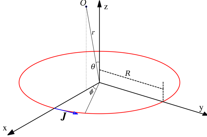
FIGURE 3.8: Current loop setting in spherical coordinate system.
