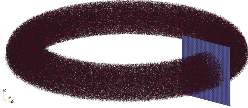
FIGURE 3.10: Extent of the 2D poloidal plane grid.
