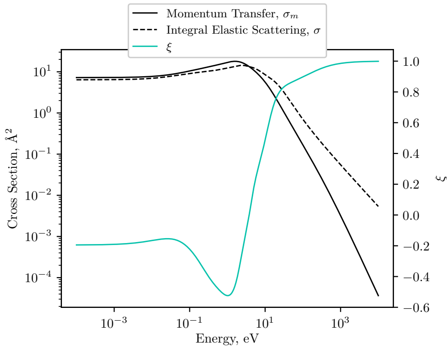
FIGURE 3.6: Cross section values of electron-H 2 molecule collision and the resulting \xi(\epsilon) plotted over electron energy of 0.0001 - 10 000 eV.
