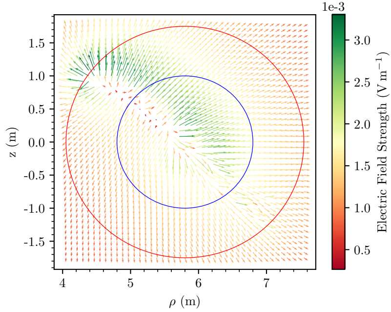
FIGURE 6.17: \mathbf{E}_{\text{int.}} due to charge imbalance between electrons and ions.
