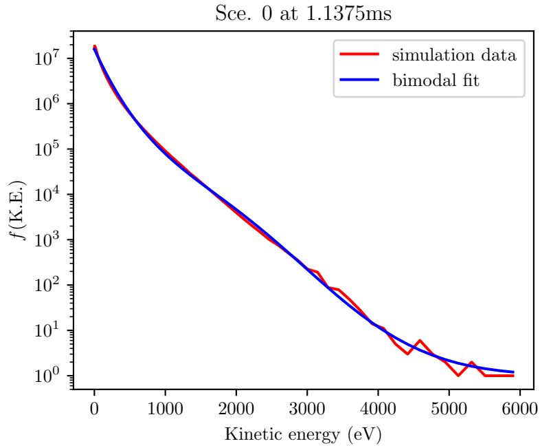
FIGURE 7.6: Electron V_{\text{par}} distribution in kinetic energy scale for Sce. 0 at 1.1375 ms, a bimodal distribution function is fitted to the simulation data.
