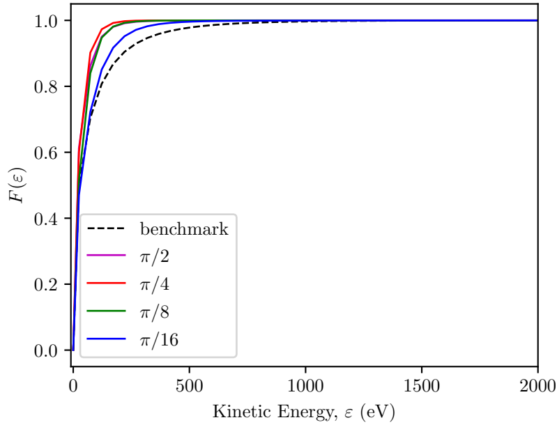
FIGURE 4.19: Cumulative distribution functions of the aforementioned comparisons.
