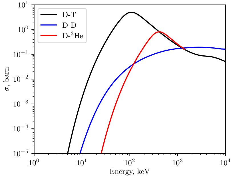
FIGURE 2.1: Cross sections of the corresponding fusion reactions [1].
