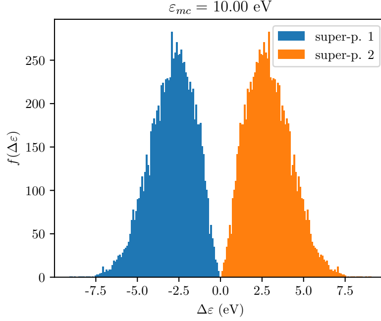
FIGURE 4.8: Histogram of \Delta\varepsilon for super-particle 1 and 2 where N_{\text{rep}} = 10\,000 with \varepsilon_{mc} = 10 eV and S = 4 . The initial merging candidates are initiated with their unit vector distributed in the range of \phi = [0, \pi/2] and \theta = [0, \pi/2] .
