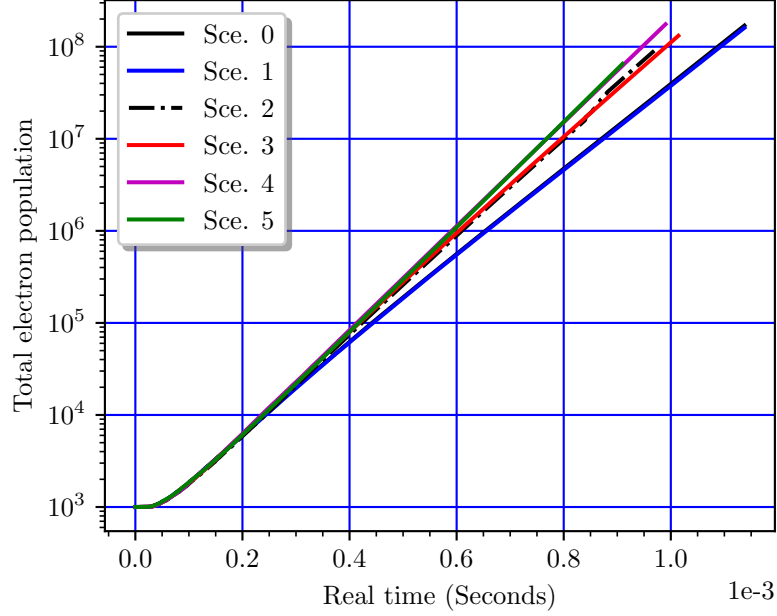
FIGURE 7.7: Total net electrons over time for all considered scenarios.
