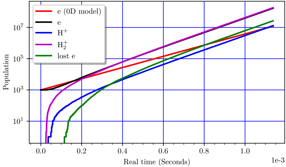
FIGURE 6.13: Population count of electrons, H^+ and H_2^+ ions in time, compared with the electron population growth predicted by Eq. 2.19. The total lost electrons over time is also plotted as well.
