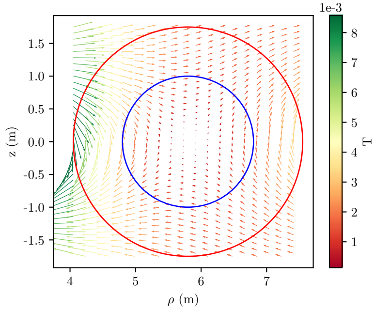
FIGURE 6.4: \mathbf{B}_\theta in the poloidal plane.
