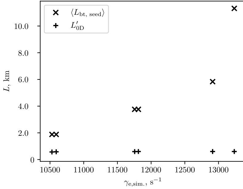
FIGURE 7.9: Comparison between L'_{0\text{D}} and \langle L_{\text{bt, seed}} \rangle for given V_e (Tab. 7.7) and \gamma_{e,\text{sim.}} (Tab. 7.10).
