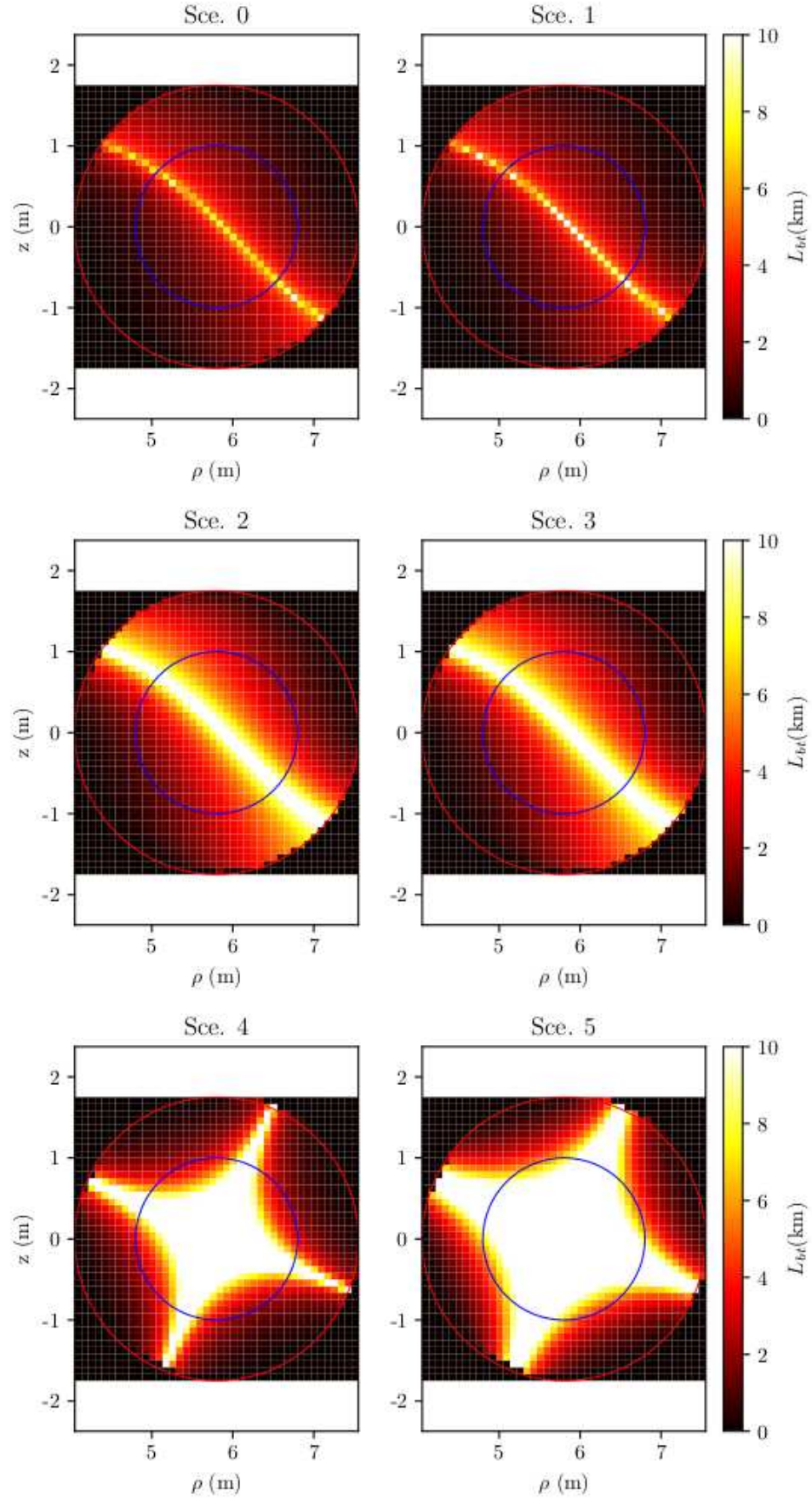
FIGURE 7.2: Map of L_{bt} for all scenarios.
