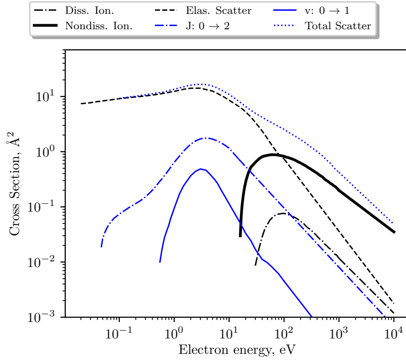
FIGURE 6.9: The extended cross sections.
