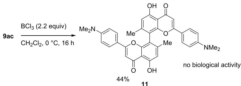
Scheme 5. Selective Deprotection of the Methoxy Groups of Biflavone 9ac for the Synthesis of Biflavone 11 . Yield of Isolated Product
