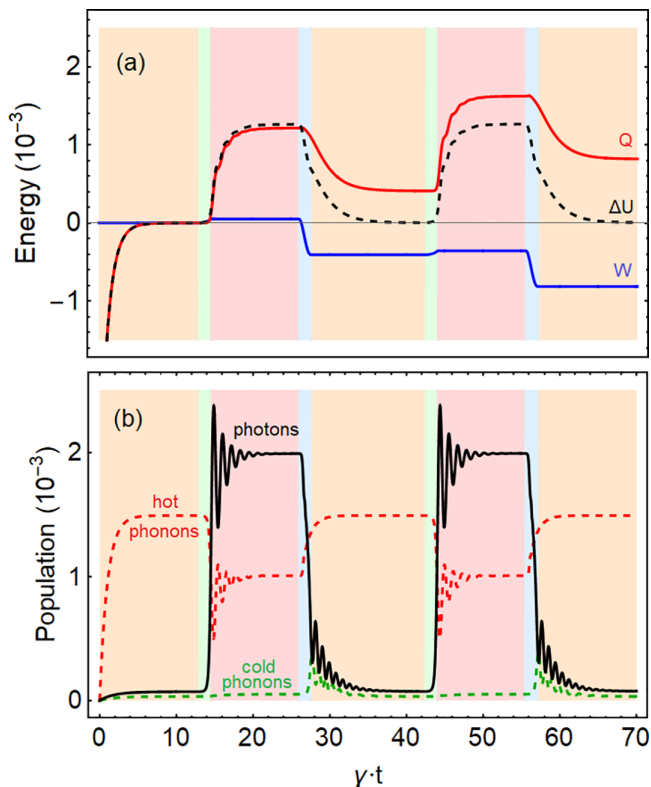
FIG. 3. Time evolution of the quantities of interest. (a) Variation of internal energy \Delta U (dashed, black), the work W (blue), and the heat Q (red). (b) Population of the cavity photon (black), the cold wall 1 phonons (dashed green), and the hot wall 2 phonons (dashed red). The background colors indicate the four strokes shown in Fig. 1: cold isochoric (orange), adiabatic compression (green), hot isochoric (red), and adiabatic expansion (blue). Here \omega_1 = 2 , \omega_2 = 2.6 , \tilde{\omega}_{c,1} = 1.01 , \tilde{\omega}_{c,2} = 1.31 , g_1 = g_2 = 0.05 , T_c = 0.15 , T_h = 0.40 , \gamma_1 = \gamma_2 = \gamma = 0.01 , \kappa = 10^{-6} , and T_0 = 10^{-7} . Frequencies and temperatures are normalized with respect to \omega_{c,1} .
