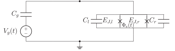
FIG. 11. Illustration of a lumped-element circuit. The right branch contains two linear capacitors with capacitances C_l (left) and C_r (right), two Josephson junctions with Josephson energies E_{J,l} (left) and E_{J,r} (right), and an external flux \Phi_e(t) threading through the loop between the two Josephson junctions. The left branch contains a linear capacitor with capacitance C_g and a voltage source V_g(t) . As it is common practice, we mark the ground node by a dashed triangle.
