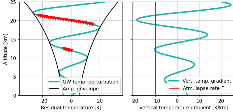
Figure 2.2: Panel a shows the GW amplitude growing exponentially with altitude at a rate of \exp\left(\frac{z}{2H}\right) . Black lines show the envelope, and red triangles show where the GW generates local convective instability. Panel b shows the temperature gradient due to the temperature perturbation of the GW (cyan) and the atmospheric lapse rate for dry air (red). The atmosphere is convectively unstable, where the temperature gradient of the perturbed field drops below the lapse rate.
