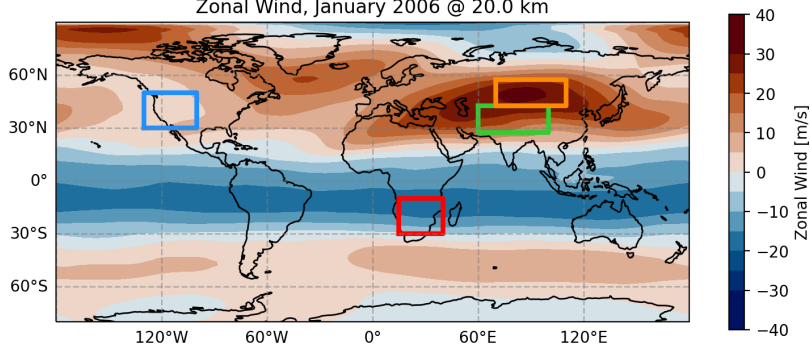
Figure 4.8: Regions of interest for critical layer filtering considered in this study shown on top of the monthly mean zonal wind at 20 km altitude: Himalaya (green), Mongolian Plateau (orange), Rocky Mountains (blue) and southern Africa (red). The same colors as in Fig. 4.7 have been used for the Mongolia and Himalaya regions.
