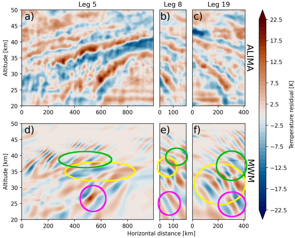
Figure 4.3: Temperature perturbations as measured by ALIMA during flight 12 of the South-TRAC campaign for selected flight legs (panels a – c) and the predictions for the same region from the MWM (panels d – f). The horizontal axis gives the distance from the start point of the flight leg. Information on the corresponding flight paths is given in Fig. 4.4. GW features of special interest for the source allocation are highlighted in the MWM predictions by green, yellow, and magenta ellipses, respectively.
