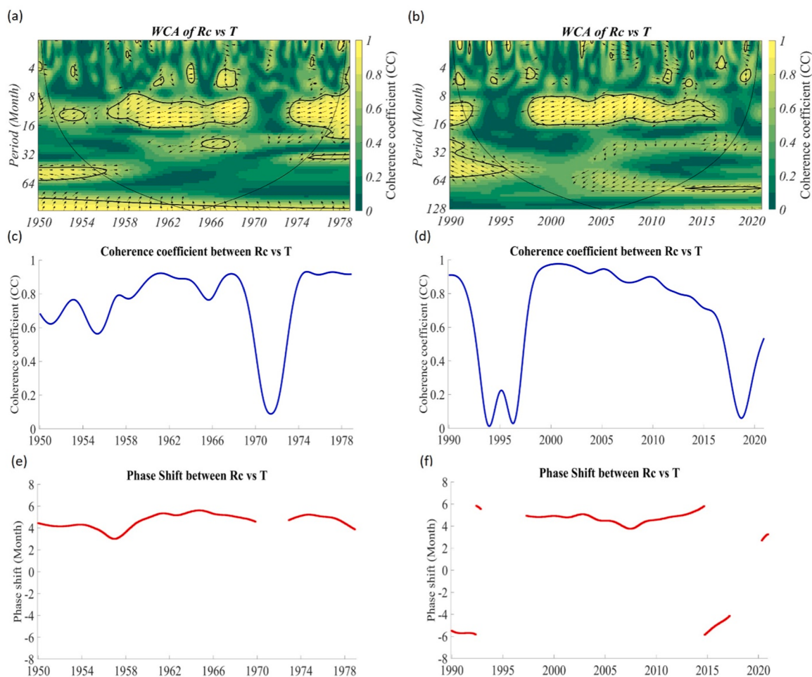
Fig. 5. WCA between R_c and average T in the Upper Tiber at Ponte Nuovo outlet (a)1950–1978 and (b)1990–2020, the 95% significance level is shown as a thick contour. CC between R_c and T during the period of yearly cycle (c)1950–1978 and (d)1990–2020; phase shift between R_c and T in the Upper Tiber at Ponte Nuovo outlet during the period of yearly cycle (e)1950–1978 and (f)1990–2020. Panel (e) and (f) do not include the section where the CC < 0.5 (insignificant).
