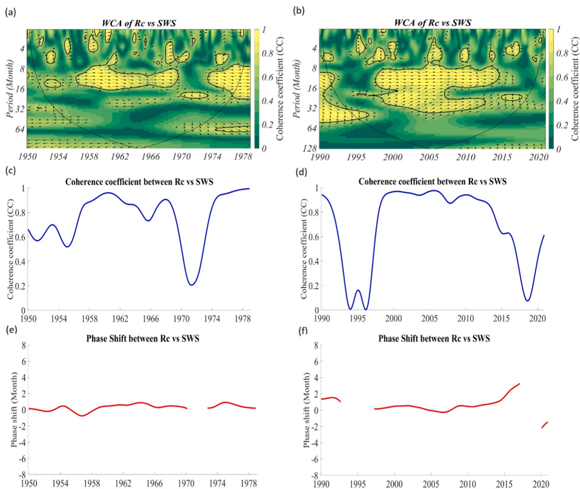
Fig. 4. WCA between Rc and average SWS in the Upper Tiber at Ponte Nuovo outlet during (a)1950–1978 and (b)1990–2020, the 95% significance level is shown as a thick contour. CC between Rc and SWS during the period of yearly cycle (c)1950–1978 and (d)1990–2020; phase shift between Rc and SWS during the period of yearly cycle (e) 1950–1978 and (f) 1990–2020. Panel (e) and (f) do not include the section where the CC < 0.5 (insignificant).
