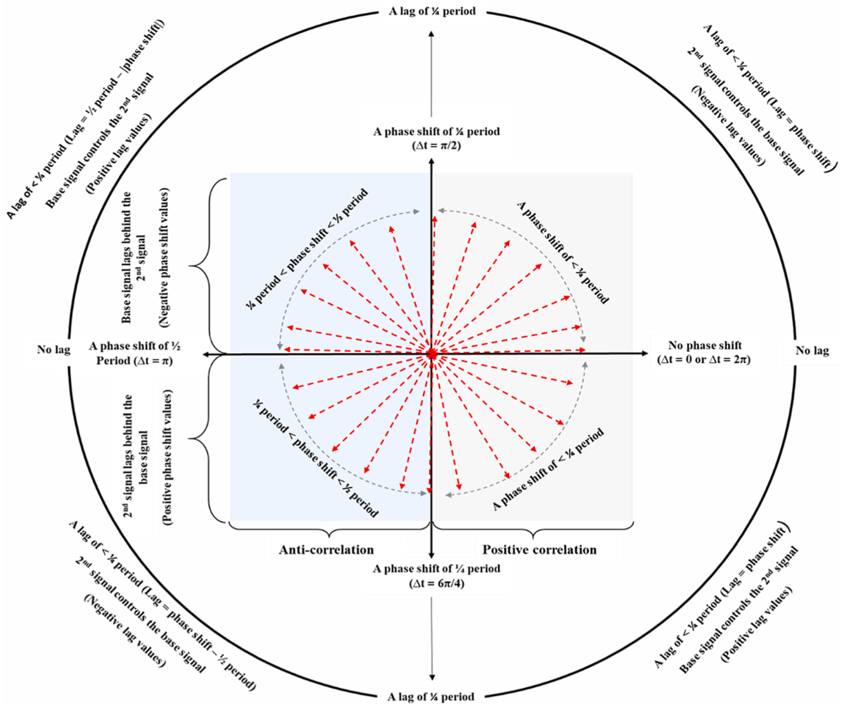
Fig. A. Phase shift, lag, correlations, and arrow directions on wavelet map between base signal and second signal.
