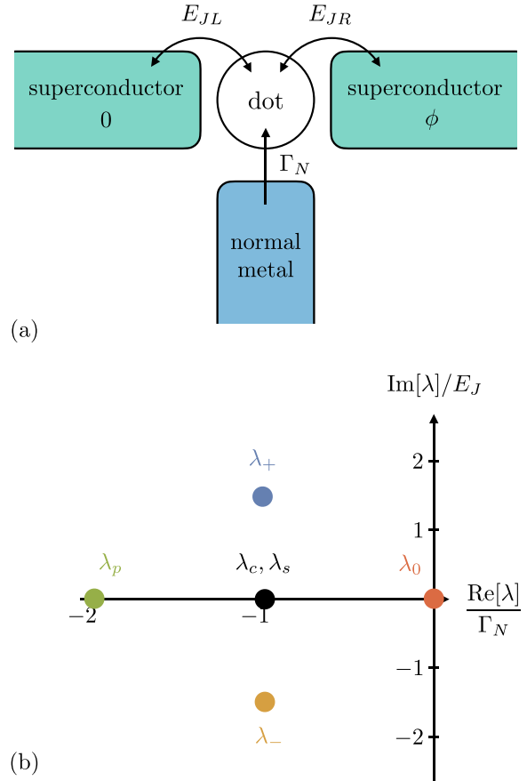
FIG. 2. (a) Sketch of the system under consideration. A central charge island (quantum dot) is connected to a left and right superconductor, with a phase bias \phi . The normal metal pumps quasiparticles into the system with the rate \Gamma_N . A detector with counting field \chi measures current into the right superconductor. (b) The complex eigenspectrum of the quantum master equation \{\lambda\} for \chi = 0 . The eigenmodes can be interpreted as follows. There is a stationary state related to the eigenvalue \lambda_0 = 0 . The nonzero eigenvalues can be associated to the decay of the parity, pseudocharge (see main text), and spin \lambda_{p,\bar{c},s} , respectively, and to the coherent dynamics \lambda_{\pm} .
