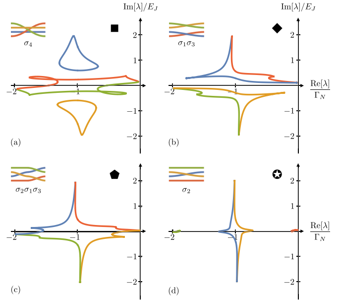
FIG. 8. The real and imaginary parts of the spectrum \lambda_n(\phi) , drawn parametrically for \phi = [0, 2\pi] , for the four different topological phases mapped out in Fig. 7(a)–7(d). In all phases, the 2\pi periodicity in \phi is broken. In (a) and (d), two eigenvalues participate in a braid, either \lambda_0 and \lambda_p in (a), or \lambda_+ and \lambda_- in (d). In (b), both \lambda_0 and \lambda_+ as well as \lambda_p and \lambda_- exchange places during a 2\pi -sweep of \phi . In (c), all eigenvalues interchange, leading to an 8\pi -periodic phase. The phase depicted in (d) has a mapping to a closed system fractional Josephson effect including weak dissipation. The other phases [(a)–(c)] do not have such a correspondence, since they involve the eigenvalues \lambda_0 and \lambda_p (see also main text).
