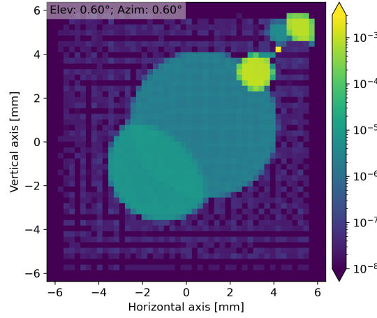
Figure 2. Example of the ghost straylight kernel captured on the detector surface at an elevation of 0.6 degrees and an azimuth of 0.6 degrees.
