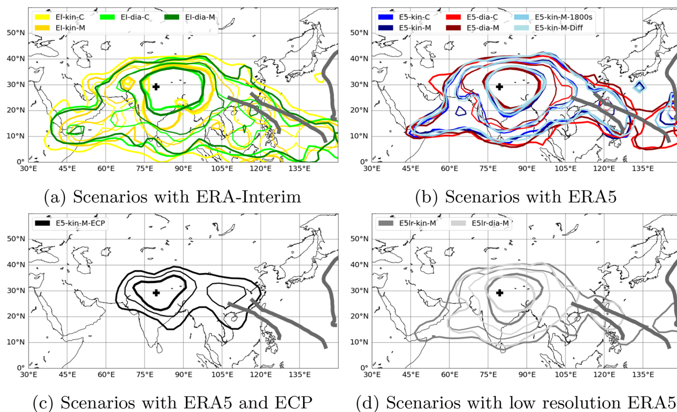
Figure 4. Contours of the probability density function (PDF) of the surface sources for 90 d backward trajectories and all measurements. Colours indicate the different scenarios. For each scenario the inner, thick contour encloses 50 % of the points where air parcels left the MBL and the outer contour encloses 90 % of them. In between, a thin contour is shown for 75 %. For the sake of clarity, the contours are smoothed by a Gaussian kernel. The black cross indicates the position of Nainital. The three thick grey lines show typhoon tracks.
