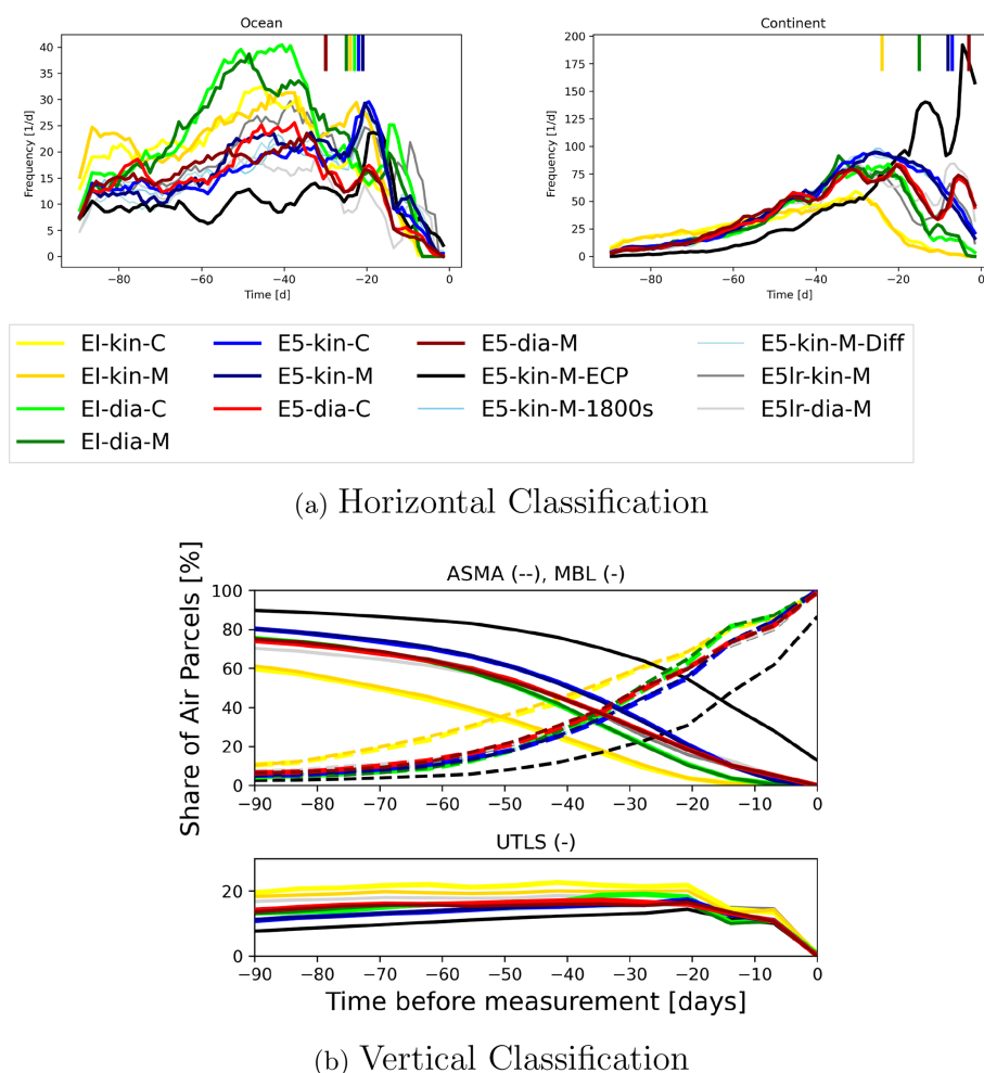
Figure 5. Time evolution of transport from the MBL to the ASMA within 90 d, relative to the start of the trajectories. Panel (a) shows the frequency of air parcels leaving the MBL smoothed with a 1-week running mean. The short lines at the top indicate for some scenarios the maximum time for the first 300 air parcels with the smallest transport time. Panel (b) shows the share of air parcels that are within the ASMA (upper panel, dashed line), the share of air parcels that are in the MBL (upper panel, solid line) and the share of air parcels that are in the UTLS (lower panel, solid line).
