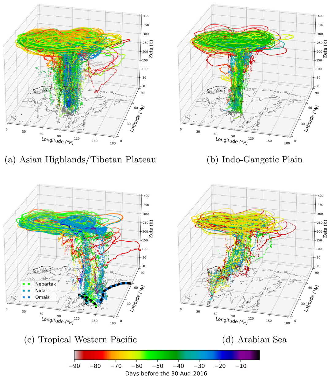
Figure 1. Examples of backward trajectories of air parcels of all of the 15 measurement days from the ATAL measurement to the MBL, categorised by the source region. Shown are trajectories of scenario E5-kin-C. Colours indicate the time when the air parcels left the MBL. Grey dots at the bottom show the horizontal position of the air parcels (APs) 48 h before they crossed the MBL from below. In (c), additionally, tracks of three typhoons are plotted (Nepartak, Nida, Omais), where each point is coloured like the trajectories and the mean time of occurrence.
