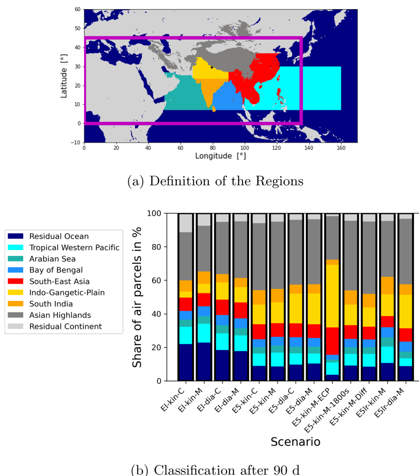
Figure 3. Panel (a) shows the definition of contributing regions. The purple box marks an area that contains most of the air parcels that circulate in the ASMA. Panel (b) shows the horizontal classification of the air parcels according to the surface regions after a 90 d backward trajectory time. Shown is the fraction of air parcels that reach the MBL.
