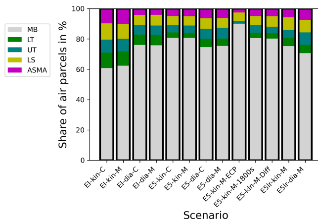
Figure 2. Vertical classification of air parcel origin after 90 d of backward trajectory calculations with different scenarios.
