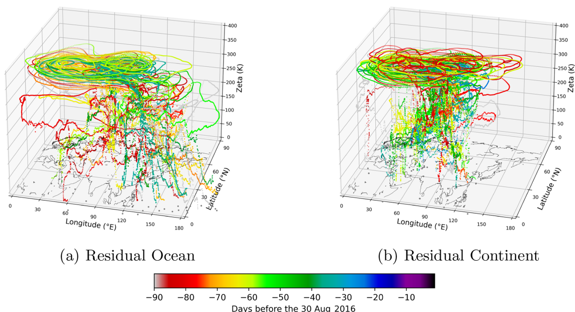
Figure B2. Exemplary backward trajectories of air parcels of all of the 15 measurement days from the ATAL measurement to the MBL, categorised by the source region. Colours indicate the time when the air parcels leaves the MBL. Grey dots at the bottom show the horizontal position of the APs 48 h before they cross the MBL from below.
