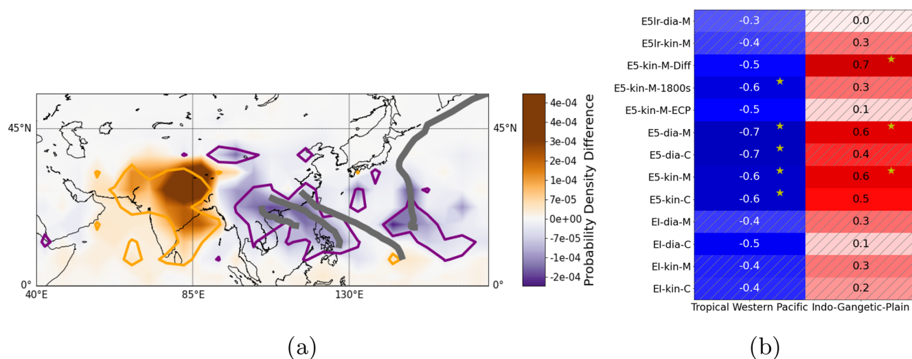
Figure 7. (a) Difference between the source region PDF of the 5 d with maximum ATAL backscatter intensity and 5 d with minimum backscatter intensity, derived from the multi-scenario mean. The orange contours show areas where at least two-thirds of the scenarios indicate high values during a strong ATAL. The purple contours show the same for the weak ATAL cases. Data are given on a 5^\circ grid. The grey lines indicate the tracks of tropical storms that influenced the measurements. (b) Spearman correlation coefficient for the relation between the daily BSR and the contributions of different regions for different scenarios. Hatched areas indicate insignificant results ( p value higher 0.10). Boxes with yellow stars indicate p values lower than 0.05. Colours emphasise positive (red) and negative (blue) correlations.
