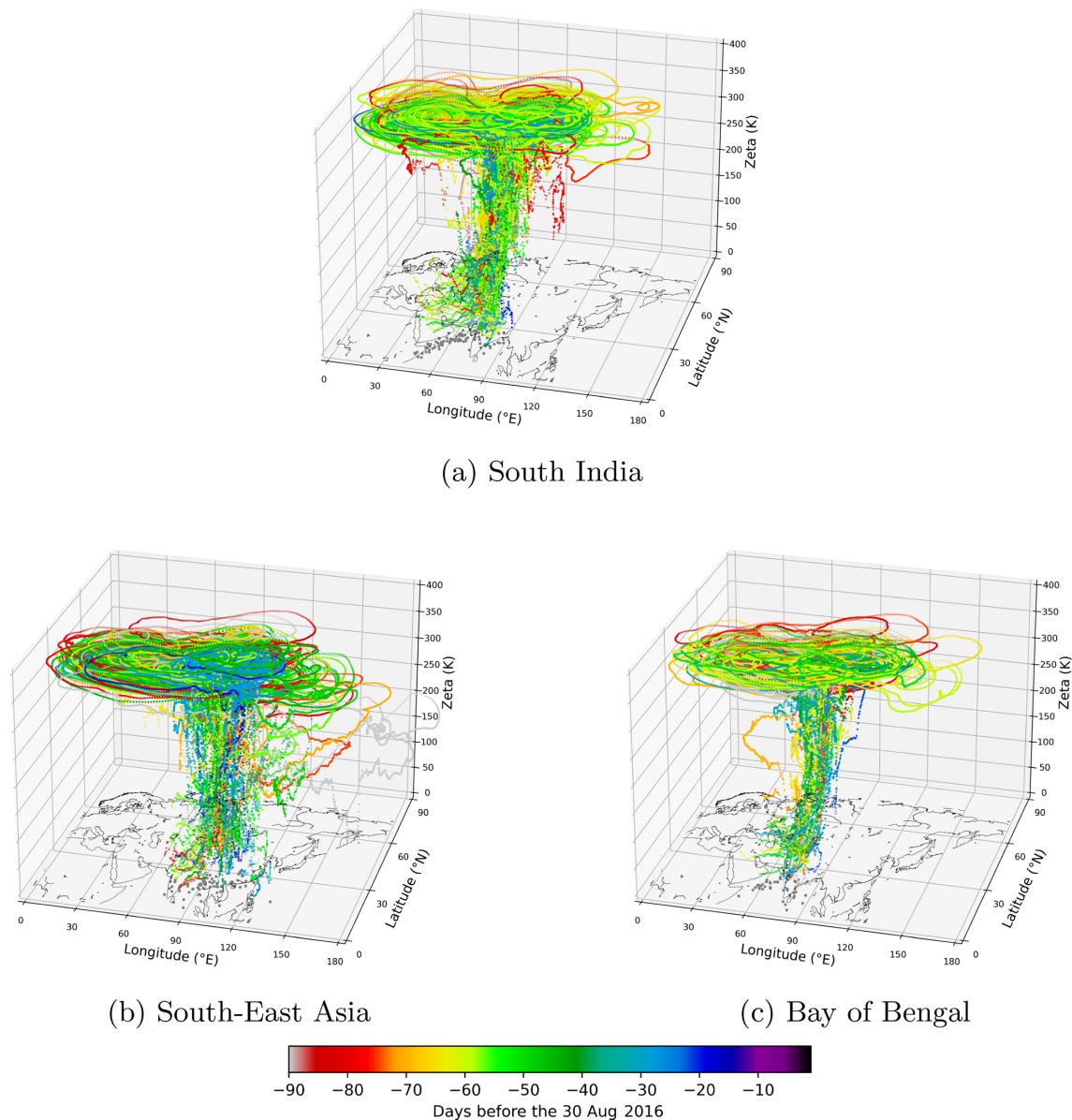
Figure B1. Exemplary backward trajectories of air parcels of all of the 15 measurement days from the ATAL measurement to the MBL, categorised by the source region. Colours are chosen as in Fig. 1.
