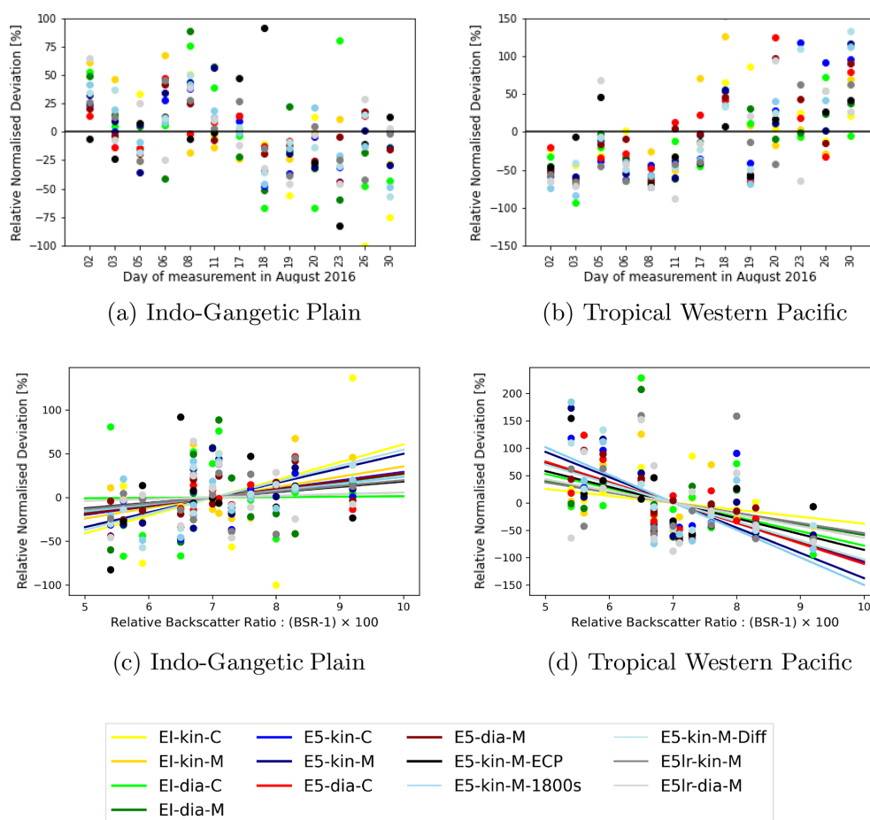
Figure 6. Panels (a) and (b) show the relative, normalised deviation for each measurement day of the Indo-Gangetic Plain and the tropical western Pacific. Panels (c) and (d) show the relations between the daily averaged backscatter intensity and the relative, normalised deviation. The lines show linear fits for each scenario. Coloured dots show results for all scenarios. The colour code for the dots is the same as in Fig. 5, where every colour corresponds to one scenario.
