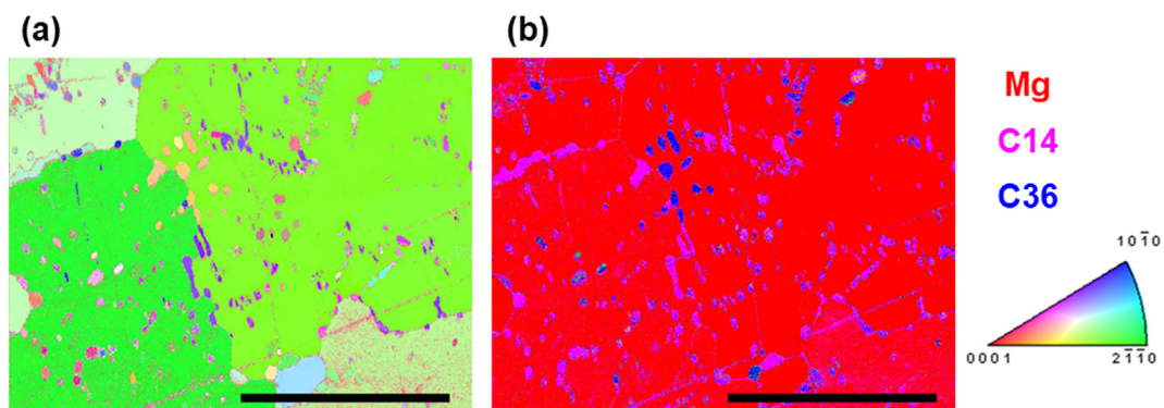
Fig. 6. (a) EBSD-inverse pole figure map and (b) phase map of Mg, C14 and C36 phases superimposed on each other for Mg-4Al-4Ca ht. Scale bars are 100 μm.
