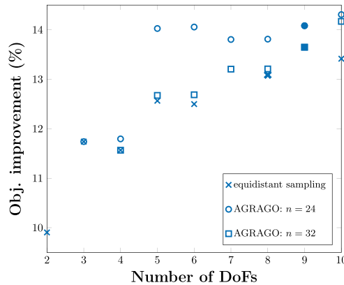
Fig. 8 Economic objective value improvement compared to non-scheduling operation with the number of DoFs for different methods and highest grid resolution of refinement. Crosses ( \times ): Solution of problem (2a)–(2d) using equidistant grid sampling for different numbers of control intervals n . Circles ( \circ ): Solution of problem (3a)–(3e) for n = 24 , q = 3 and different numbers of control set-point intervals. Squares ( \square ): Solution of problem (3a)–(3e) for n = 32 , q = 1 and different numbers of control intervals. The points with filled marks correspond to AGRAGO's suggestion and the point with the bold cross mark correspond to the solution of equidistant sampling
