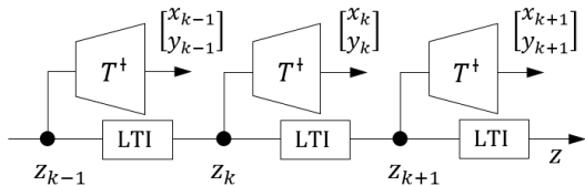
Figure 2: Graph structure of Koopman model prediction.
