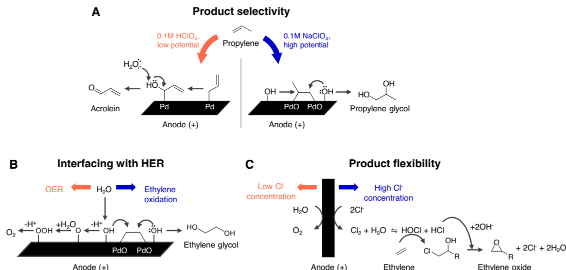
Fig. 4 | Technical targets that must be achieved for anodic hydrocarbon oxidations and reported strategies to overcome them. A Funnelling selectivity towards the desired product (adapted from ref. 24, copyright 2019 Royal Society of Chemistry). B The interfacing of anodic partial hydrocarbon oxidation with
