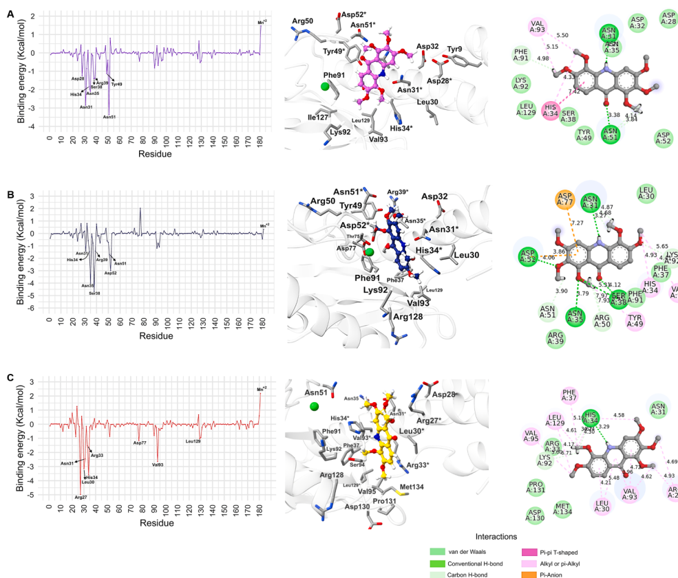
Fig. 7. MD of complexes that presented the best Vina score values. The figure is organized by row: Per-residue decomposition analysis from MM/PBSA calculation; the best \Delta G_{\text{binding}} binding mode and 2D interactions between ligand and protein residues. Ligand binding mode that presents the lower \Delta G_{\text{binding}} residues less than 5 Å away from the FAC21 (in gray stick): (A) replica 1, (B) replica 2, and (C) replica 3. Residues are numbered according to the protein sequence, and \text{Mn}^{2+} is 181. The residues marked with * in the middle panel appeared with \Delta G_{\text{binding}} lower than −1 kcal/mol in per-residue MM/PBSA analysis. The \text{Mn}^{2+} is represented by a green ball in the middle panel figures.
