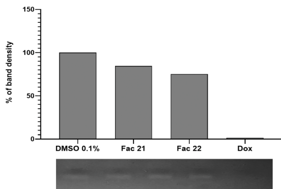
Fig. 4. Interaction of FAC21 and FAC22 with viral dsRNA. Thirty nanomoles of JFH-1 HCV dsRNA were incubated with FAC21 and 22 at 18.5 \mu M or the controls (DMSO 0.1 % and doxorubicin at 100 \mu M) for 45 min at room temperature. The reaction products were subjected to 1 % agarose 1X TAE electrophoresis gel containing Ethidium Bromide, followed by densitometry analysis on ImageJ.JS version 1.53j.
