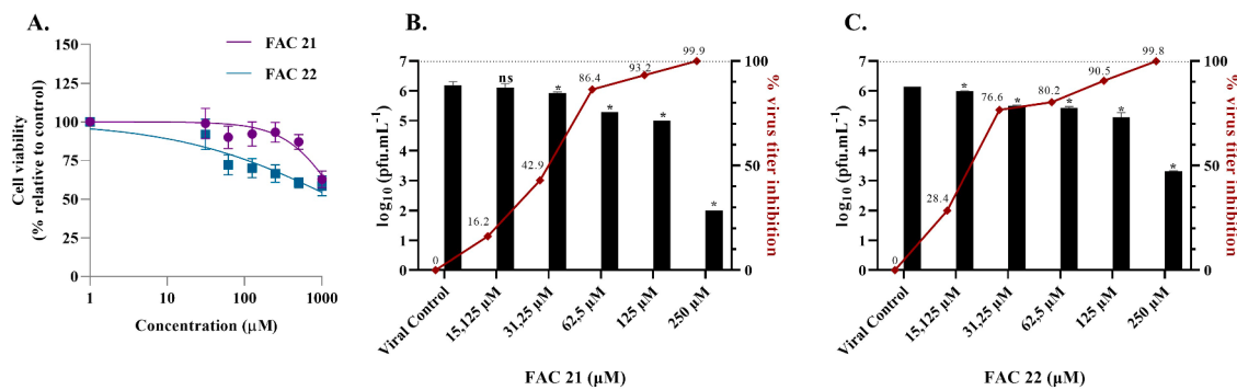
Fig. 2. Acridones have low cytotoxicity, and their effect on viral yield is concentration-dependent. (A) Cytotoxicity assay of the tested compounds in Vero cells. The cytotoxicity of acridones based on the dose-response was determined using MTT. The 50 % cytotoxic concentration (CC 50 ) was calculated for each compound using nonlinear regression analysis of GraphPad Prism software (version 8.0.1). (B/C) OROV production was measured in the presence of several dilutions of the tested compound in Vero cells, with an initial inoculum of MOI 0.1 under simultaneous treatment (bars chart and left axis). The diamond shape (◆) and the right axis represents percentages of viral inhibition under viral control. Error bars represent standard deviations. Values are the mean ± standard error obtained from three independent experiments. The dashed line indicates the detection limit for the viral titers assay. Asterisks indicate statistical significance between the control and each group as determined by two-way ANOVA and subsequent Dunnett's test (*, p < 0.05 ).
