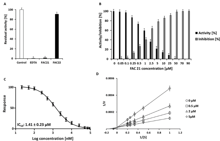
Fig. 5. Inhibition test, \text{IC}_{50} value determination and inhibition mode of the acridones FAC21 and FAC22 against OROV endonuclease. The enzyme activity was determined using the FAM-TCT CTA GCA GTG GCG CC-TAM DNA substrate, and the fluorescence intensities after cleavage were measured at 495 nm (excitation) and 520 nm (emission). (A) Primary inhibition test of FAC21 and FAC22 (50 \mu\text{M} ) against the OROV endonuclease activity. EDTA (50 \mu\text{M} ) was used as a known inhibitor control. (B) Normalized activity and inhibition of the endonuclease protein under the effect of FAC21. FAC21 was tested using a concentration range of 0–90 \mu\text{M} . (C) Dose–response curve for the \text{IC}_{50} value of FAC21 was determined by nonlinear regression. The normalized response [%] of OROV Endonuclease is plotted against the Log of the FAC21 concentration. The determined \text{IC}_{50} value is presented insert. (D) Inhibition mode of FAC21. The experiment was performed using different final concentrations of the inhibitor (0, 0.5, 2 and 5 \mu\text{M} ) and titration of the substrate. The data were analyzed using a Lineweaver-Burk plot; therefore, the reciprocal of velocity ( 1/V ) vs the reciprocal of the substrate concentration ( 1/[S] ) was compared. Data shown are the mean \pm standard deviation (SD) from three independent measurements ( n = 3 ).
