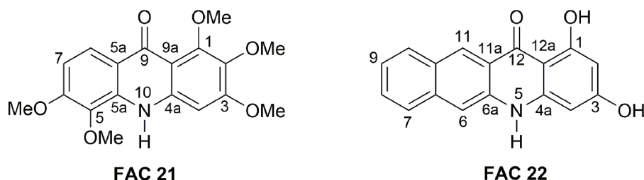
Fig. 1. Chemical structure of the acridones FAC21 and FAC22.
