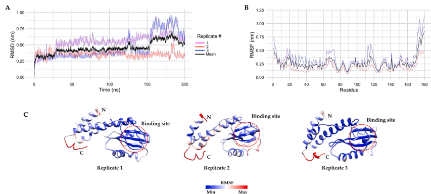
Fig. 6. MD simulations analysis of the N-terminal Endonuclease of OROV. (A) C \alpha RMSD evolution by 200 ns trajectory of three replicates (1 - purple, 2 - red, 3 - blue) and mean (black line). (B) RMSF analysis of three replicates using the same color scheme used in (A). It shows the average fluctuation per residue along the MD trajectory. (C) Ribbon representation of the three replicates coloured according to the RMSF values (with low and high fluctuation in blue and red, respectively). The \text{Mn}^{2+} binding site is shown in a red circle.
