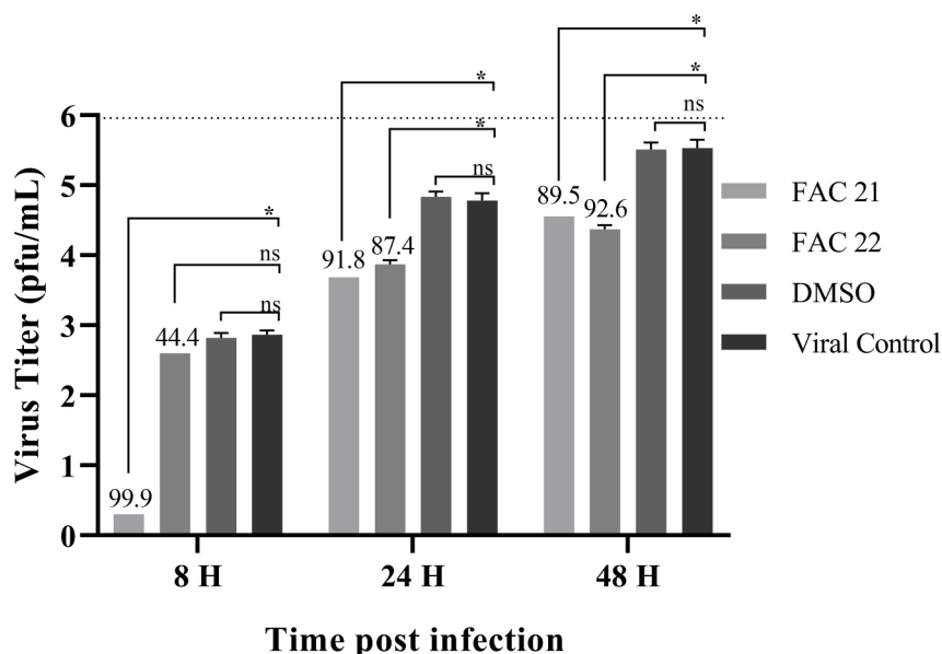
Fig. 3. Antiviral activity of acridones in Oropouche Virus Progeny. Culture supernatants were harvested at the indicated time points. OROV production was measured in the presence of 125 μM dilution of the FAC21 or FAC22 in cells infected with MOI 0.1 by plaque forming assay. DMSO represents diluent control. Values are the mean ± standard error obtained from three independent experiments. The numbers above the bars indicate the percentage of virus inhibition (under the viral control). The dashed line indicates the detection limit for the viral titers assay. Asterisks indicate statistical significance between the control and each group as determined by two-way ANOVA and subsequent Dunnett's test (*, p < 0.05 ).
