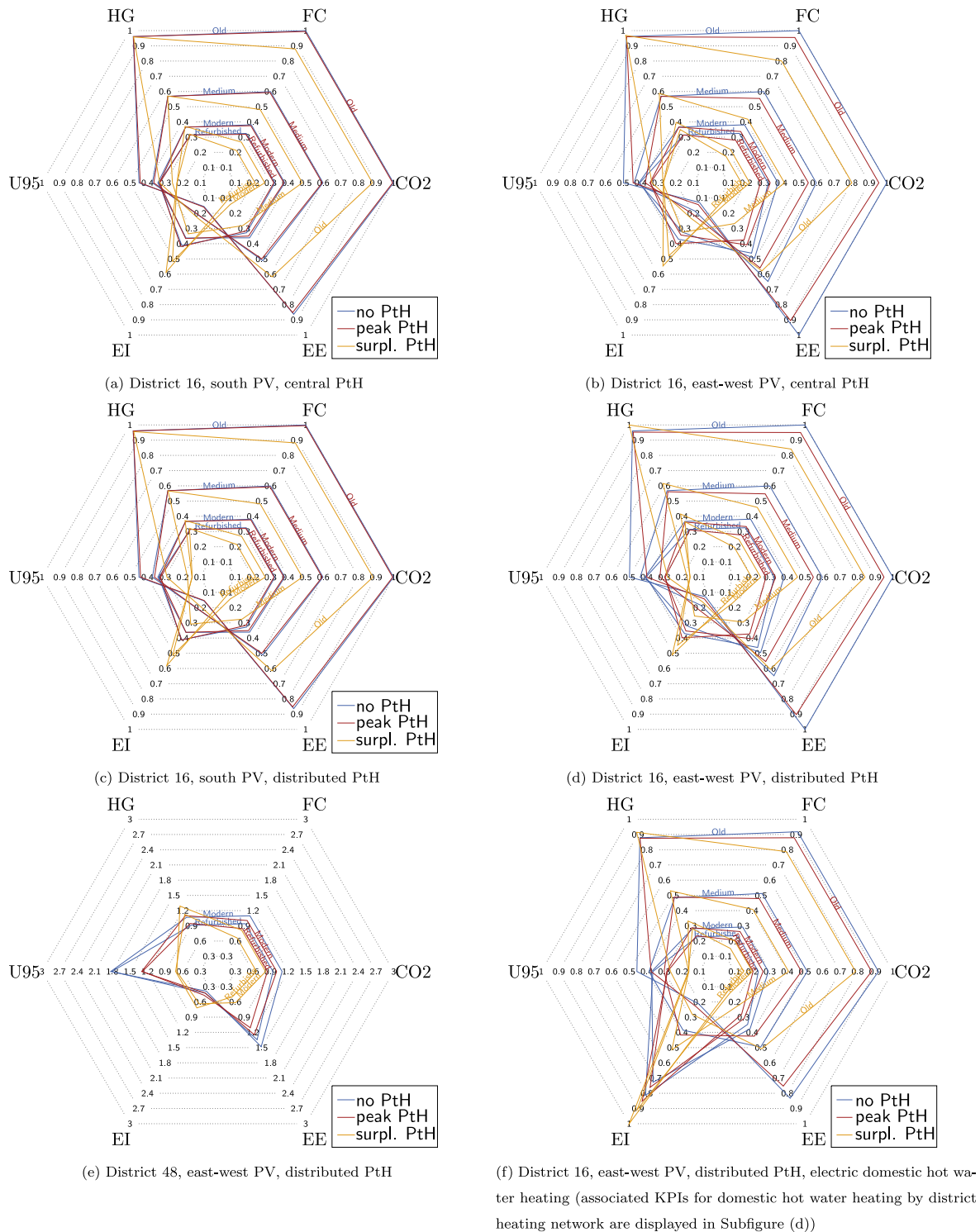
Fig. 11. Key performance indicators CO 2 emissions (CO 2 ), fuel consumption (FC), heat generation (HG), electrical energy import (EI), electrical energy export (EE), line end voltage (U95) from Table 4 for selected configurations. The values are normalized to the associated maximum occurring value.
