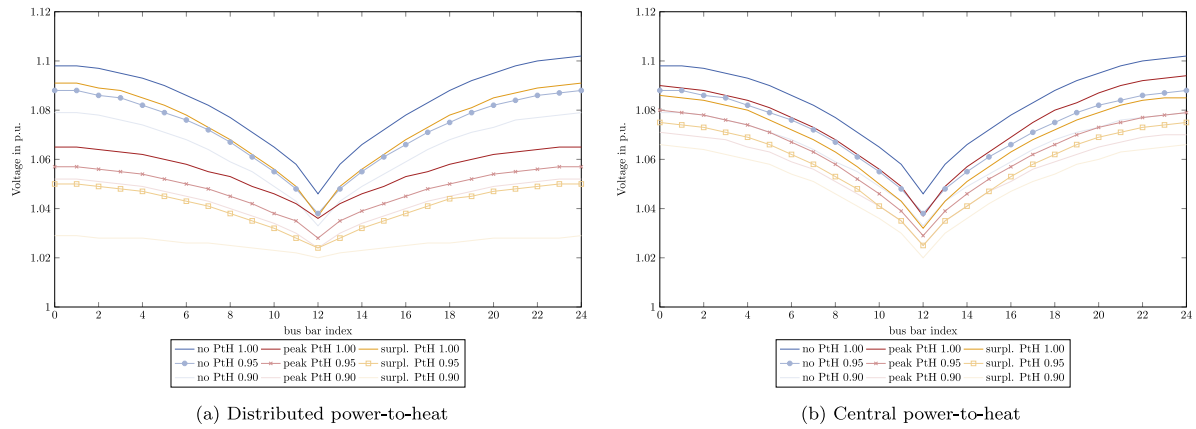
Fig. 7. Voltage distributions for District 48, Refurbished buildings, and East-west PV between May 28th, 2020 and June 3rd, 2020 based on 10 min average. Each line displays the voltages that are not exceeded in the associated share of time. The power-to-heat operation modes peak shaving and surplus yield a significant voltage reduction for distributed power-to-heat (Subfigure (a)). Supplementary Figure 3 depicts the voltage distributions in 0.01 granularity.
