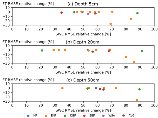
Figure 12. Comparison of the SWC and ET characterization for the OL and DASP simulations. Each point represents the overall average RMSE change for one site. The color of the points indicates the classification code for the different forest types (MF – mixed forest, ENF – evergreen needle leaf forest, DBF – deciduous broad leaf forest, EBF – evergreen broad leaf forest, AVG – average over all forest types).
