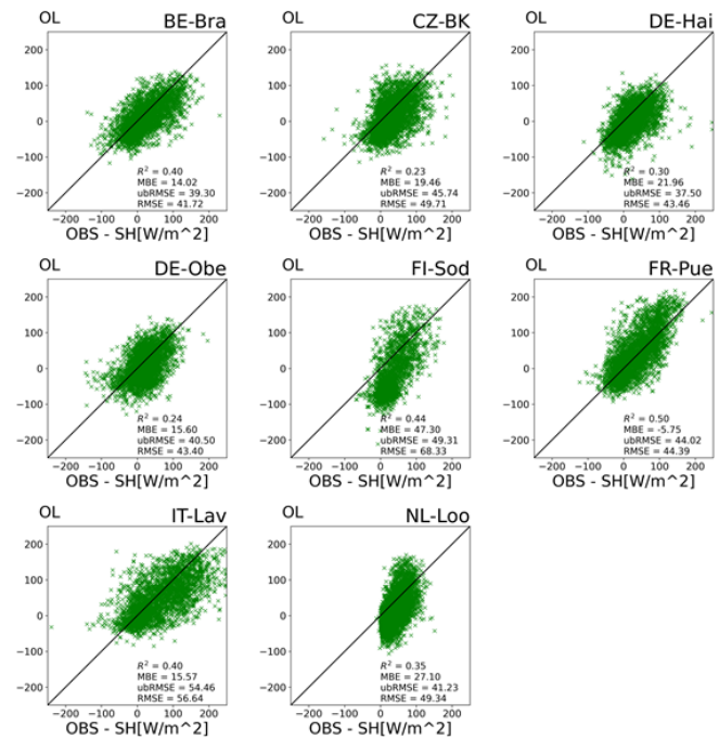
Figure 14. Scatter plots of observed sensible heat flux at eight study sites versus OL simulation results. The points represent daily averages for the days on which observation data are available.
