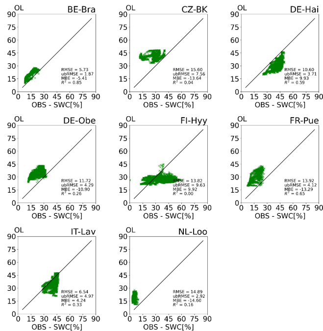
Figure A6. Scatter plots of observed soil water content at eight study sites versus OL simulation results at 50 cm depth. The points represent daily averages for the days on which observation data are available.
