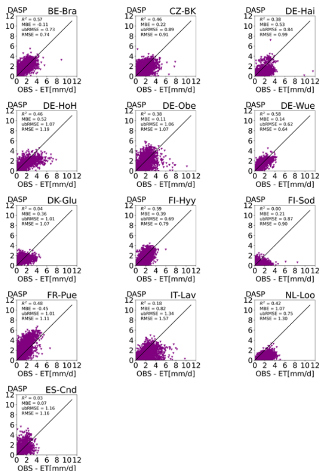
Figure 11. Scatter plots of observed evapotranspiration at 13 study sites versus DASP simulation results. The points represent daily averages for the days on which observation data are available.
