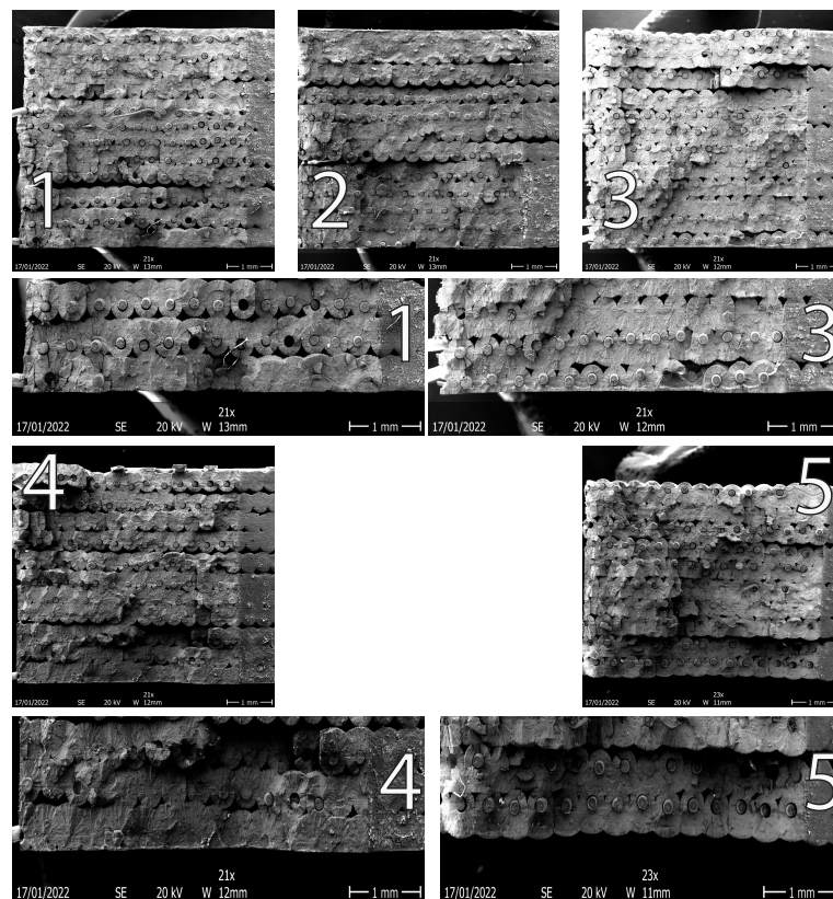
Figure 14. Pictures of the fracture surface of the individual medium-sized samples (numbers indicated sample name), the closeups highlight the good ductile failure of the fibres in some cases and the brittle nature in others.
