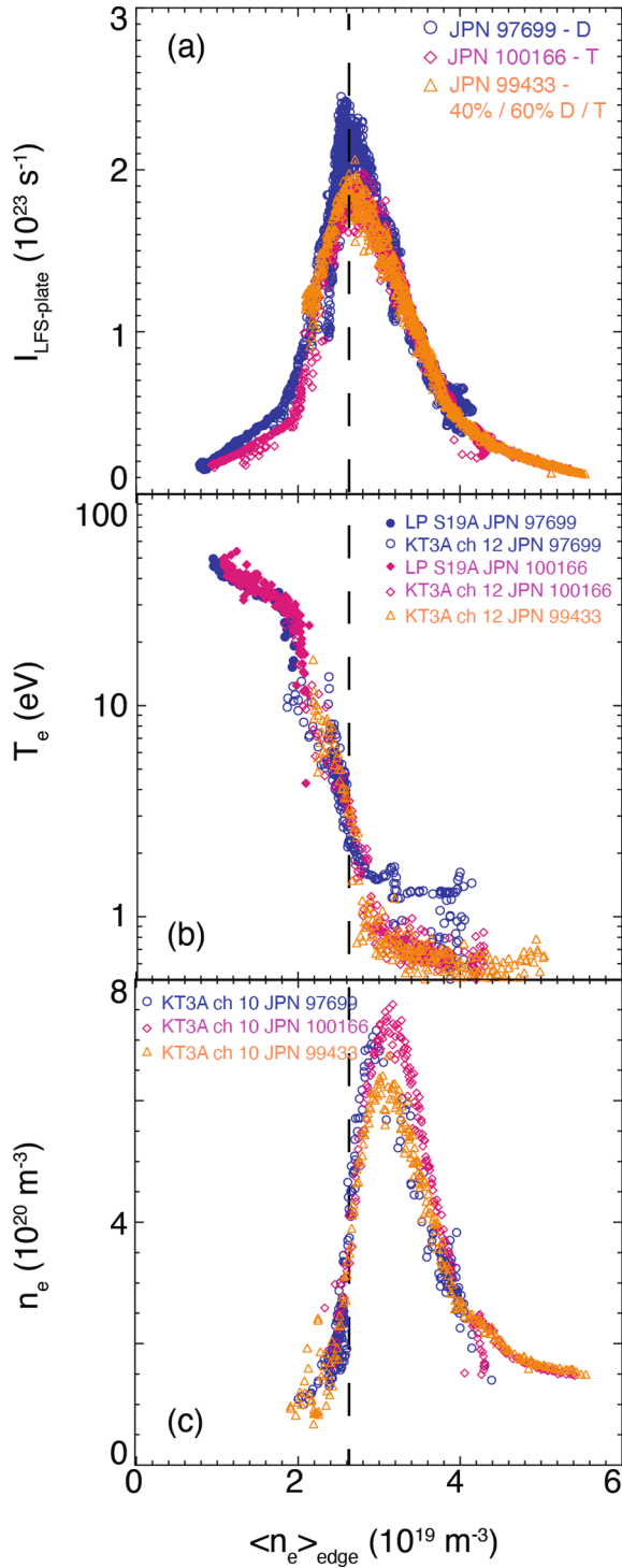
Fig. 3. Total ion current to the LFS target plate (a), electron temperature (b) and electron density (c) as a function of line-averaged density at the outer edge of the core plasma in unpumped plasmas. Deuterium plasmas are shown in blue (JPN 97699), tritium in magenta (JPN 100166) and deuterium–tritium in gold (JPN 99433). T_e (b) was measured with Langmuir probes (circles, probe S19A) and inferred spectroscopically (KT3A, squares, channel 12), while n_e was inferred spectroscopically only (KT3A, squares, channel 10). The black dashed vertical line indicates the assumed detachment onset density based on the saturation of I_{\text{div,LFS-plate}} . (For interpretation of the references to colour in this figure legend, the reader is referred to the web version of this article.)
