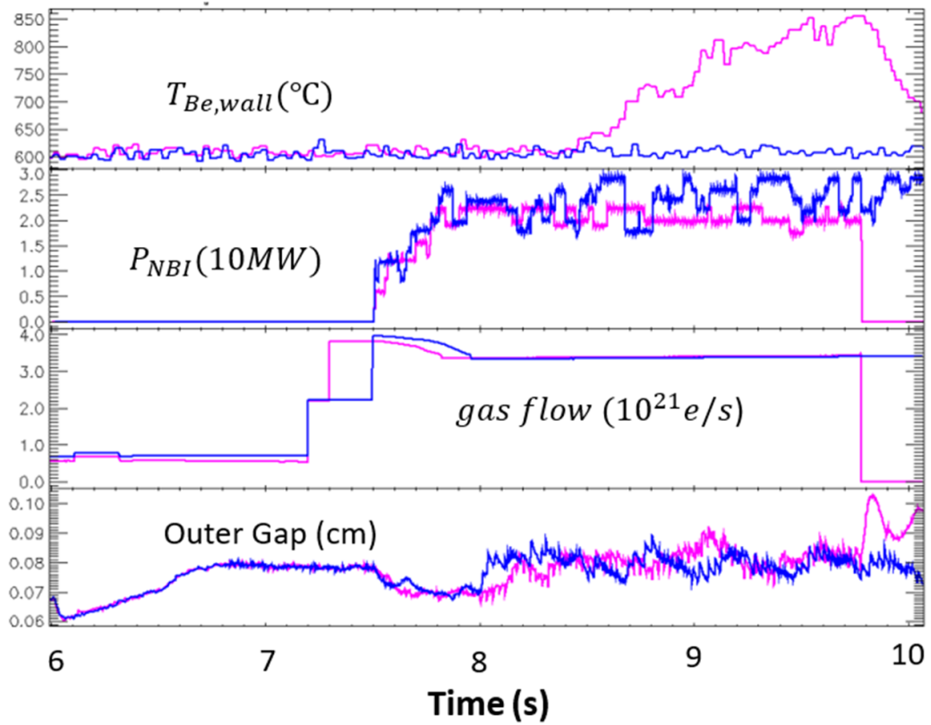
Figure 6. Time traces of JET T pulse #98901 (magenta) and its D reference #97886 (blue): beryllium wall surface temperature ( T_{\text{Be,wall}} ) next to the NBI duct, NBI total heating power ( P_{\text{NBI}} ), injecting gas flow and radial outer gap.
