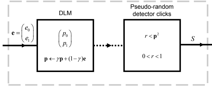
Fig. 4. Diagram of the event-based detector model defined by Eqs. (7) and (8). The dashed line indicates the data flow within the processing unit.
