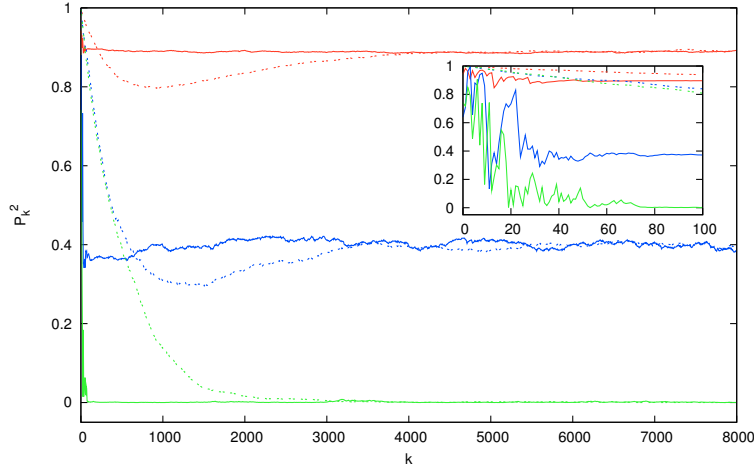
Fig. 9. (color online) The square of the length of the internal vector \mathbf{p}_k^2 as a function of the number of received events k for three different input messages \mathbf{e}_k = (r_k^{1/2}, (1 - r_k)^{1/2}) (top lines), \mathbf{e}_k = (\cos \pi r_k, \sin \pi r_k) (middle lines), and \mathbf{e}_k = (\cos 2\pi r_k, \sin 2\pi r_k) (bottom lines) where the 0 \leq r_k < 1 are uniform pseudo-random numbers. Dashed lines: Model Eq. (7). Solid lines: Model Eq. (22) with \kappa = 0.9 . The inset shows the short-time response of models Eq. (7) and Eq. (22) in more detail. In all cases \mathbf{p}_0 = (1, 0) , w_0 = 0.9 and \gamma = 0.999 .
