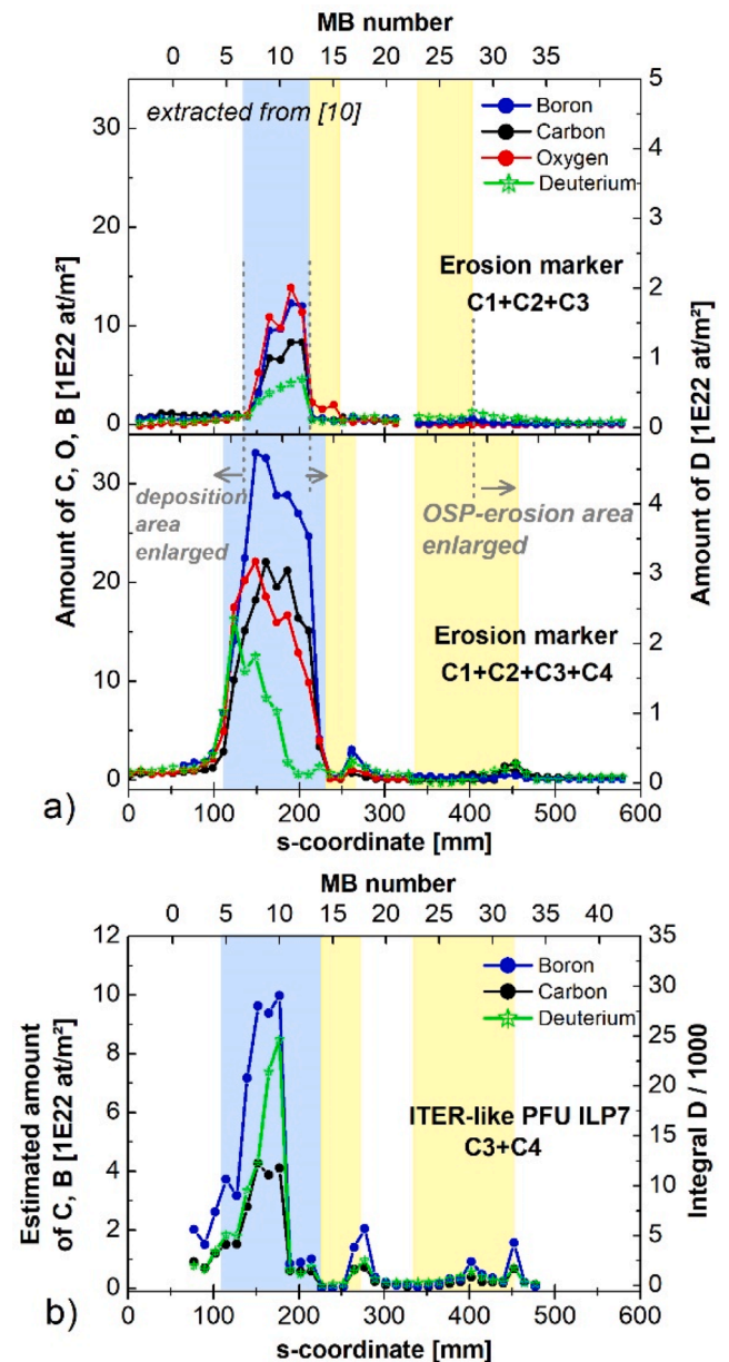
Fig. 9. (a) RBS/NRA analysis showing the amount of B, C, O and D along the post-C3 and post-C4 erosion marker tiles, highlighting changes in the erosion/redeposition pattern between C3 and C4. The data are extracted from [10]. (b) The same analysis was performed on ILP7 exposed to C3 and C4, except that the data were evaluated in the thin-layer limit (increased error for thick deposits). A scaling factor of 8.9 was applied between the y-axis of B and C to take the difference in cross-section into account.
