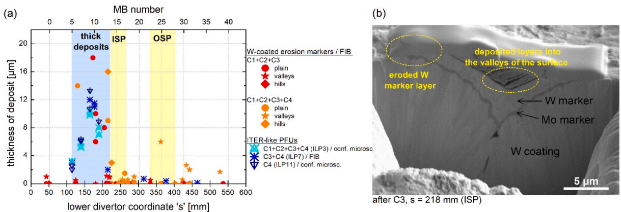
Fig. 7. (a) thickness of redeposited layers along the radial s -coordinate of the divertor targets. The data were obtained on the central line of post-C3, post-C4 erosion marker tiles and ILP7 using SEM/FIB. Confocal microscopy was also used on ILP3 and ILP11 after the deposits were removed by adhesive tape. (b) SEM/FIB image of post-C3 erosion marker tile showing the competition between erosion and redeposition in areas close to the SP due to the roughness of the tiles.
