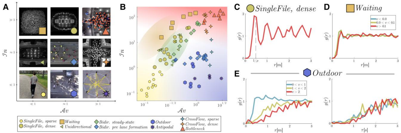
Fig. 1. Delineation of crowd flow regimes with the dimensionless numbers \ln and Av . A) Sketch of the expected diagram, illustrated with snapshots from the collated datasets (described in SI Appendix A). B) Empirical diagram obtained from various pedestrian datasets. Each datapoint corresponds to one experimental run or observational sequence. The experimental data from SingleFile and CrossFlow were split into a sparse and a dense dataset. Colored gradients are visual guides, to indicate different regimes. C) Pair-distribution function (pdf) for one run of the SingleFile, dense dataset. D) Pdf for the Waiting dataset and E) for the Outdoor dataset. The curves are binned according to the rate of approach v = -dr/dt (given in m/s). As for D) the pdf is well parameterized by r and poorly by \tau (see Fig. S3) and in E) vice versa.
