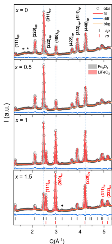
Figure 2. XRD data and Rietveld refinements of particles at different degrees of lithiation. The two main structures, \text{Fe}_3\text{O}_4 (inverse spinel, denoted as sp) and \text{LiFeO}_2 (rock-salt, denoted as rs), are indicated at each degree of lithiation ( 0 \leq x \leq 1.5 ). The black symbols correspond to observed data points, the red curve to the Rietveld fit, and the blue line to the difference between the experimental data and the fit. The bars at the bottom indicate the peak positions for both phases. The stars indicate the position of the superstructure reflections of the maghemite phase. An additional peak at ca. 3.2 \text{ \AA}^{-1} (black dot) can be related to metallic iron. The diffraction ( hkl ) planes of each phase are shown above the peaks.
